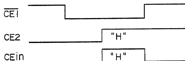
FIG. 3 (PRIOR ART)
