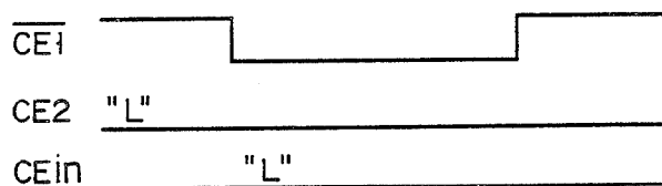
FIG. 2 (PRIOR ART)
