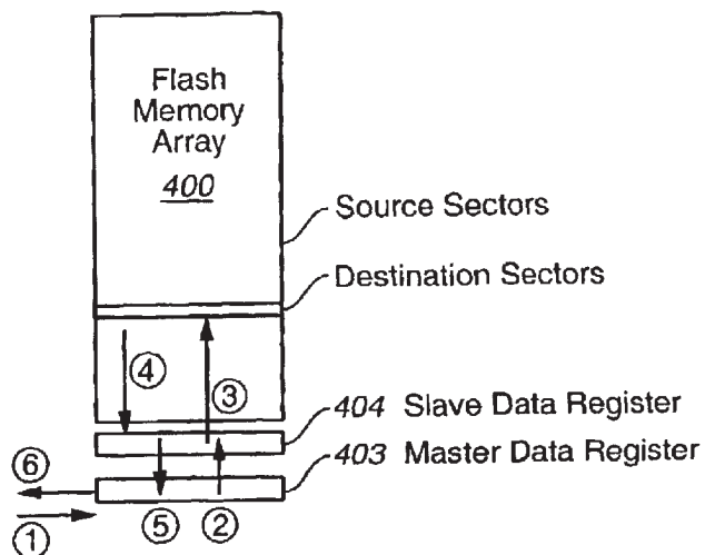
FIG. 4 (PRIOR ART)
