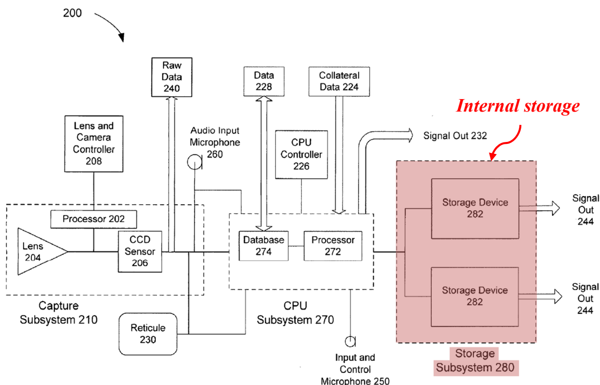
Spatharis, Fig. 2 (annotated)
