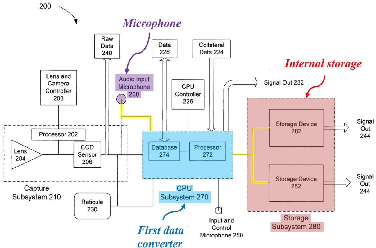
Spatharis, Fig. 2 (annotated)
