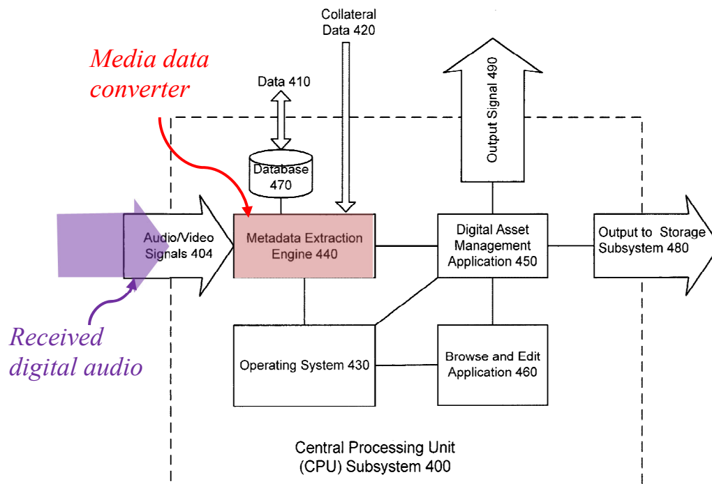
FIG. 4 Spatharis, Fig. 4 (annotated)
