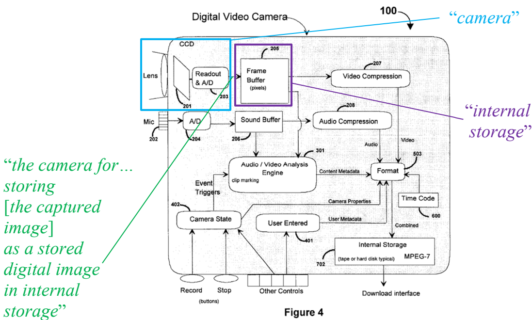
Fuller, FIG. 4 (annotated)
