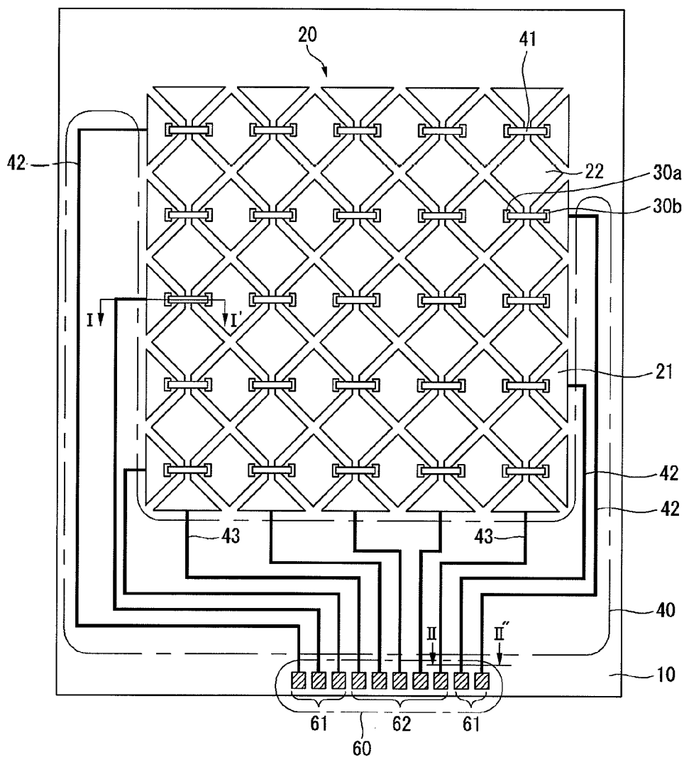
FIG. 1 RELATED ART
