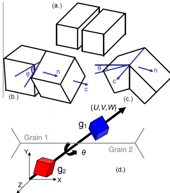
Fig. 11. (a) Schematic of two adjacent lattices, where the interface is known as a grain boundary, (b) a twist GB as the axis of rotation corresponds to the normal plane of the GB, (c) a tilt GB as the axis of rotation is perpendicular to the GB normal, and (d) schematic of the axis-angle pair for grain boundary description.
