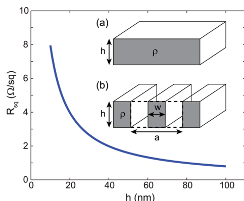
FIGURE 1. Electrical sheet resistance of a metallic film electrode as a function of film thickness. (a) The sheet resistance R_{sq} = \rho/h of a homogeneous film depends on the resistivity of the metal \rho and physical thickness of the film h . (b) The sheet resistance for a nanopatterned film R_{sq} = (\rho/h)(a/w) depends on the one-dimensional (1D) period a and the metal width w as well.
