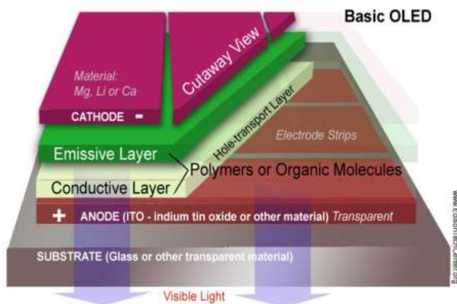
Fig 2: The figure is a simple modern OLED. There are many new ways to construct the OLED using a variety of layer configurations. Displays will have additional layers such as an active matrix TFT (thin film transistor) which control pixel regions.
