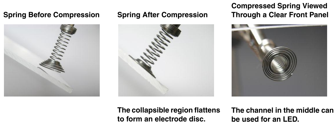
Figure 3-12. Compressing a Philipp Spring Product
