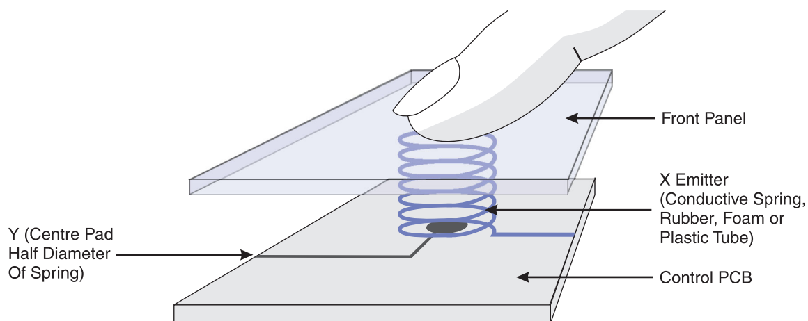
Figure 4-11. Using a Spring In a Mutual-capacitance Type Sensor
