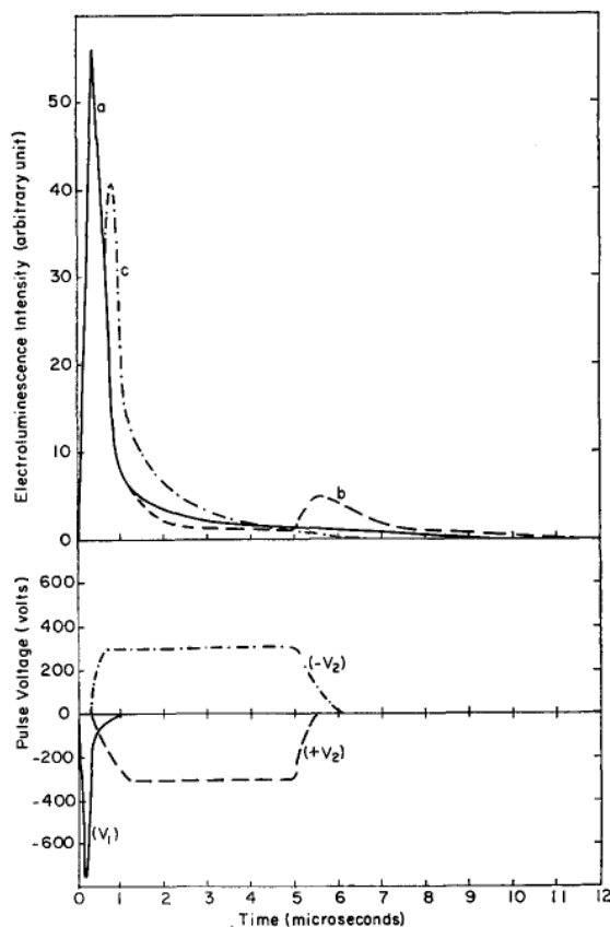
FIG. 1. Effect of electric field on delayed electroluminescence in anthracene crystal. Top: a, ( V_1 )=780 V, ( V_2 )=0 V; b, ( V_1 )=780 V, ( +V_2 )=320 V; c, ( V_1 )=780 V, ( -V_2 )=320 V. Crystal thickness: 20 \mu ; temperature: -67°C; pressure: 10 -6 mm Hg. Bottom: Pulse ( V_1 ) width: 0.1 \mu sec; pulse ( V_2 ) width: 4.4 \mu sec.
