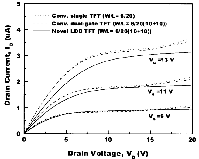
Fig. 4. Output characteristics of conventional single-, dual-gate, and novel LDD poly-Si TFT's.
