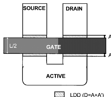
Fig. 1. Schematic structure of the novel LDD poly-Si TFT structure. The value of A (or A' ) is half of the total LDD length ( D ); A (or A' ) = D/2 .
