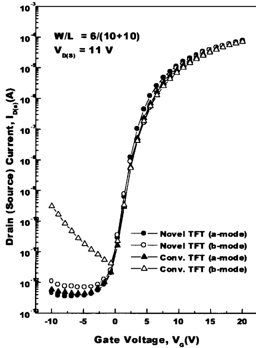
Fig. 2. I_D - V_G transfer characteristics of the conventional (Con.) and novel (New) poly-Si TFT's with the LDD length of 1.0\ \mu\text{m} . "a-mode" means that the current flows from drain ( V_d = 11\ \text{V} ) to source ( V_s = 0\ \text{V} ). "b-mode" means that the current flows from source ( V_s = 11\ \text{V} ) to drain ( V_d = 0\ \text{V} ).
