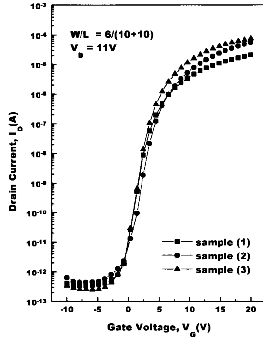
Fig. 3. I_D - V_G transfer characteristics of three novel poly-Si TFT samples where D = 1.5\ \mu\text{m} . Sample (1): A = 0\ \mu\text{m} , A' = D\ \mu\text{m} ; sample (2): A = D\ \mu\text{m} , A' = 0\ \mu\text{m} ; and sample (3): A = D/2\ \mu\text{m} , A' = D/2\ \mu\text{m} .
