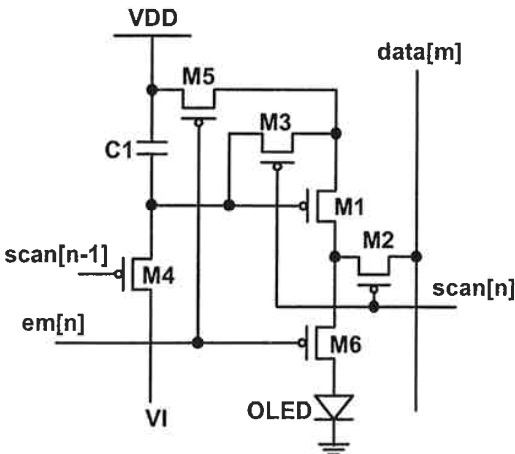
Figure 5. Modified example C of proposed pixel structure.
