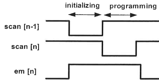
Figure 2. Timing diagram of proposed structure.
