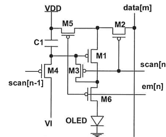
Figure 1. Proposed pixel structure.
