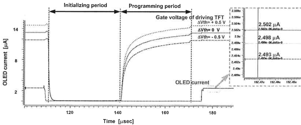
Figure 6. HSPICE simulation waveforms when I_{OLED} is maximum value.
