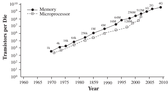
Fig. 1. A plot of circuit density per chip of Si memory and logic devices against year.
