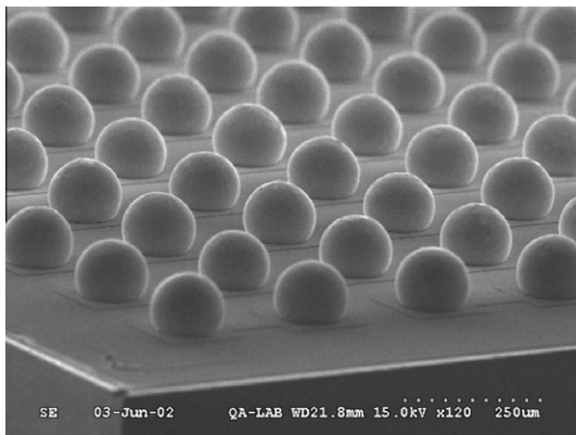
Fig. 2. SEM image of an array of solder balls on a chip surface.
