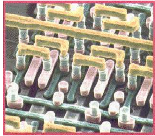
Fig. 7. Scanning electron microscopy (SEM) image of a two-level Al interconnect on a Si surface after the insulating dielectric has been etched away.
