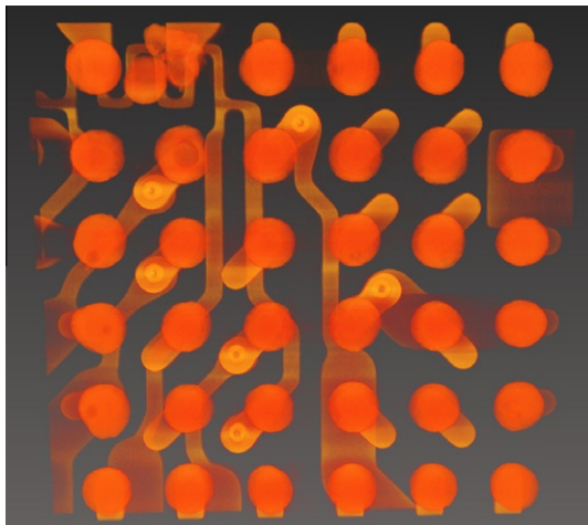
Fig. 8. Synchrotron radiation X-ray tomography image of an array of flip chip solder joints in chip size packaging. One of them at the upper left corner was failed by electromigration. (Courtesy of Miss Tian Tian, UCLA and Dao-Chih Chang, ITRI, Taiwan.)
