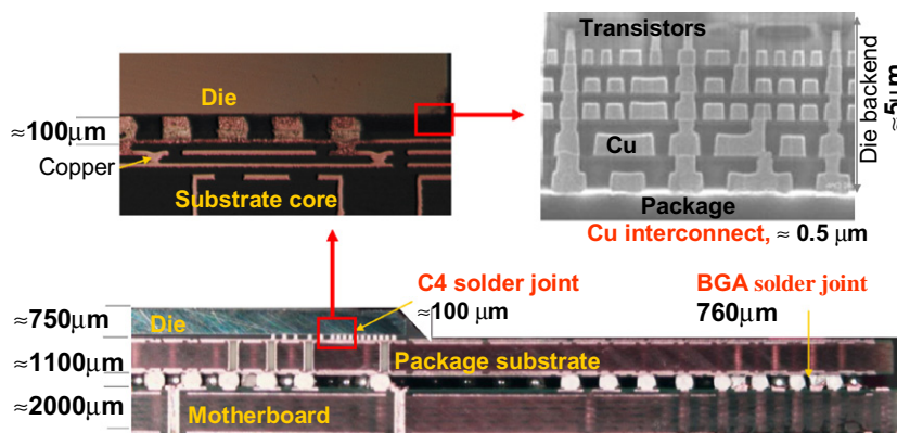
Fig. 3. SEM cross-sectional images of two levels of packaging technology where solder joints are used. (Courtesy of Yishao Lai, ASE, Taiwan.)
