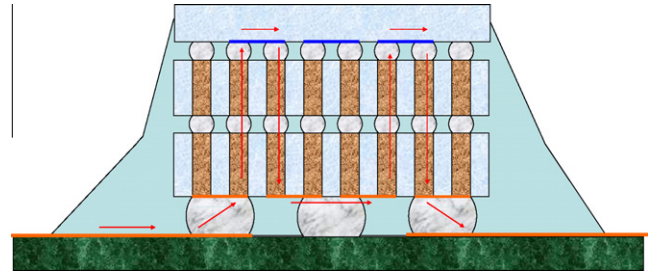
Fig. 4. Schematic diagram of the cross-section of vertical interconnects between the stacking of three wafers.
