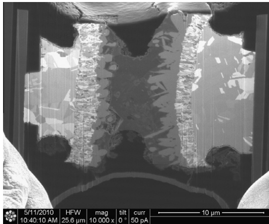
Fig. 6. A focused-ion-beam image of the cross-section of the metallization in a micro-bump. (Courtesy of Tian Tian, UCLA and Dao-Chih Chang, ITRI, Taiwan.)
