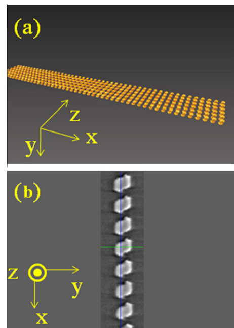
Fig. 5. (a) A synchrotron radiation X-ray tomography of an array of micro-bumps and (b) an enlarged X-ray tomography of the cross-sectional view of a row of micro-bumps. (Courtesy of Tian Tian, UCLA and Alastair Macdowell, ALS/LBNL.)
