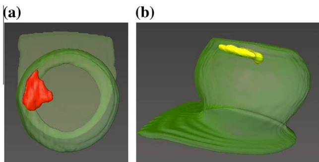
Fig. 9. Synchrotron radiation X-ray tomography images of a pancake void in a flip chip solder joint. (a) Top view, and (b) Side view. (Courtesy of Kai Chen, UCLA and Alastair Macdowell, ALS/LBNL.)
