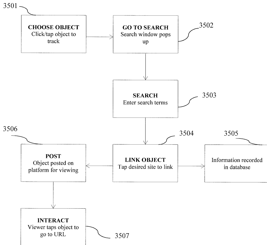
Fig. 35 Process flowchart
