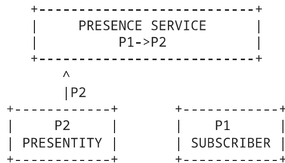
Fig. 3b: NOTIFICATION (Step 2)
