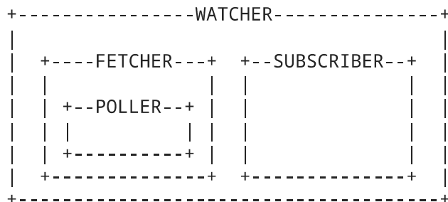
Fig. 2: Varieties of WATCHER
