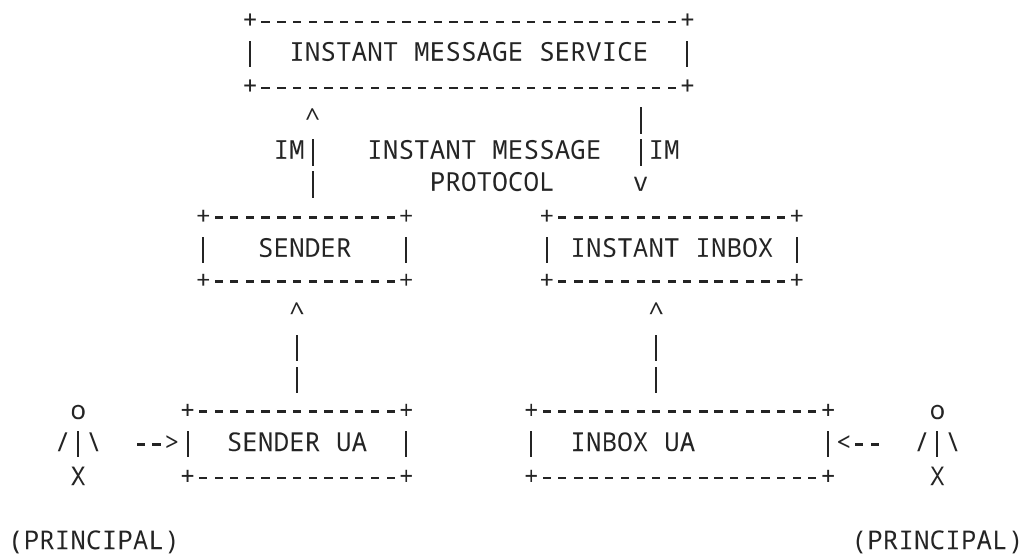
Fig. 7: An instant messaging system
