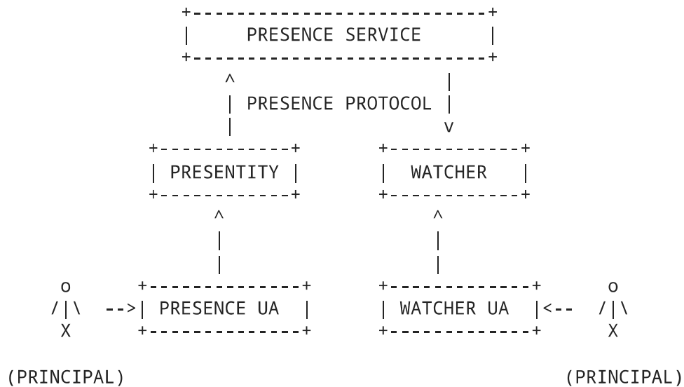
Fig. 6: A presence system
