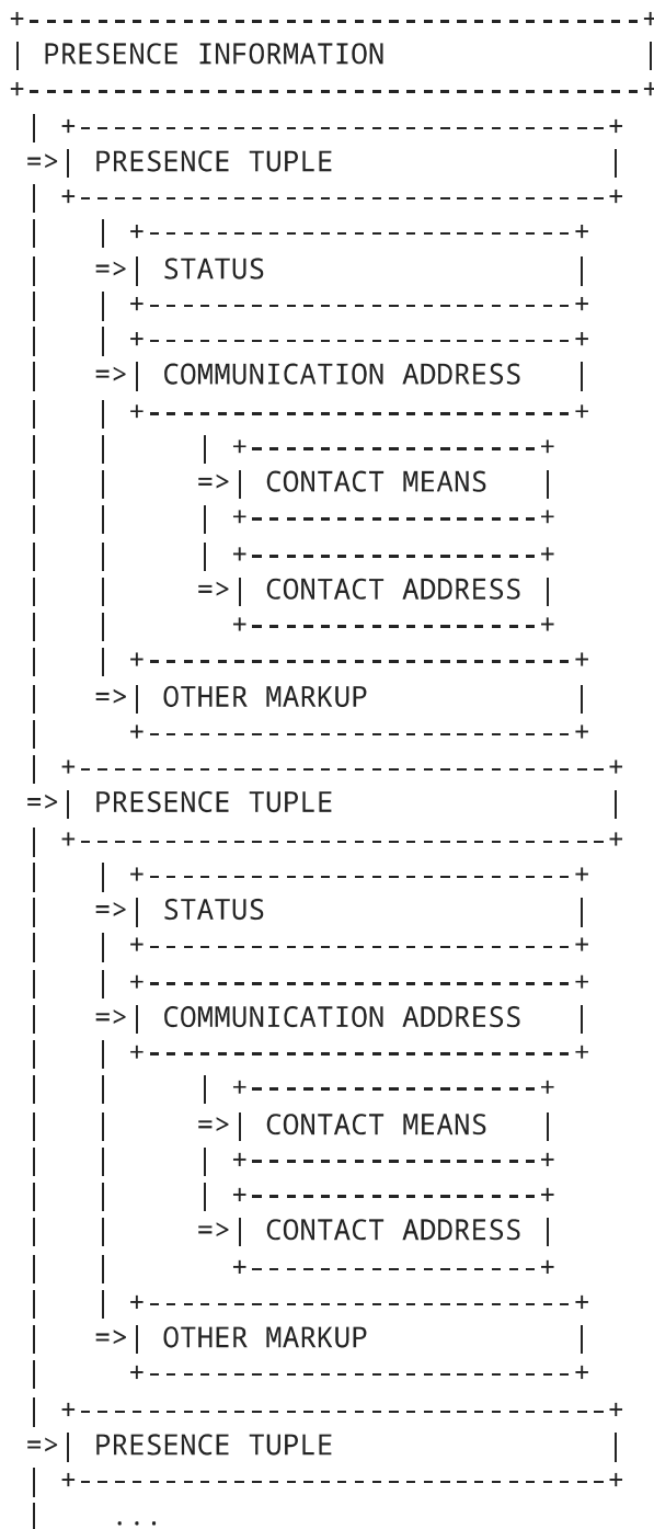
Fig. 5: The structure of PRESENCE INFORMATION
