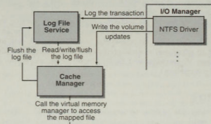
Figure 4-1. Log File Service (LFS)
