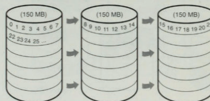
Figure 5-3. Logical Numbering of Physical Sectors on a Stripe Set
