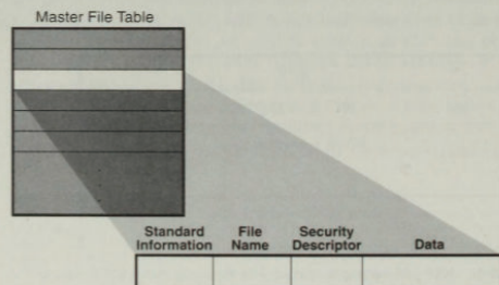
Figure 3-5. MFT Record for a Small File
