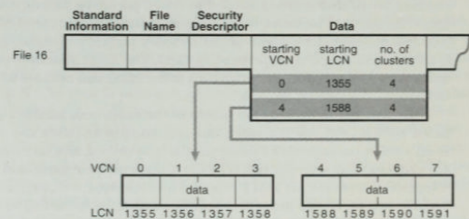
Figure 3-12. VCN-to-LCN Mappings for a Nonresident Data Attribute
