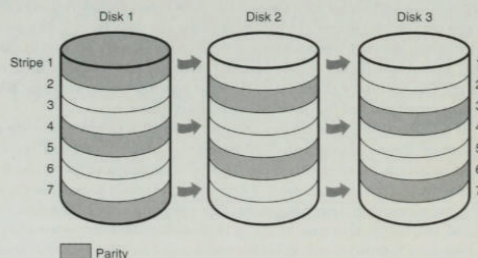
Figure 5-5. Stripe Set with Parity
