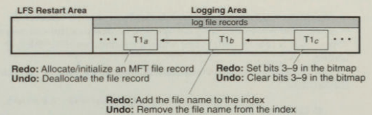
Figure 4-3. Update Records in the Log File
