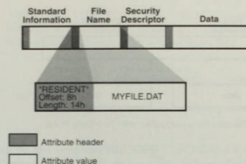
Figure 3-7. Resident Attribute Header and Value
