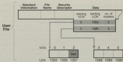
Figure 5-6. MFT Record for a User File with a Bad Cluster
