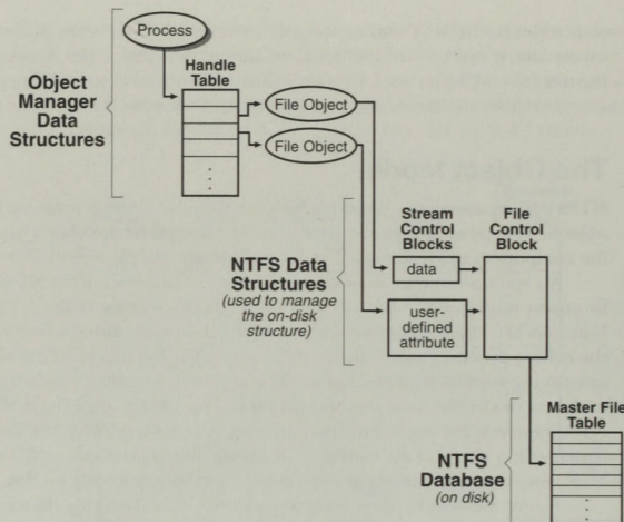
Figure 2-5. Locating an NTFS File
