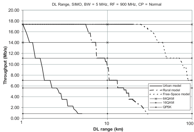
Figure 21.14: Throughput versus coverage.
