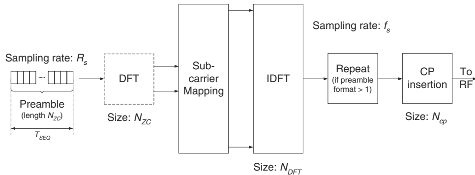
Figure 17.24: Functional structure of PRACH preamble transmitter.
