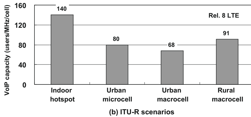
Figure 26.7: VoIP capacity of LTE Release 8 FDD.
