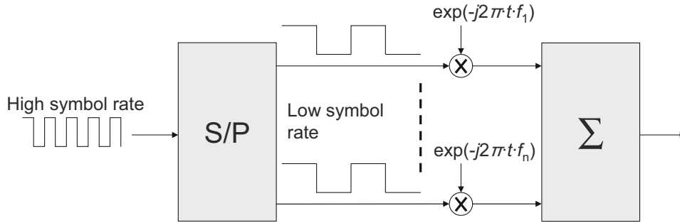
Figure 5.2: Serial-to-Parallel (S/P) conversion operation for OFDM.
