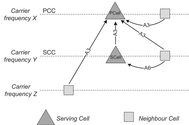
Figure 28.2: Measurement Events A3 and A6.
