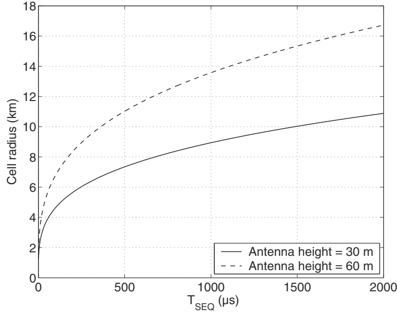
Figure 17.7: PRACH coverage performance versus sequence duration.
