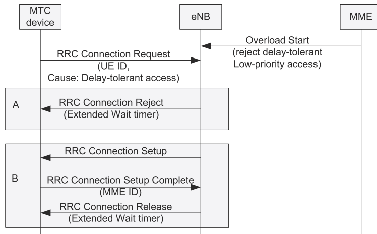
Figure 31.8: Mechanisms for handling CN overload.
