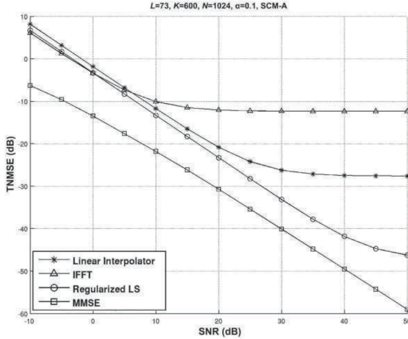
Figure 8.9: Frequency-domain channel estimation performance.
