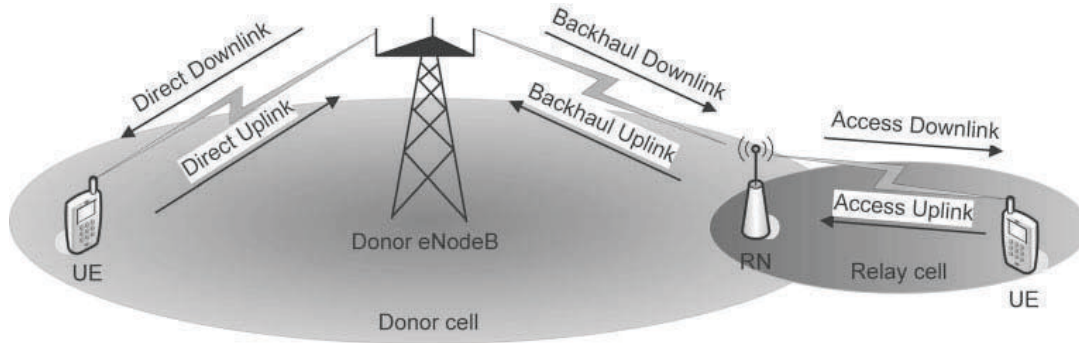
Figure 30.2: Terminology for relaying.
