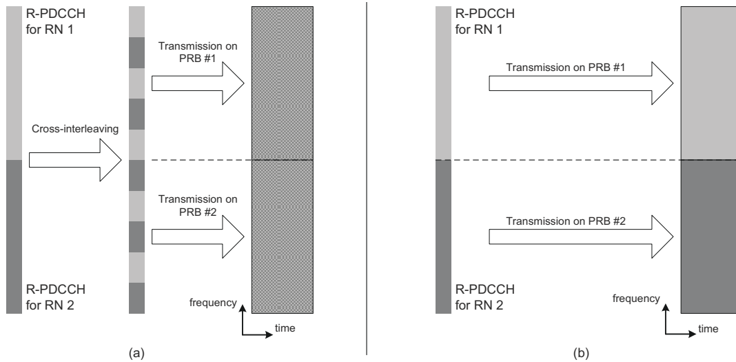
Figure 30.15: R-PDCCH formats: (a) cross-interleaved; (b) non-cross-interleaved.
