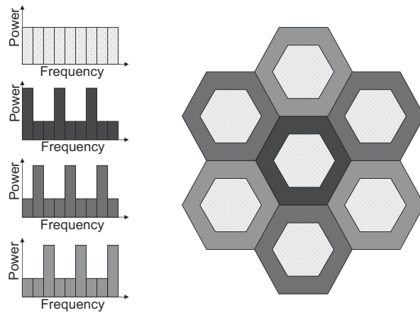
Figure 12.6: Partial frequency reuse.
