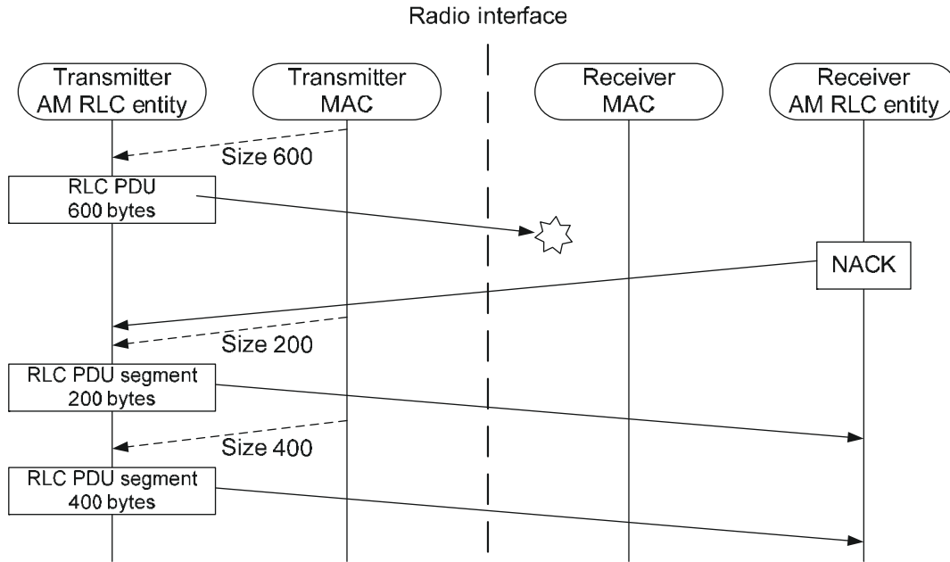
Figure 4.11: Example of RLC resegmentation.
