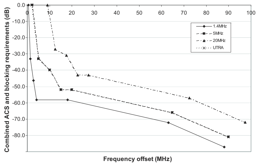
Figure 21.17: Selectivity and blocking requirements.
