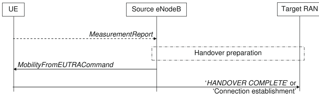
Figure 3.8: Mobility from LTE.
