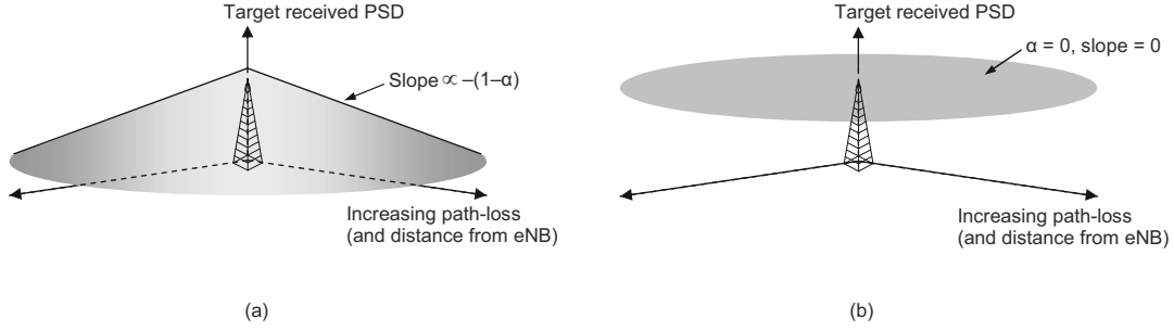
Figure 18.4: (a) Fractional and (b) non-fractional power control.
