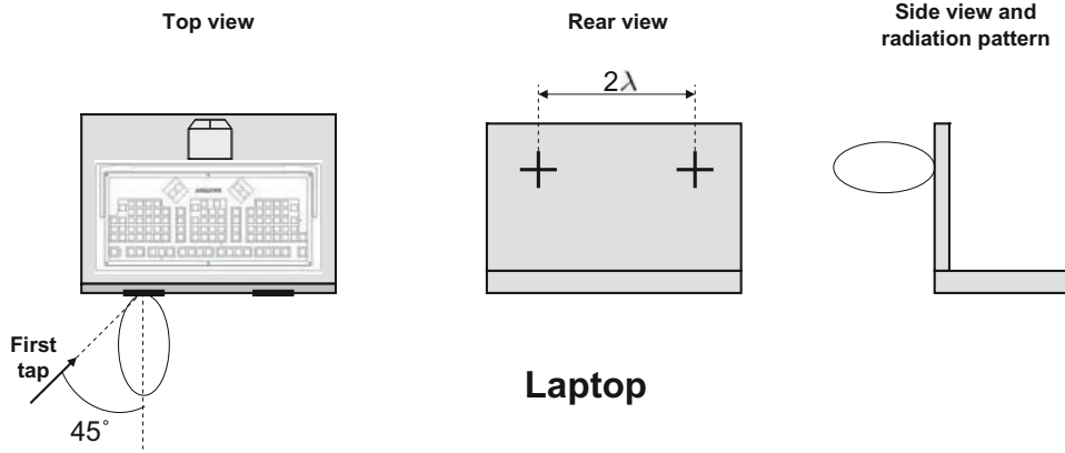
Figure 20.5: Laptop antenna configuration.
