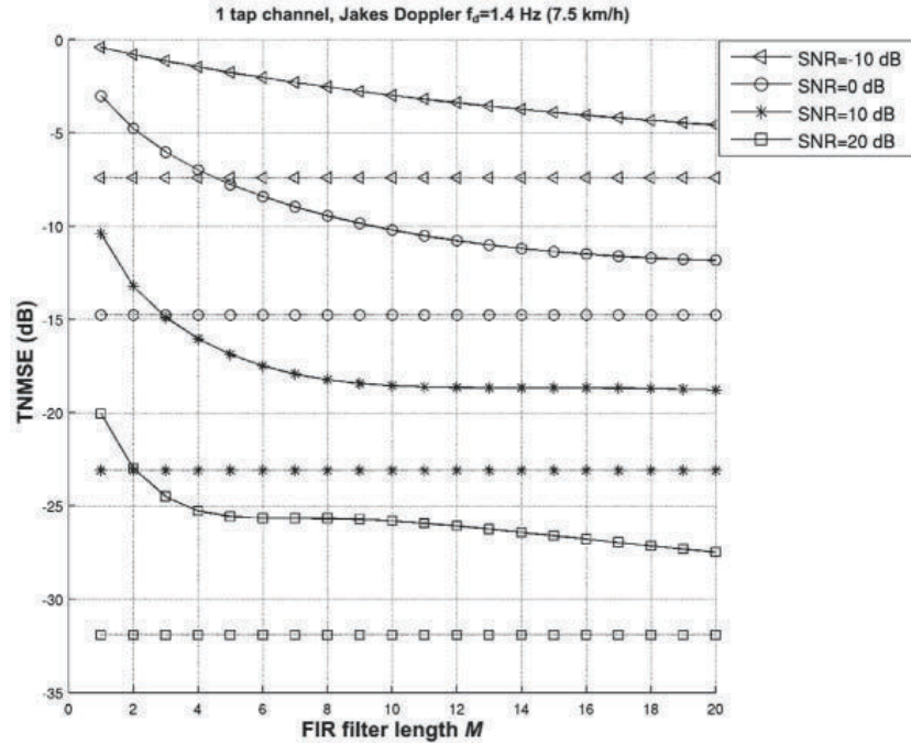
Figure 8.11: Time-domain channel estimation performance.
