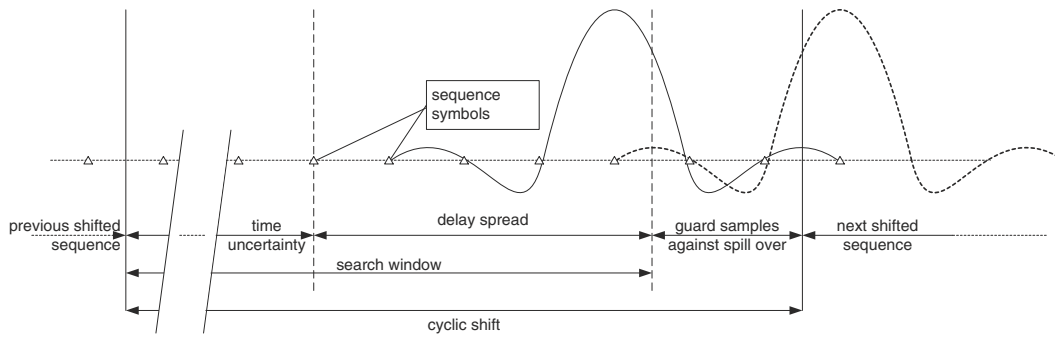
Figure 17.15: Cyclic shift dimensioning.
