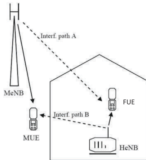
Figure 24.4: Macro/femto downlink interference scenarios.
