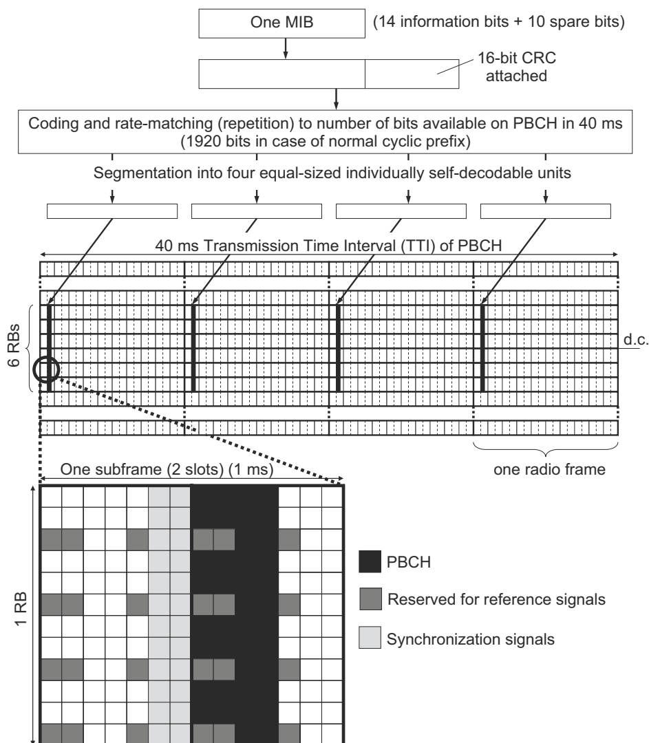
Figure 9.1: PBCH structure.
