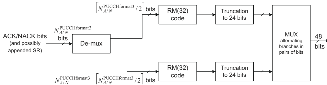
Figure 28.10: Coding and scrambling for PUCCH format 3.
