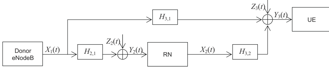
Figure 30.5: The general Gaussian relay channel model in the context of downlink transmission in an RN-assisted cellular network. The same model can be applied to the uplink case, with the UE and the donor eNodeB reversed.
