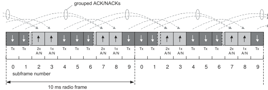
Figure 23.12: Grouped ACK/NACK transmission in TDD operation.
