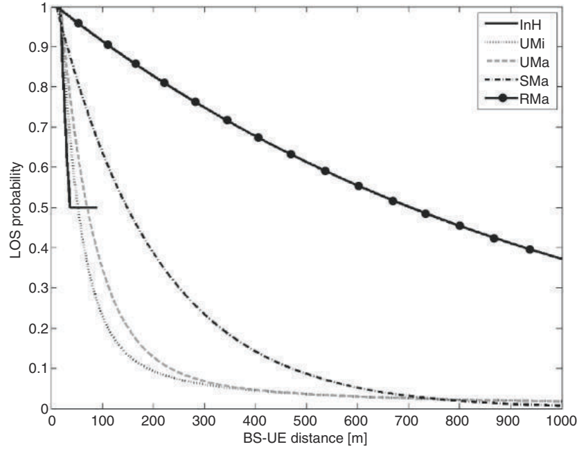
Figure 20.7: LOS probabilities for the ITU deployment scenarios.
