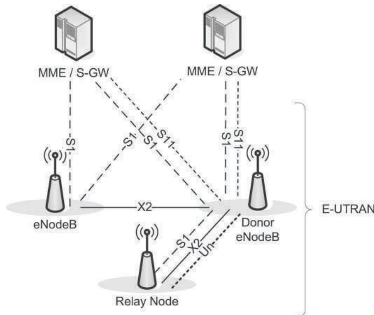
Figure 30.10: Network architecture and interfaces for RNs.
