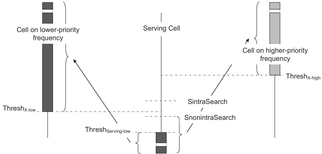
Figure 3.13: Frequency/RAT evaluation.
