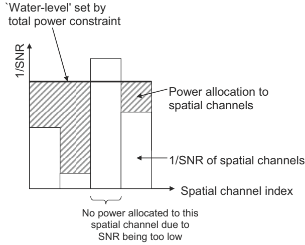
Figure 11.3: The waterfilling principle for optimal power allocation.
