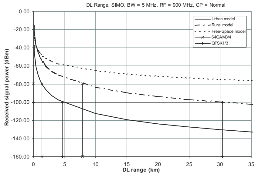
Figure 21.13: Downlink coverage taking receiver sensitivity into account.
