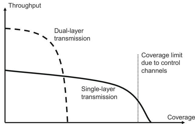
Figure 11.8: Trade-off between throughput and coverage with beamforming.
