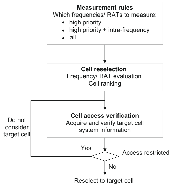
Figure 3.12: Cell reselection.
