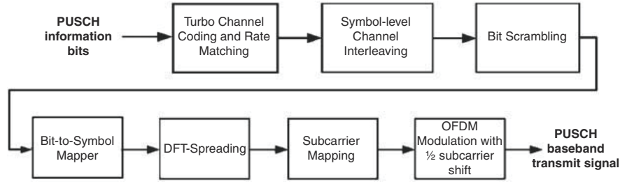
Figure 16.2: Uplink physical data channel processing.
