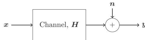
Figure 8.1: A simple transmission model.
