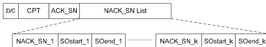
Figure 4.15: STATUS PDU format.
