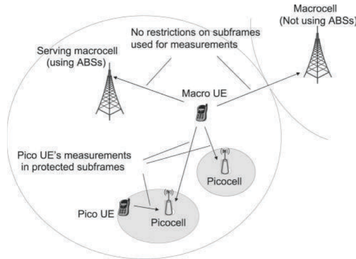
Figure 31.5: UE measurements of serving and neighbour cells.
