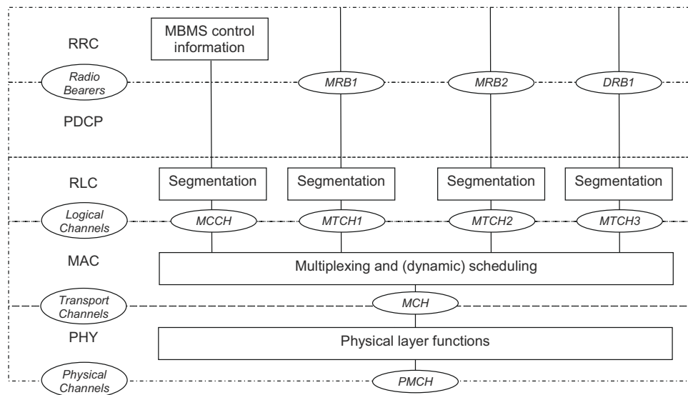
Figure 13.8: LTE protocol extensions to support MBMS.
