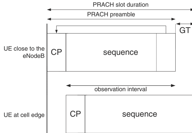
Figure 17.6: PRACH preamble received at the eNodeB.
