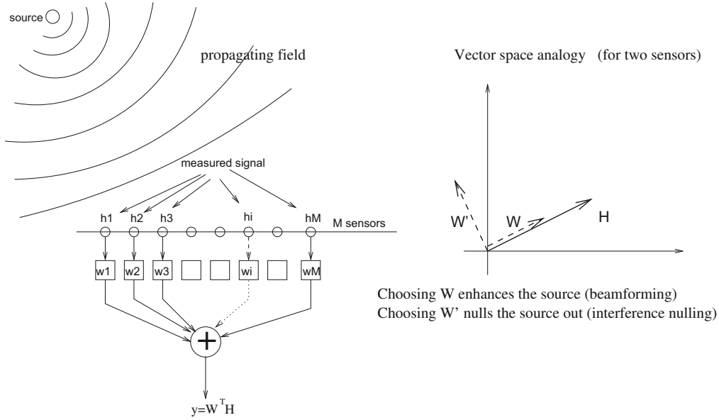
Figure 11.4: The beamforming and interference cancelling concepts.
