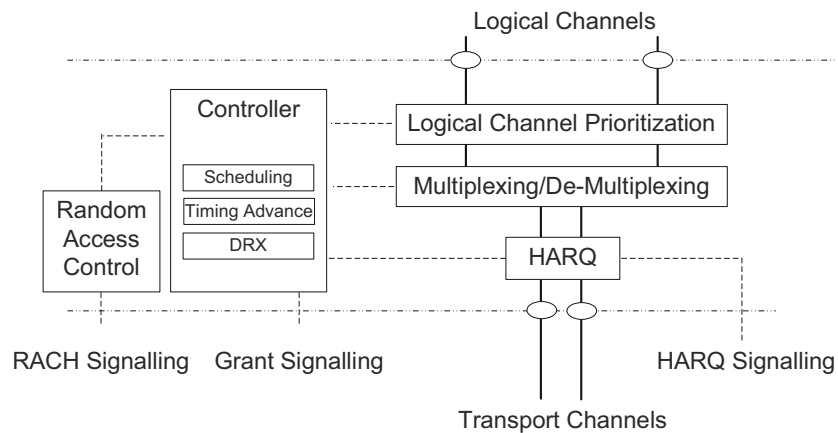
Figure 4.16: Conceptual overview of the UE-side MAC architecture.
