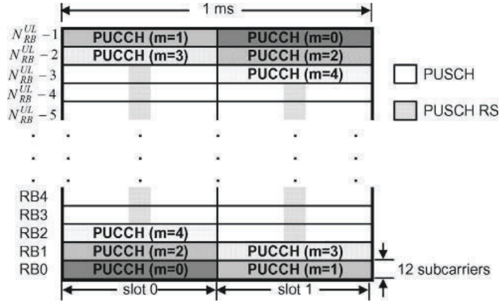
Figure 16.7: Example of an odd number of PUCCH regions ( N_{RB}^{UL} = 5 ).
