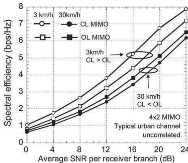
Figure 11.9: Example of closed-loop and open-loop MIMO performance.
