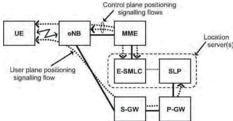
Figure 19.8: CP and UP architecture for positioning.
