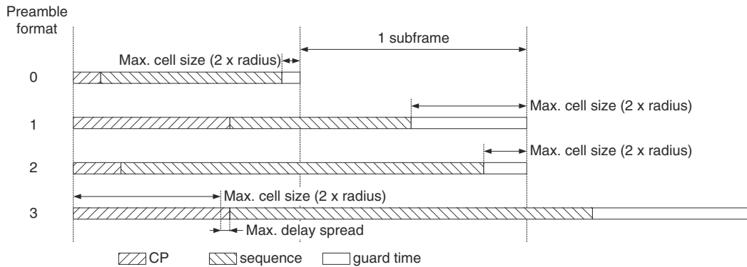
Figure 17.9: PRACH preamble formats and cell size dimensioning.
