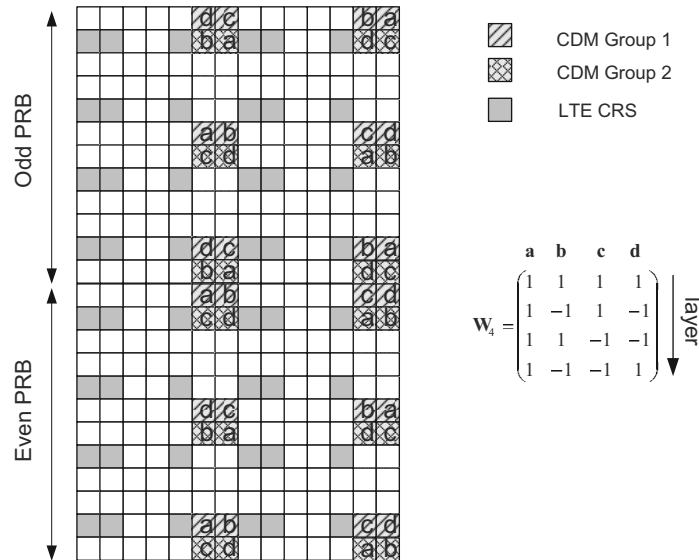
Figure 29.2: Length-4 OCC mapping to REs.
