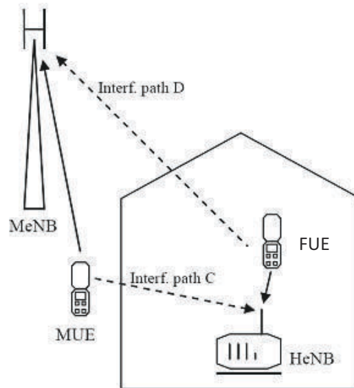
Figure 24.5: Macro/femto uplink interference scenarios.
