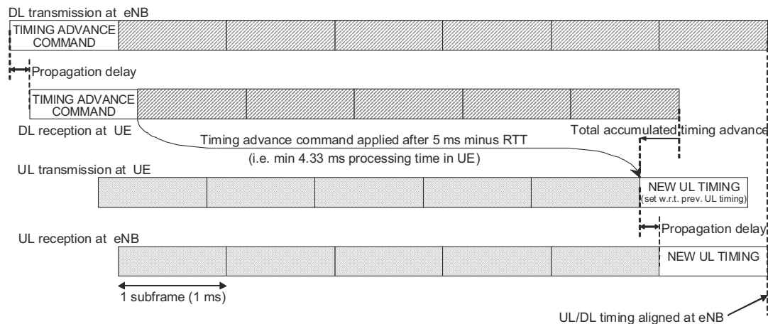
Figure 18.2: Application of timing advance update commands.
