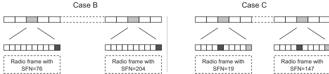
Figure 3.14: Paging frame and paging occasion examples.
