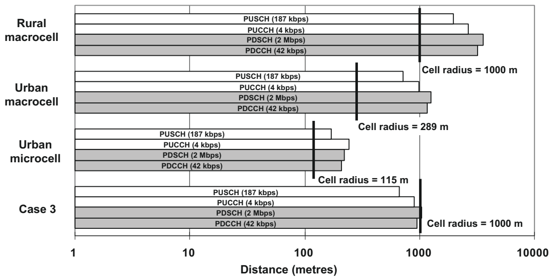
Figure 26.8: LTE coverage (10 MHz, FDD).
