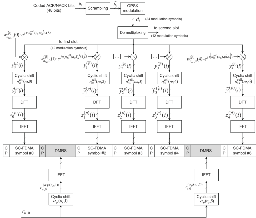
Figure 28.9: Structure of PUCCH format 3.
