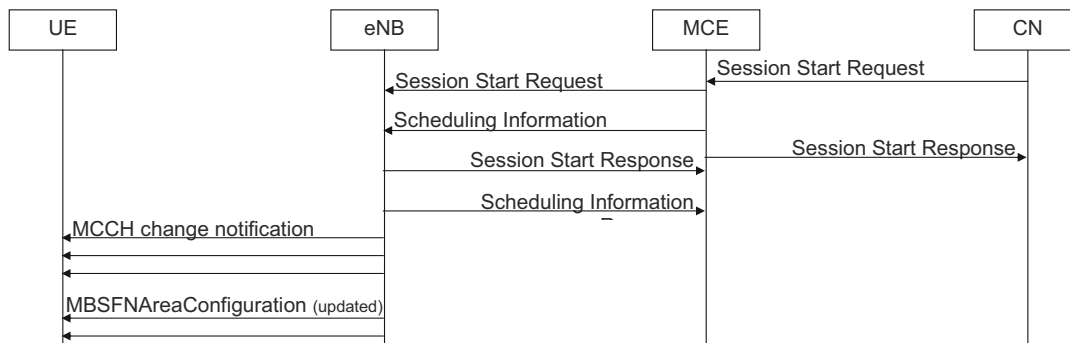
Figure 13.9: The MBMS session start message sequence.
