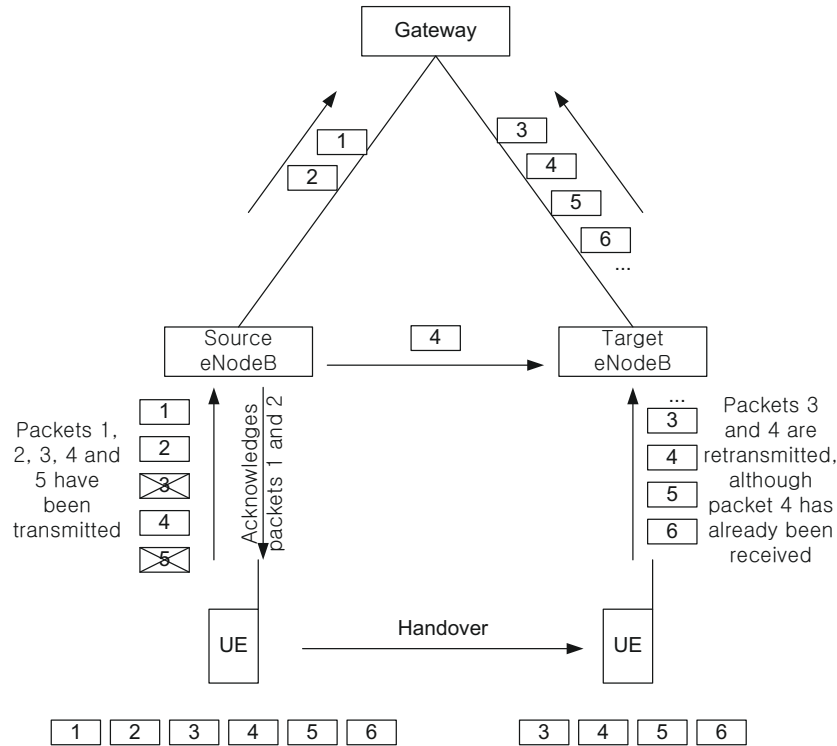
Figure 4.4: Lossless handover in the uplink.
