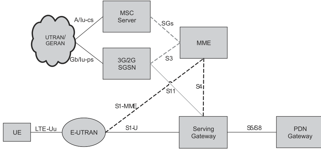
Figure 2.10: Architecture for 3G UMTS interworking.
