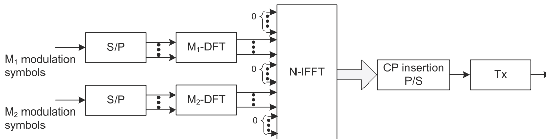
Figure 28.12: Block diagram of multiple SC-FDMA.
