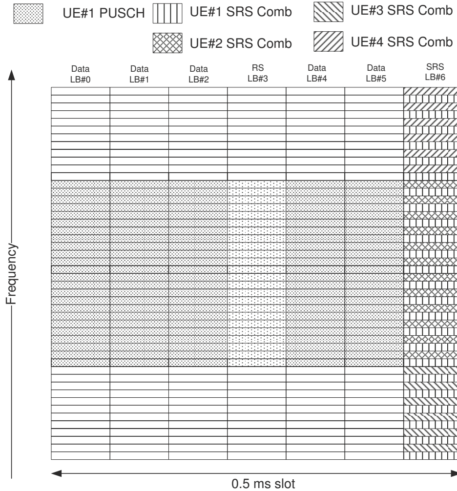
Figure 15.9: SRS symbol structure with RPF = 2.
