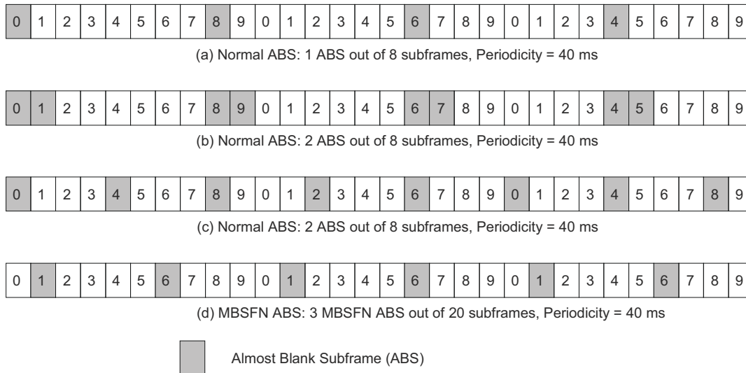
Figure 31.7: Examples of ABS patterns.
