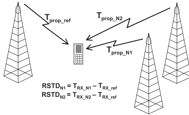
Figure 19.2: Basic principle of OTDOA in LTE.
