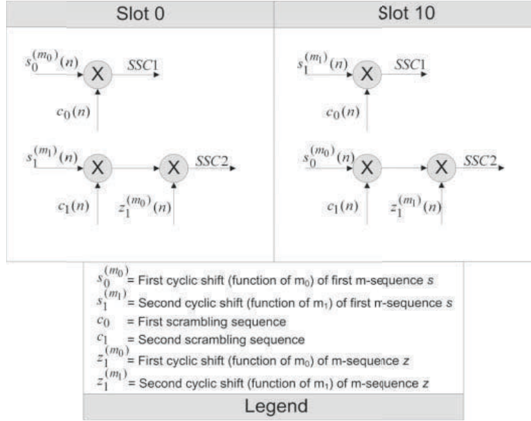
Figure 7.12: SSS sequence generation.
