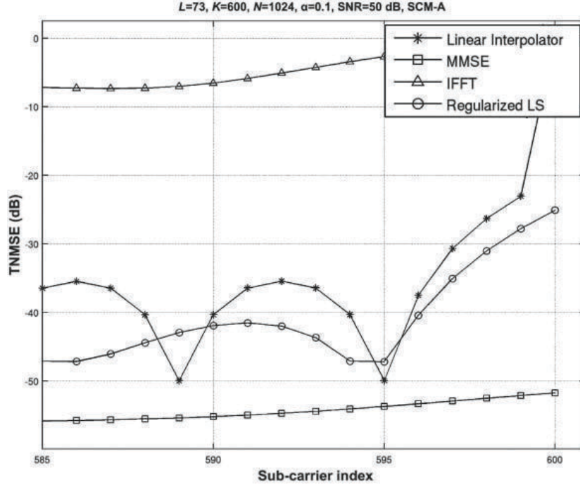
Figure 8.10: Band-edge behaviour of frequency-domain channel estimation.
