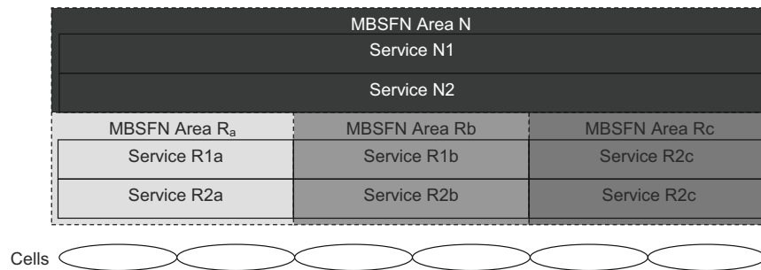
Figure 13.6: Example scenario with overlapping MBSFN areas.
