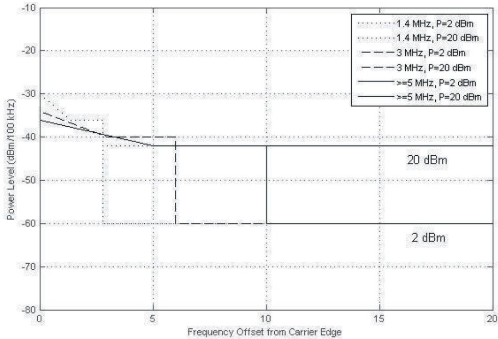
Figure 24.7: Spectrum Emission Mask for Home eNodeB class.
