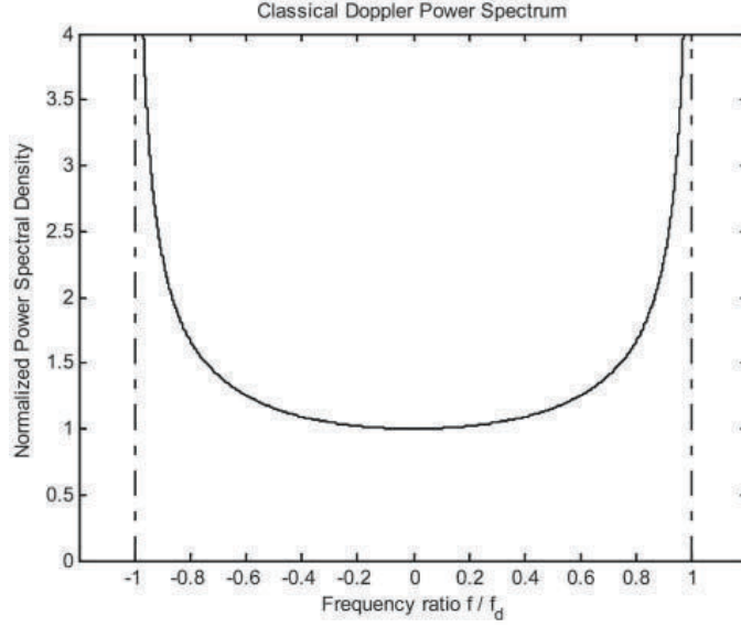
Figure 8.8: Normalized PSD for Clarke's model.
