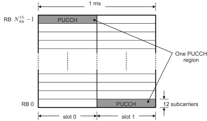
Figure 16.4: A PUCCH region.
