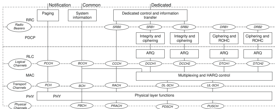
Figure 3.1: Radio architecture.
