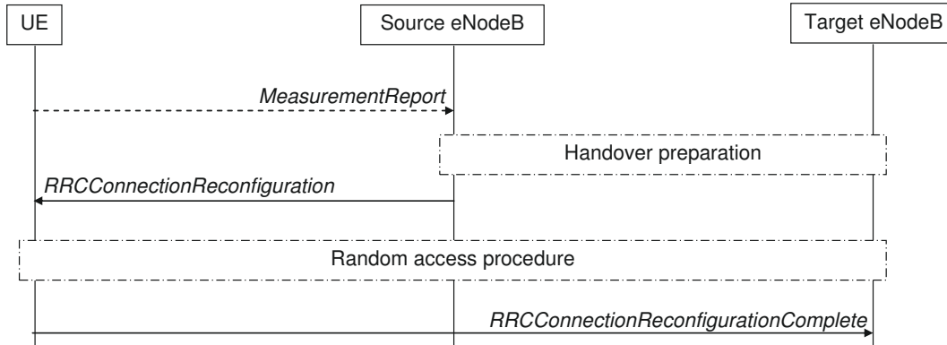
Figure 3.7: Handover within LTE.
