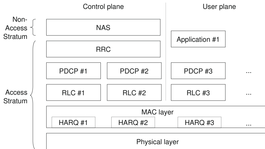
Figure 4.1: Overview of user-plane architecture.
