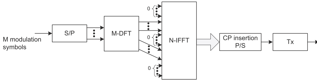
Figure 28.11: Block diagram of clustered DFT-S-OFDM.
