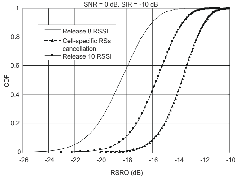
Figure 31.6: RSSI measurement modification.
