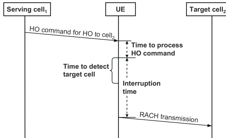
Figure 22.7: Handover to an unknown target cell.
