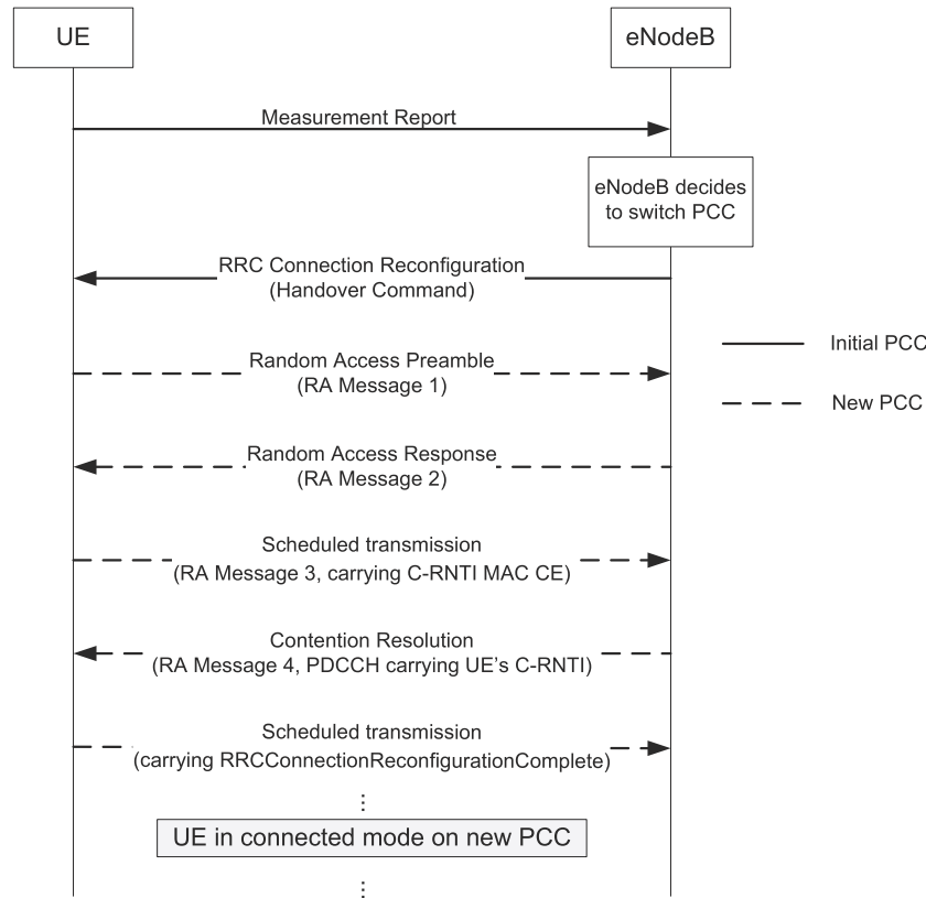
Figure 28.1: Procedure for PCell change with contention-based handover.
