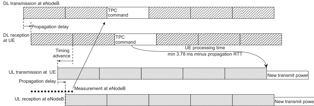
Figure 18.5: Timing of the uplink power control loop.
