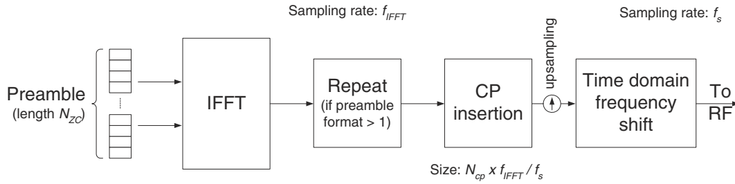
Figure 17.25: Hybrid frequency/time domain PRACH generation.
