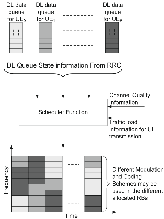
Figure 12.2: Generic view of a wideband resource scheduler.
