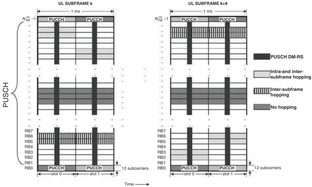
Figure 16.3: Uplink physical data channel processing.
