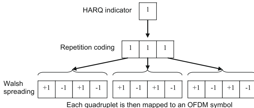
Figure 9.7: An example of PHICH signal construction.
