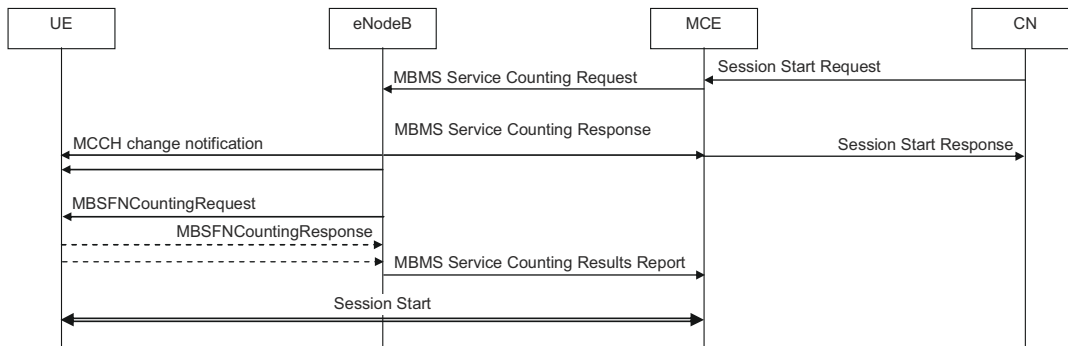
Figure 13.13: MBMS counting upon session start.
