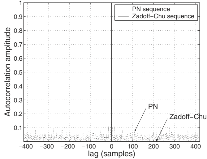
Figure 7.5: Zadoff–Chu versus PN sequence: periodic autocorrelation.
