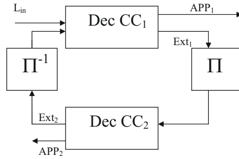
Figure 10.7: Schematic turbo decoder representation.
