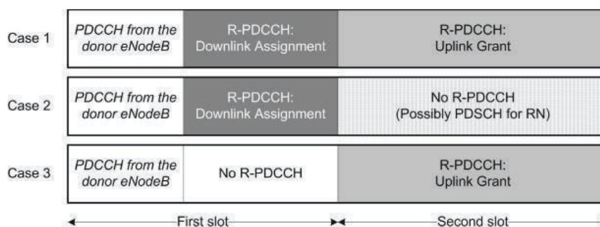
Figure 30.16: Supported R-PDCCH/PDSCH multiplexing possibilities.
