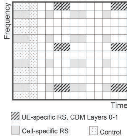
Figure 8.6: Dual-layer UE-specific RS arrangement in Release 9.
