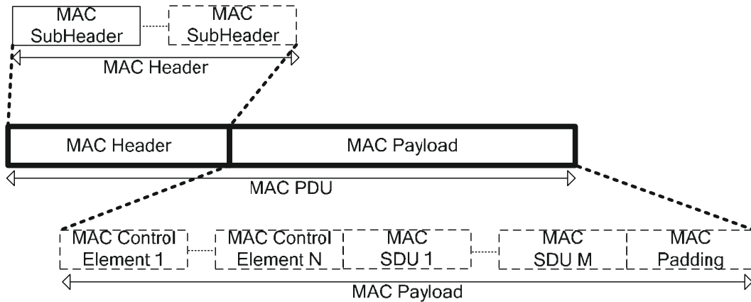
Figure 4.21: General MAC PDU format.
