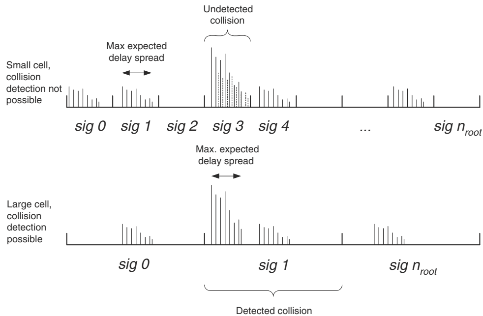
Figure 17.29: Collision detection.
