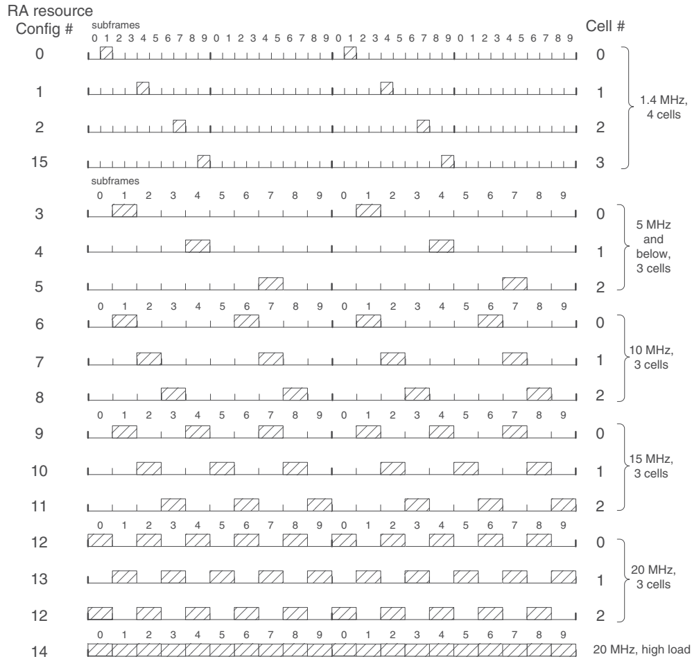
Figure 17.11: Random Access resource configurations.
