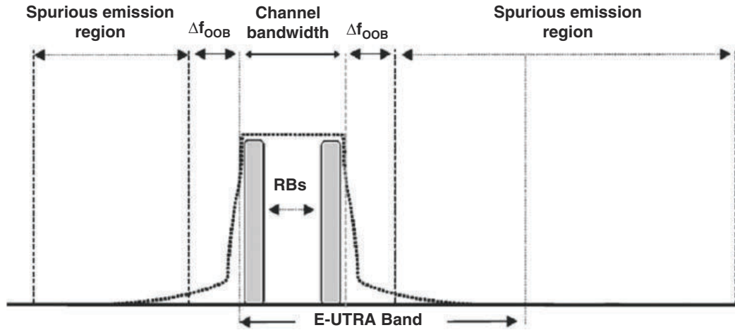
Figure 21.5: Transmitter spectrum. Reproduced by permission of © 3GPP.
