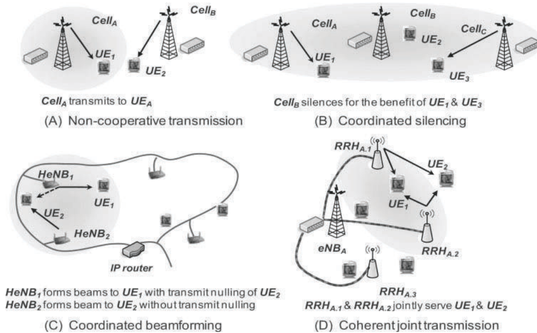
Figure 29.11: Downlink transmission schemes:
