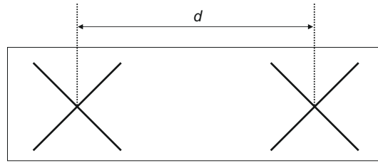
Figure 20.3: Base station antenna configuration.
