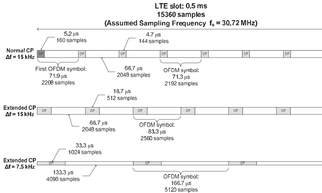
Figure 5.13: LTE OFDM symbol and CP lengths.
