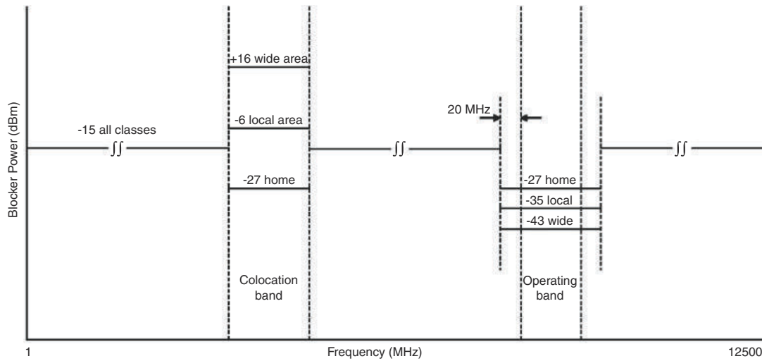
Figure 24.8: Blocking requirements.
