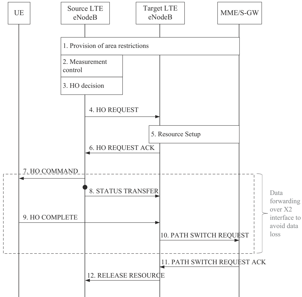
Figure 2.19: X2-based handover procedure.
