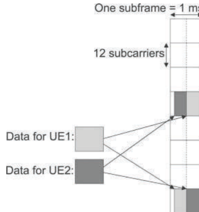
Figure 9.3: Frequency-distributed data mapping in LTE downlink.
