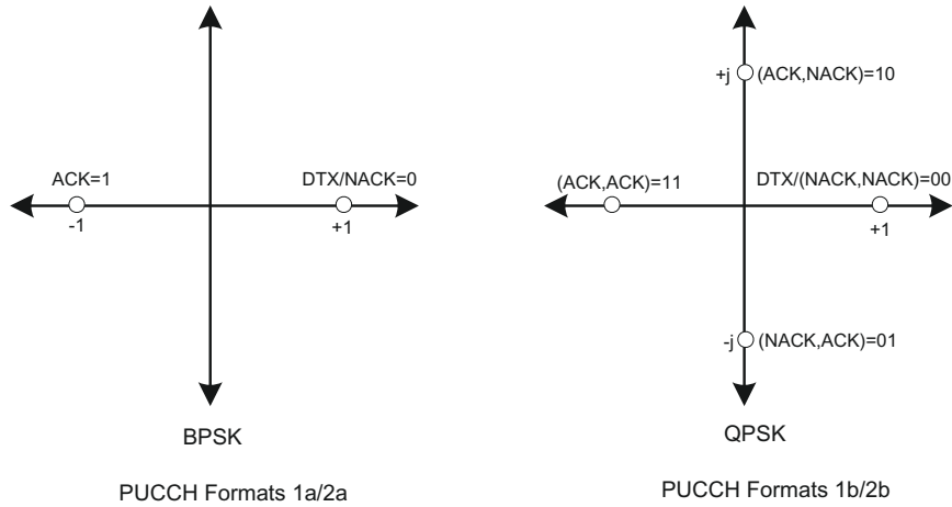
Figure 16.10: Constellation mapping for HARQ ACK/NACK.
