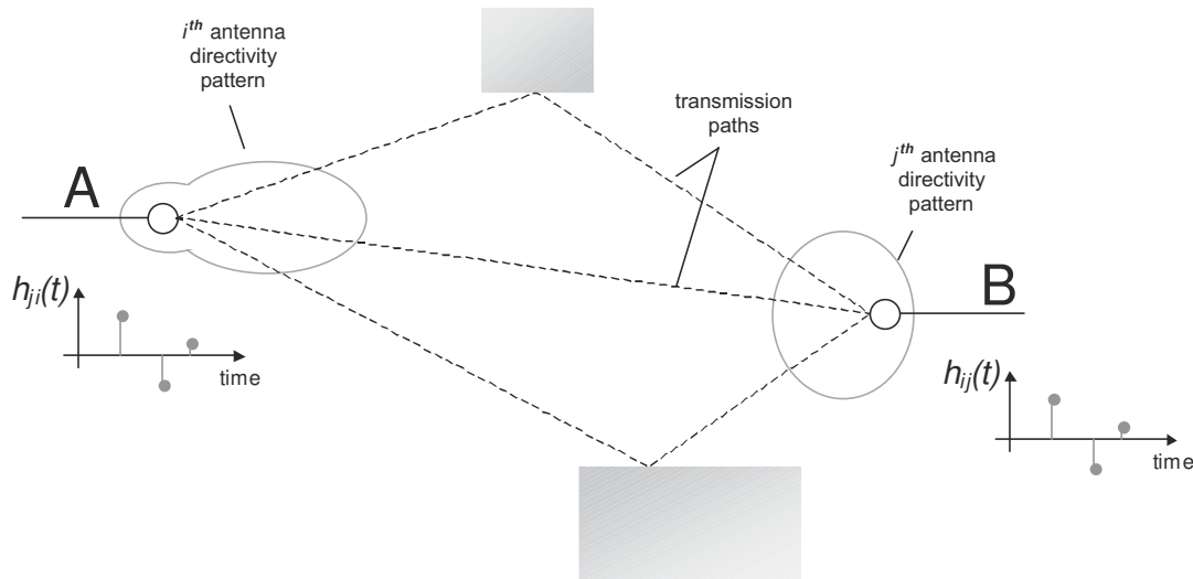
Figure 23.13: Reciprocity between a pair of transceivers.
