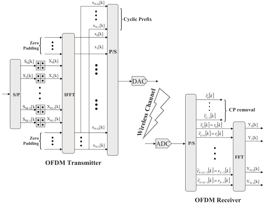
Figure 5.4: OFDM system model: (a) transmitter; (b) receiver.
