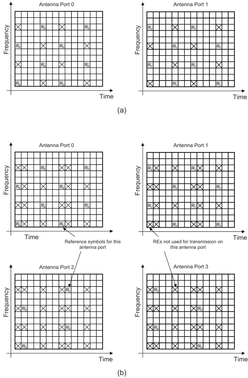
Figure 8.3: Cell-specific RS arrangement in the case of normal CP length for (a) two antenna ports, (b) four antenna ports. Reproduced by permission of © 3GPP.
