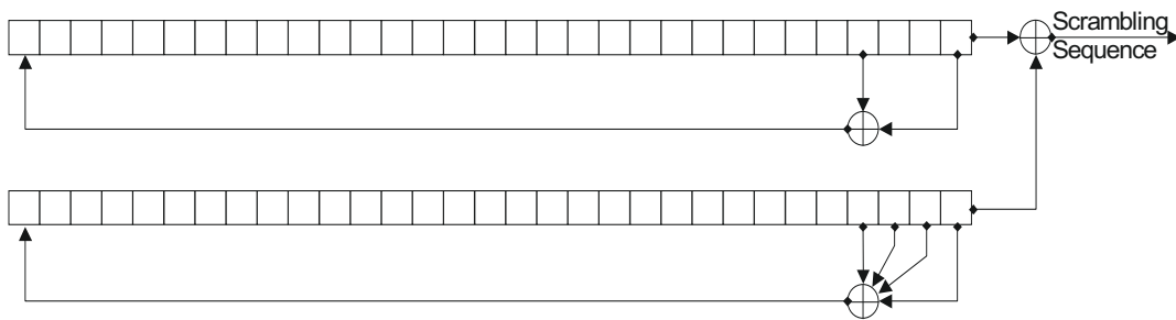
Figure 6.4: Shift-register implementation of scrambling sequence generator.
