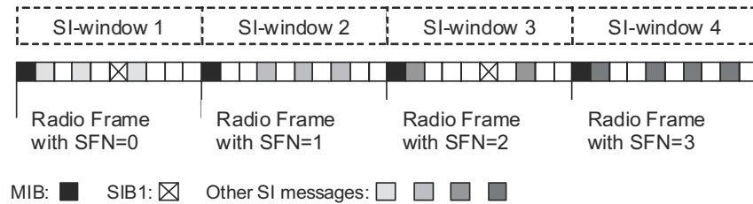
Figure 3.2: SI scheduling example.
