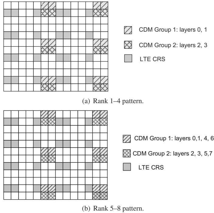
Figure 29.1: Release 10 UE-specific RS patterns.
