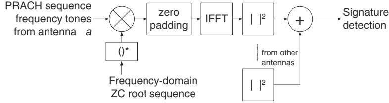
Figure 17.27: PDP computation per root sequence.
