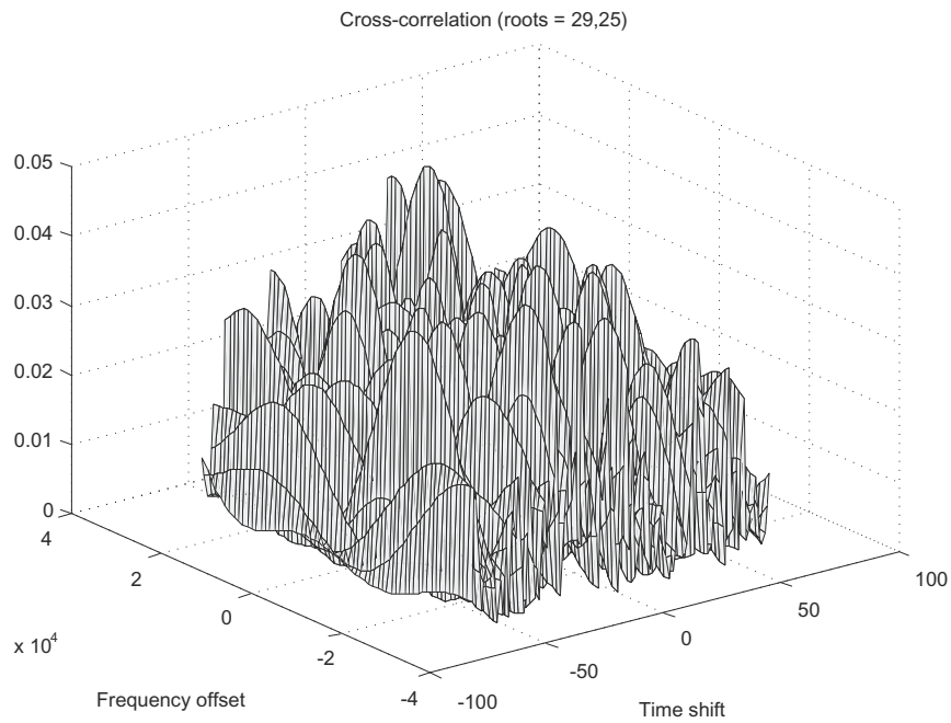
Figure 7.8: Cross-correlation of the PSS sequence pair 25 and 29.
