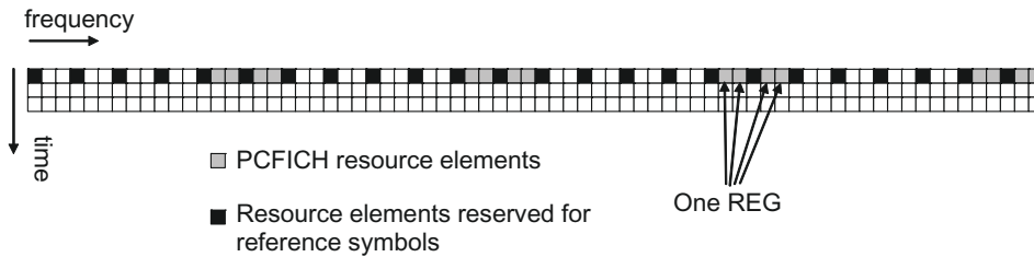
Figure 9.6: PCFICH mapping to Resource Element Groups (REGs).
