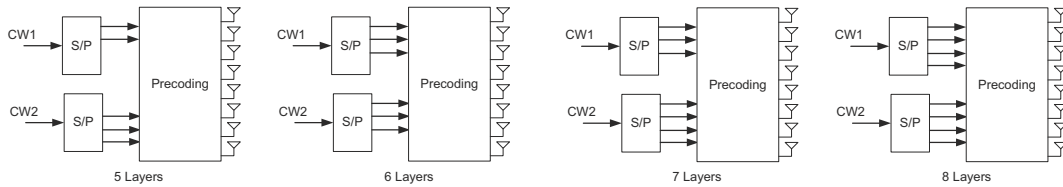
Figure 29.7: Codeword-to-layer mapping for up to 8 antenna ports.
