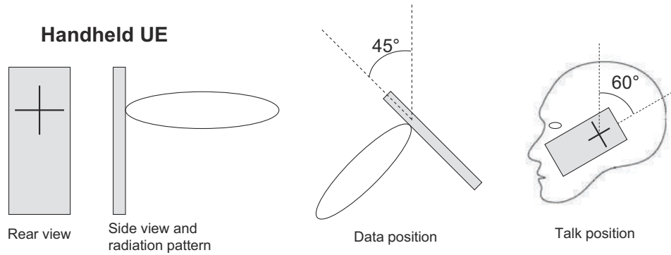
Figure 20.4: Handset antenna configuration.
