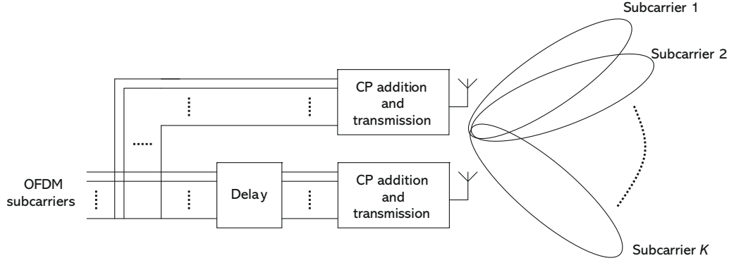
Figure 11.7: Principle of Cyclic Delay Diversity.
