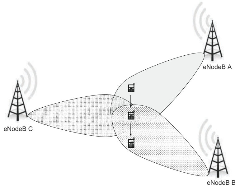
Figure 25.5: Handover to an inappropriate cell.
