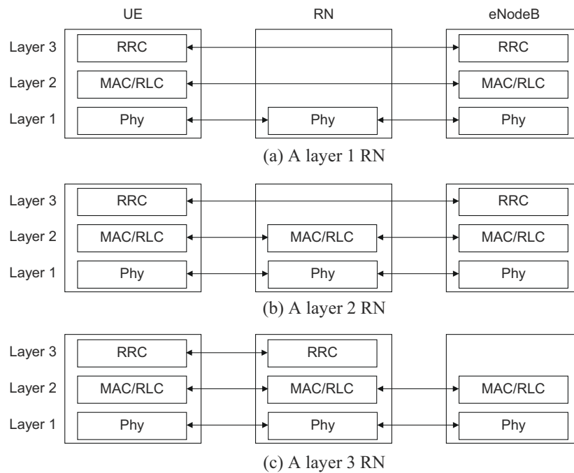
Figure 30.3: Protocol stack alternatives for an RN.
