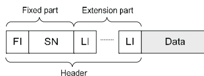
Figure 4.12: Key features of UMD PDU format.
