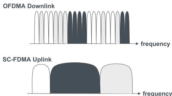
Figure 1.4: Frequency-domain view of the LTE multiple-access technologies.
