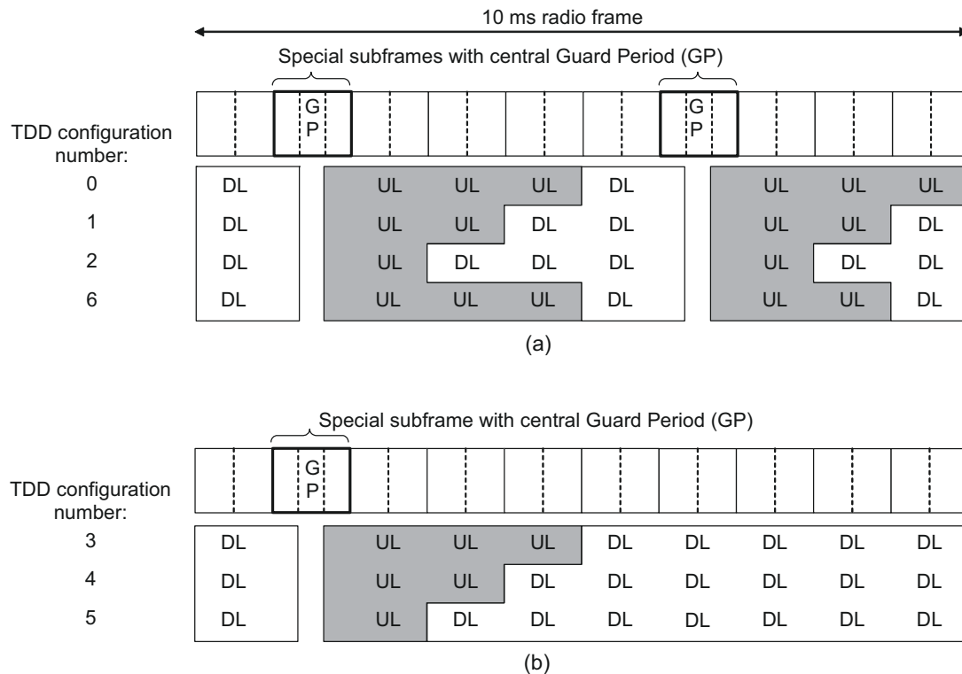
Figure 6.2: LTE subframe structure for TDD operation:
