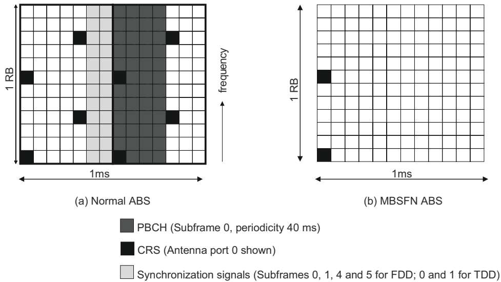
Figure 31.3: Normal and MBSFN Almost Blank Subframes.
