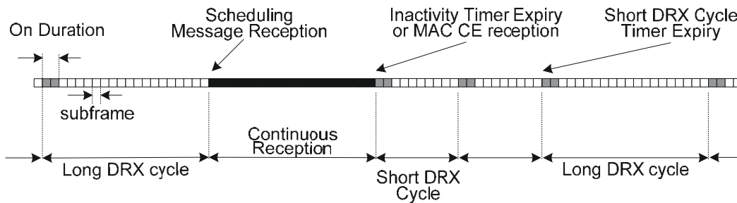
Figure 4.19: The two-level DRX procedure.
