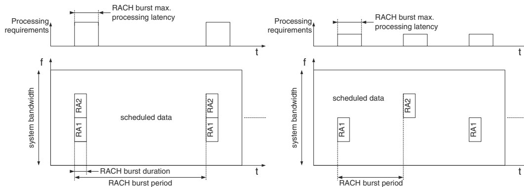
Figure 17.10: Processing peaks of the random access preamble receiver.
