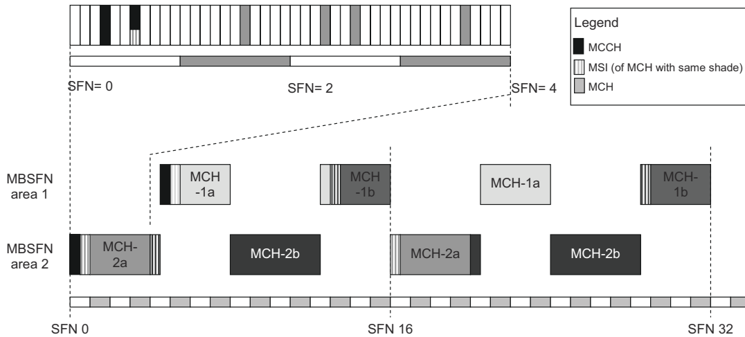
Figure 13.11: An example of MBMS resource allocation.
