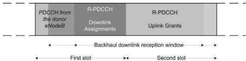
Figure 30.14: Placement of the R-PDCCH.
