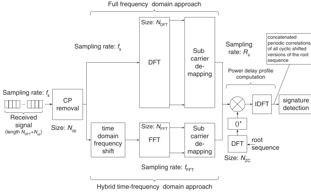
Figure 17.26: PRACH receiver options.
