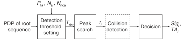
Figure 17.28: Signature detection per root sequence.
