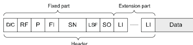
Figure 4.14: Key features of AMD PDU segment format.
