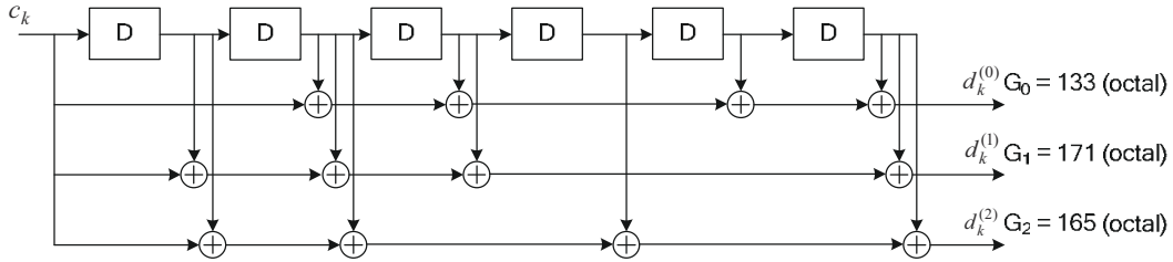
Figure 10.2: Rate 1/3 convolutional encoder used in LTE with m = 6 , n = 3 , k = 1 [10].
