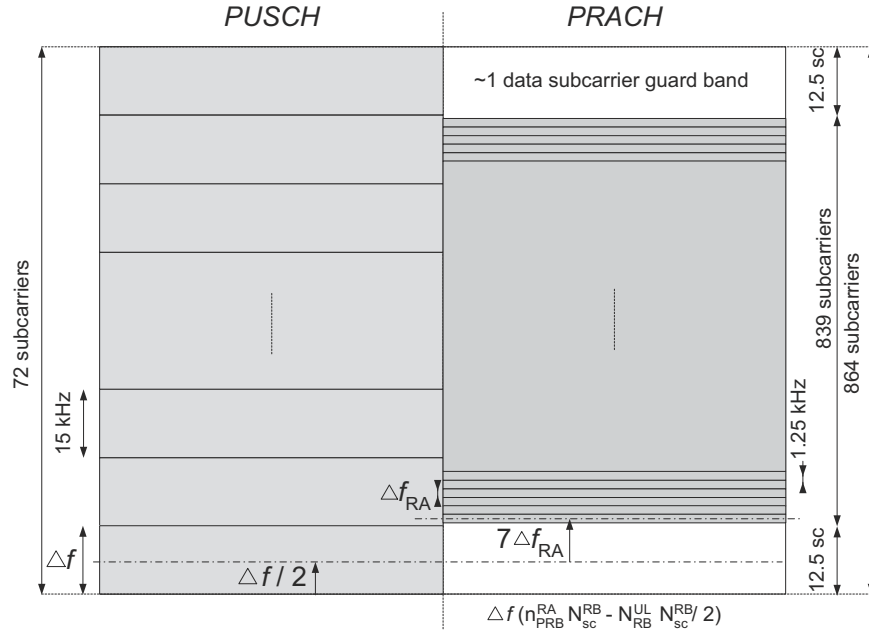
Figure 17.14: PRACH preamble mapping onto allocated subcarriers.
