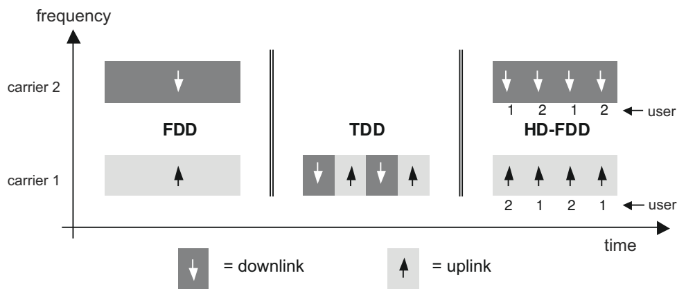
Figure 23.1: FDD, TDD and HD-FDD duplex modes.
