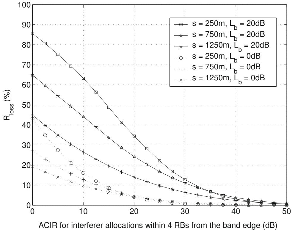
Figure 23.6: Throughput reduction due to UE-to-UE interference.
