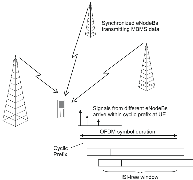
Figure 13.3: ISI-free operation with MBSFN transmission.
