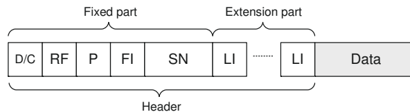
Figure 4.13: Key features of AMD PDU format.
