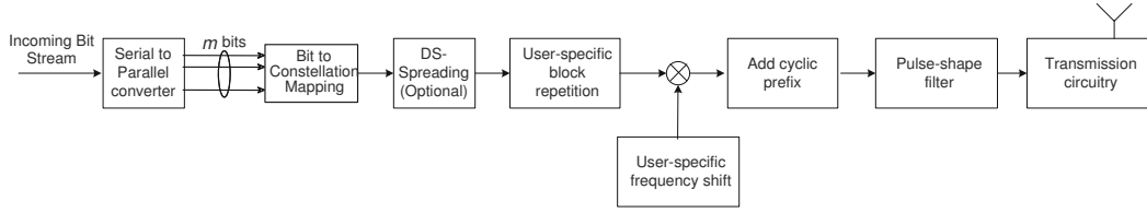
Figure 14.1: SC-FDMA time-domain transmit processing.
