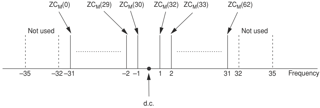
Figure 7.6: PSS sequence mapping in the frequency domain.
