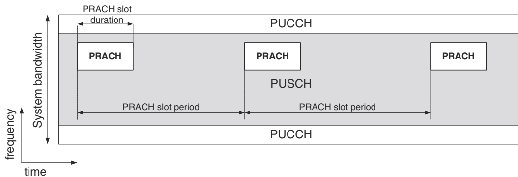
Figure 17.5: PRACH multiplexing with PUSCH and PUCCH.
