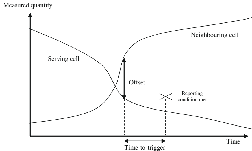
Figure 3.10: Event triggered report condition (Event A3).
