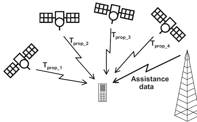
Figure 19.1: Basic principle of A-GNSS.
