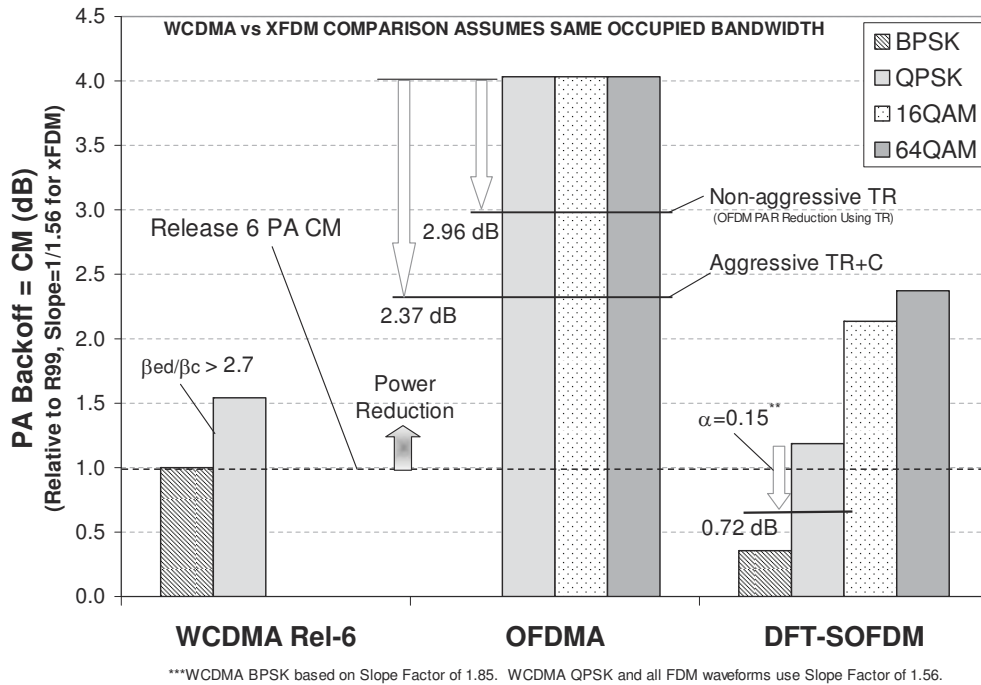
Figure 21.10: Cubic Metric (CM) for different waveforms.
