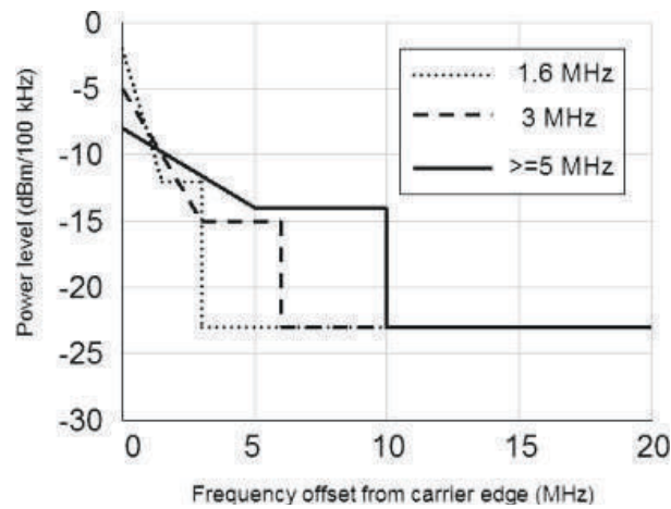
Figure 21.7: Spectrum emission mask for eNodeB transmitter.
