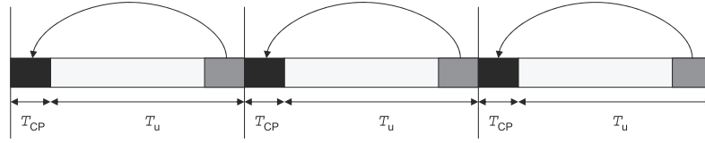
Figure 5.5: OFDM Cyclic Prefix (CP) insertion.
