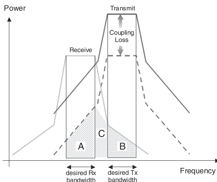
Figure 23.2: Frequency-domain interference between transmitter and receiver.
