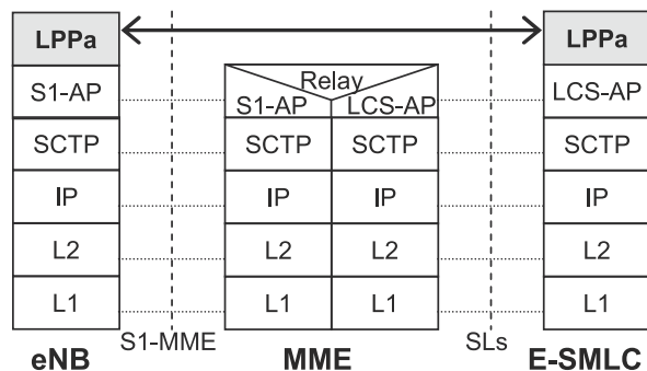
Figure 19.10: The LPPa protocol stack between the E-SMLC and the eNodeB.
