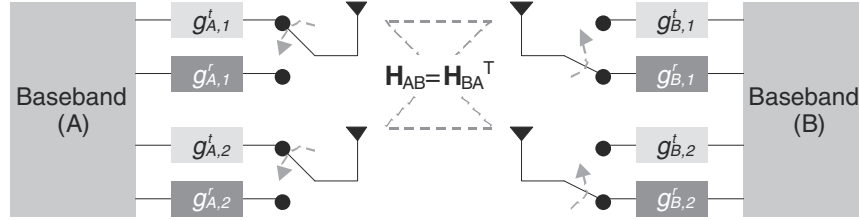
Figure 23.16: Transceiver elements in a reciprocal channel.
