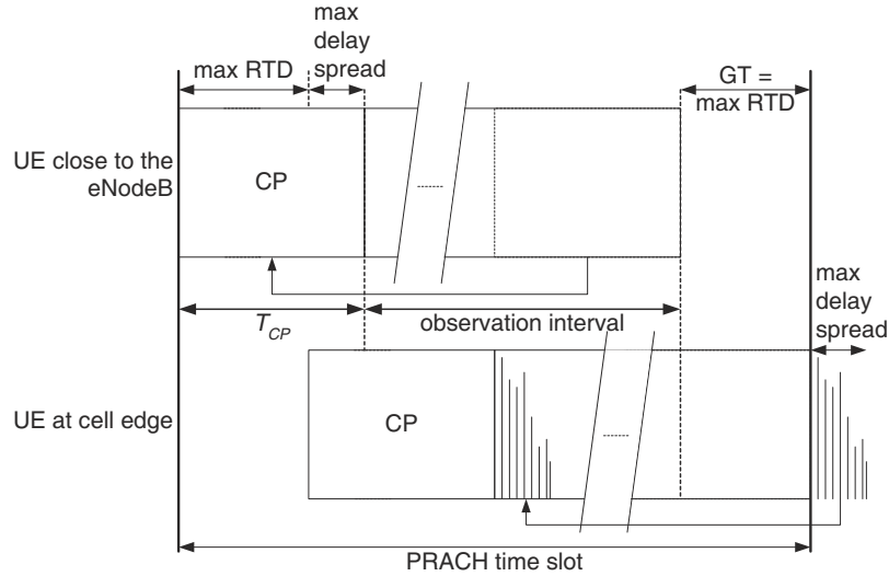
Figure 17.8: PRACH CP/GT dimensioning for formats 0 and 2.
