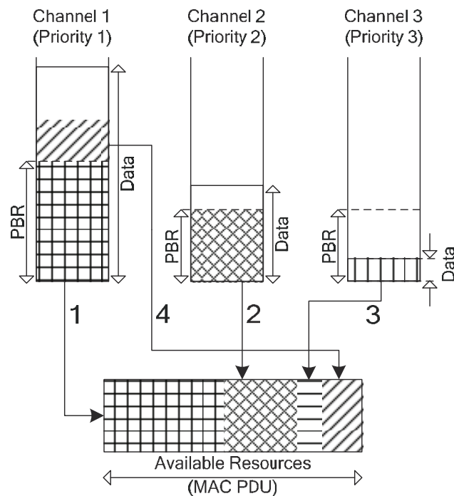
Figure 4.20: Example of MAC multiplexing.
