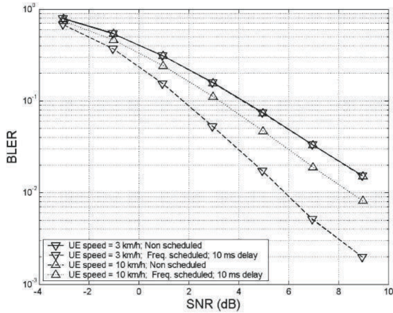
Figure 17.31: BLER performance of post-preamble scheduled data.
