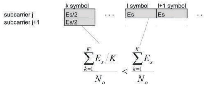
Figure 16.5: The link budget of a two-slot narrowband transmission exceeds that of a one-slot wider-band transmission, given equal coding gain.
