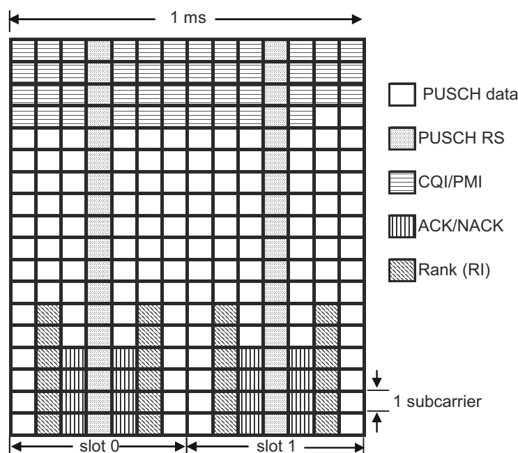
Figure 16.15: Multiplexing of control signalling with UL-SCH data.
