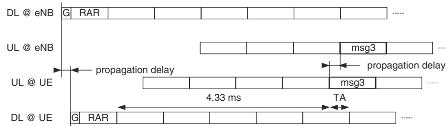
Figure 17.3: Timing of the message 3 transmission.
