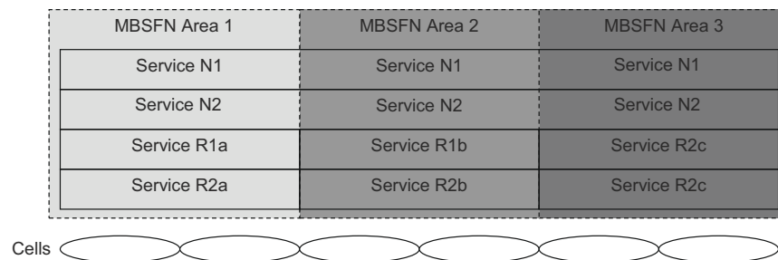
Figure 13.7: Example scenario without overlapping MBSFN areas.
