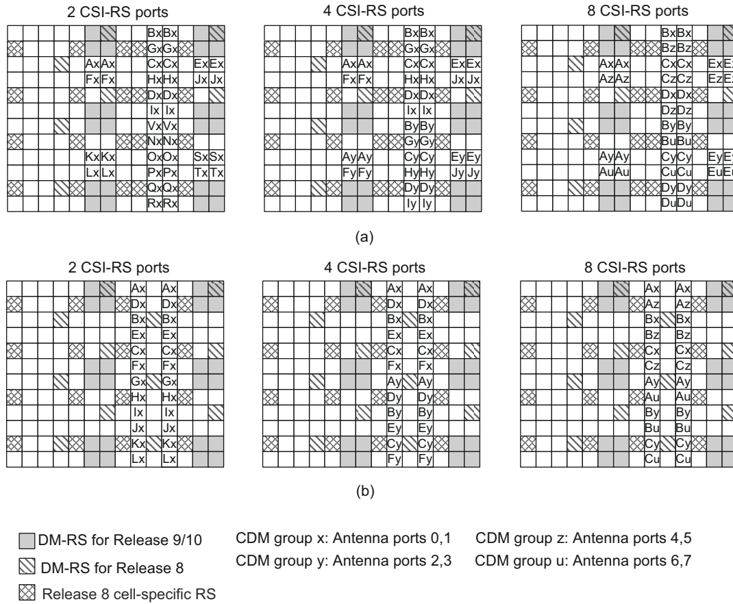
Figure 29.4: CSI-RS patterns for LTE-Advanced.
