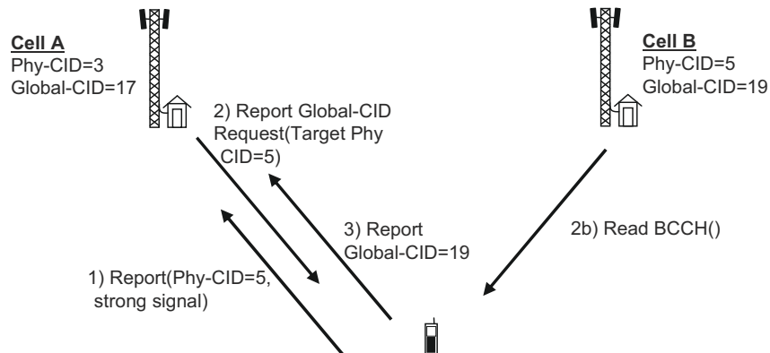
Figure 25.1: The intra-LTE ANR Function. Reproduced by permission of © 3GPP.
