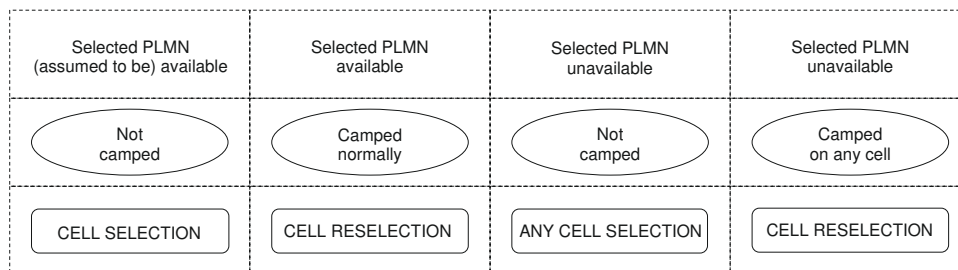
Figure 3.11: Idle mode states and procedures.
