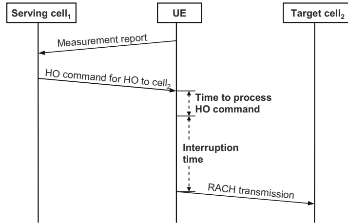
Figure 22.6: Handover to a known target cell.
