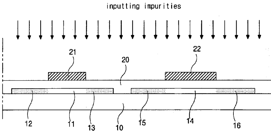
FIG. 3B (RELATED ART)
