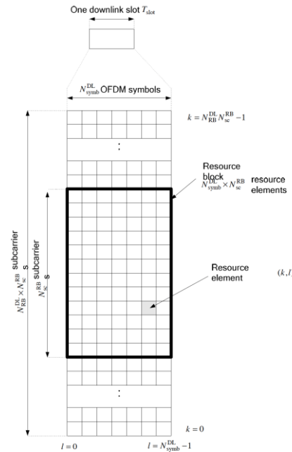
Figure 6.2.2-1: Downlink resource grid.
