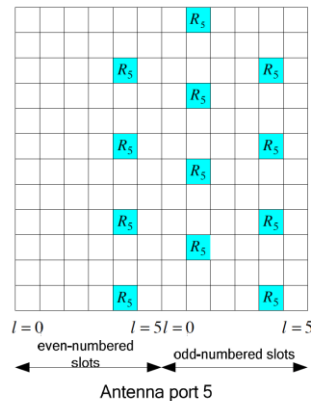
Figure 6.10.3.2-2: Mapping of UE-specific reference signals, antenna port 5 (extended cyclic prefix).
