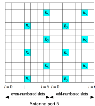
Figure 6.10.3.2-1: Mapping of UE-specific reference signals, antenna port 5 (normal cyclic prefix).
