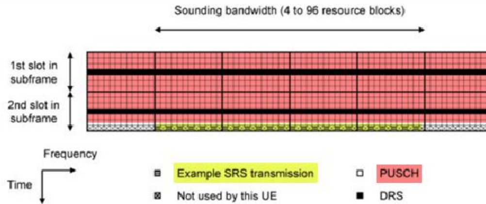
Figure 8.11 Example resource element mapping for the sounding reference signal, using a normal cyclic prefix.
