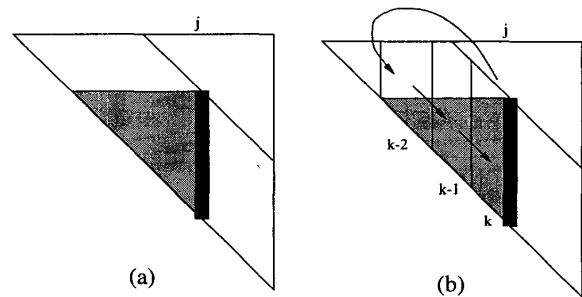
Figure 12. (a) Working set for the j^{th} column (b) Working set decomposition
