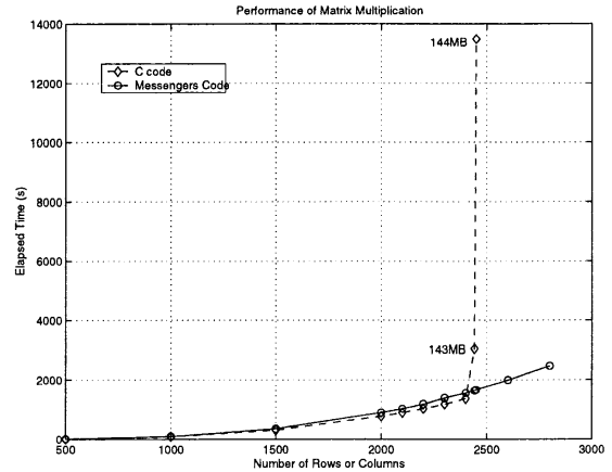
Figure 5. Performance of matrix multiplication
