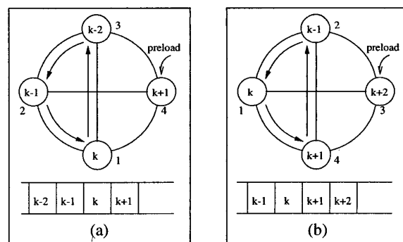
Figure 13. Logical network for Crout factorization. (a) currently computing piece k . (b) currently computing piece k + 1 .
