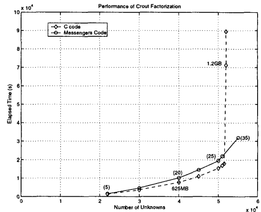
Figure 15. Performance of Crout factorization
