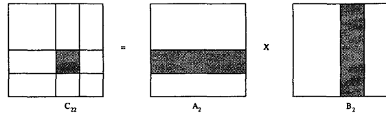
Figure 2. Matrix decomposition
