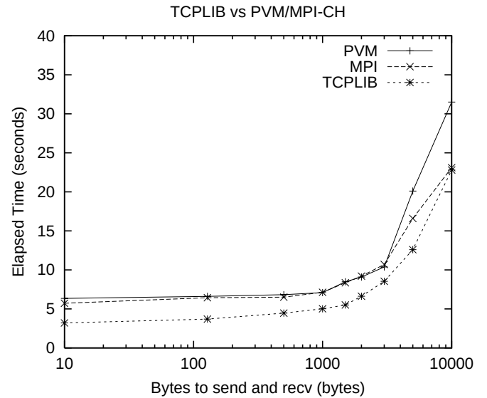
Figure 4. Performance of inter-daemon communication module
