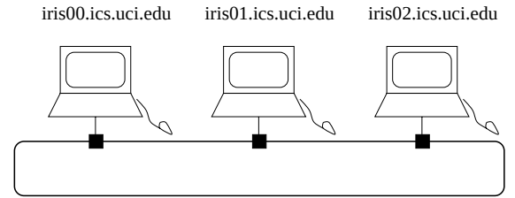
Figure 1. Computational network
