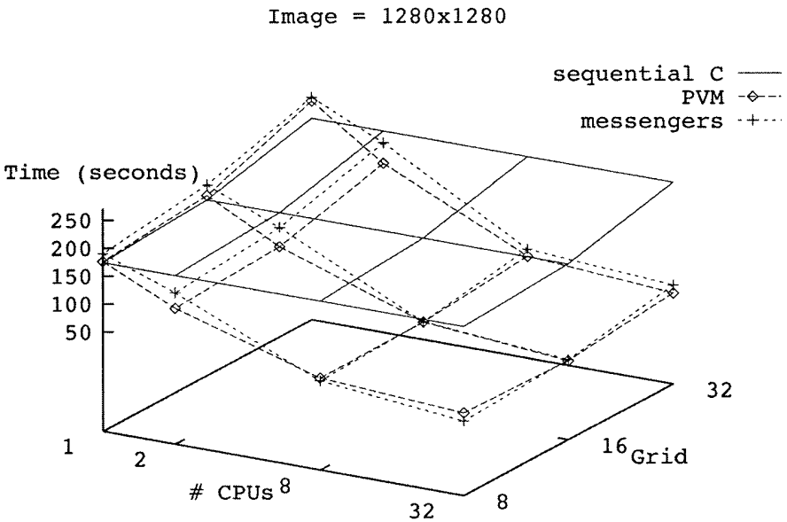
FIG. 6. Mandelbrot set computation with image size = 1280 × 1280.
