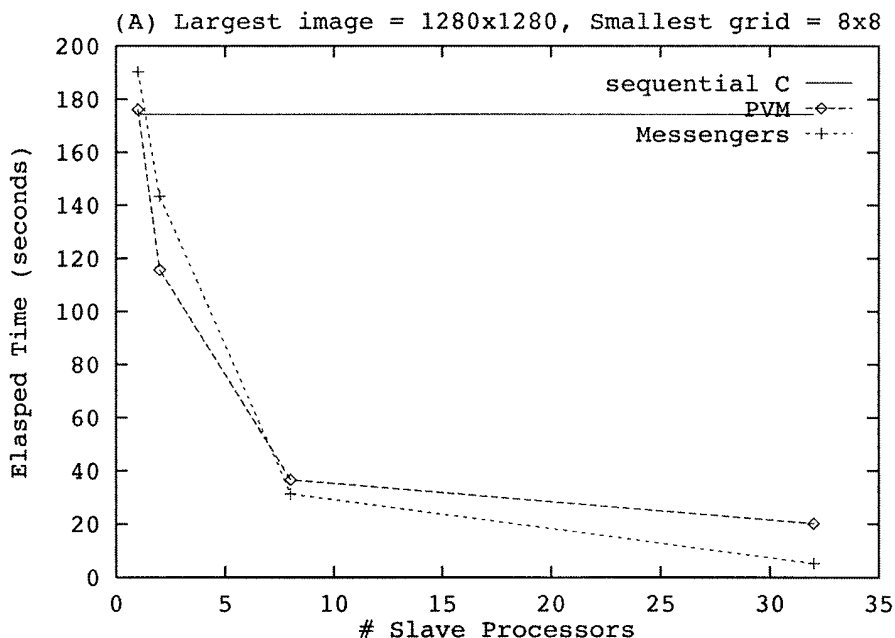
FIG. 7. The best case of Mandelbrot set generation.
