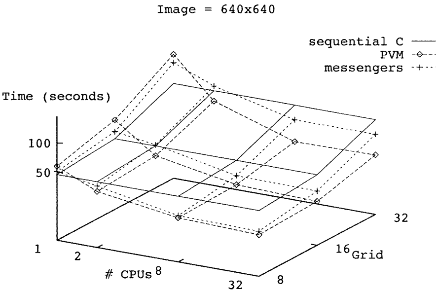
FIG. 5. Mandelbrot set computation with image size = 640 × 640.
