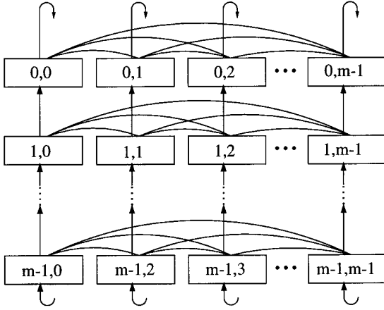
FIG. 10. Logical network for matrix multiplication.
