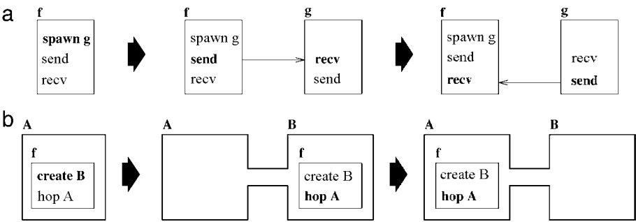
FIG. 1. (a) Task creation and message-passing. (b) Logical node creation and navigation.
