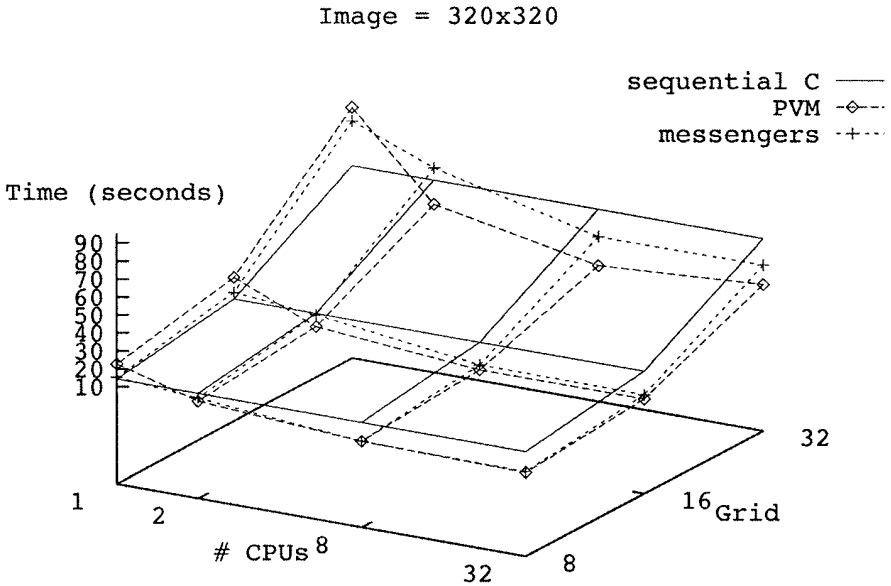
FIG. 4. Mandelbrot set computation with image size = 320 \times 320 .
