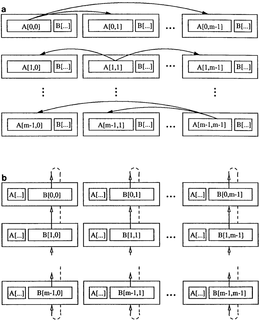
FIG. 8. (a) Distribution of A; (b) rotation of B.
