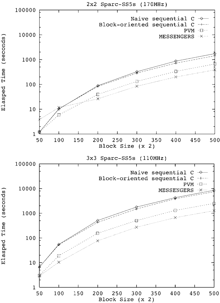
FIG. 12. Matrix multiplication results.
