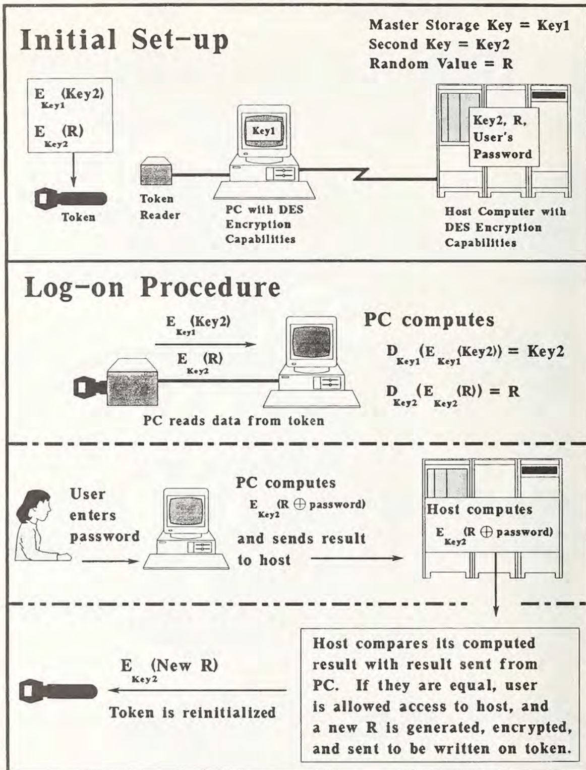
Figure 10. Access Control System for Cryptographic Workstations
