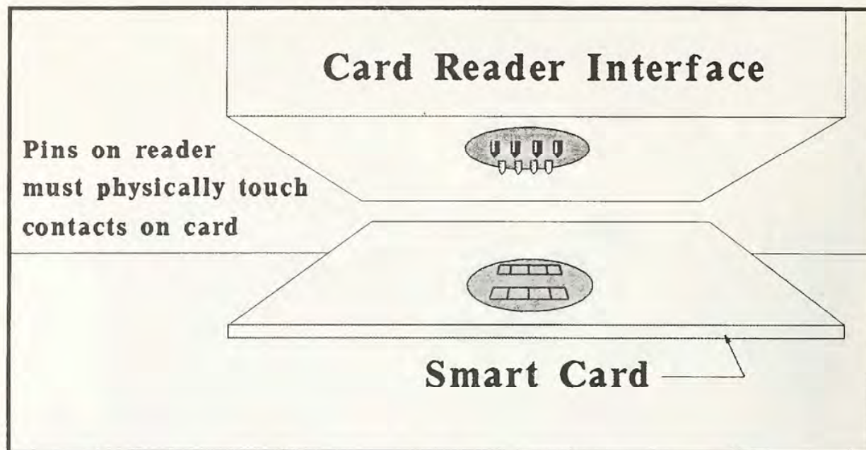
Figure 4. Contact-Type Smart Card Interface
