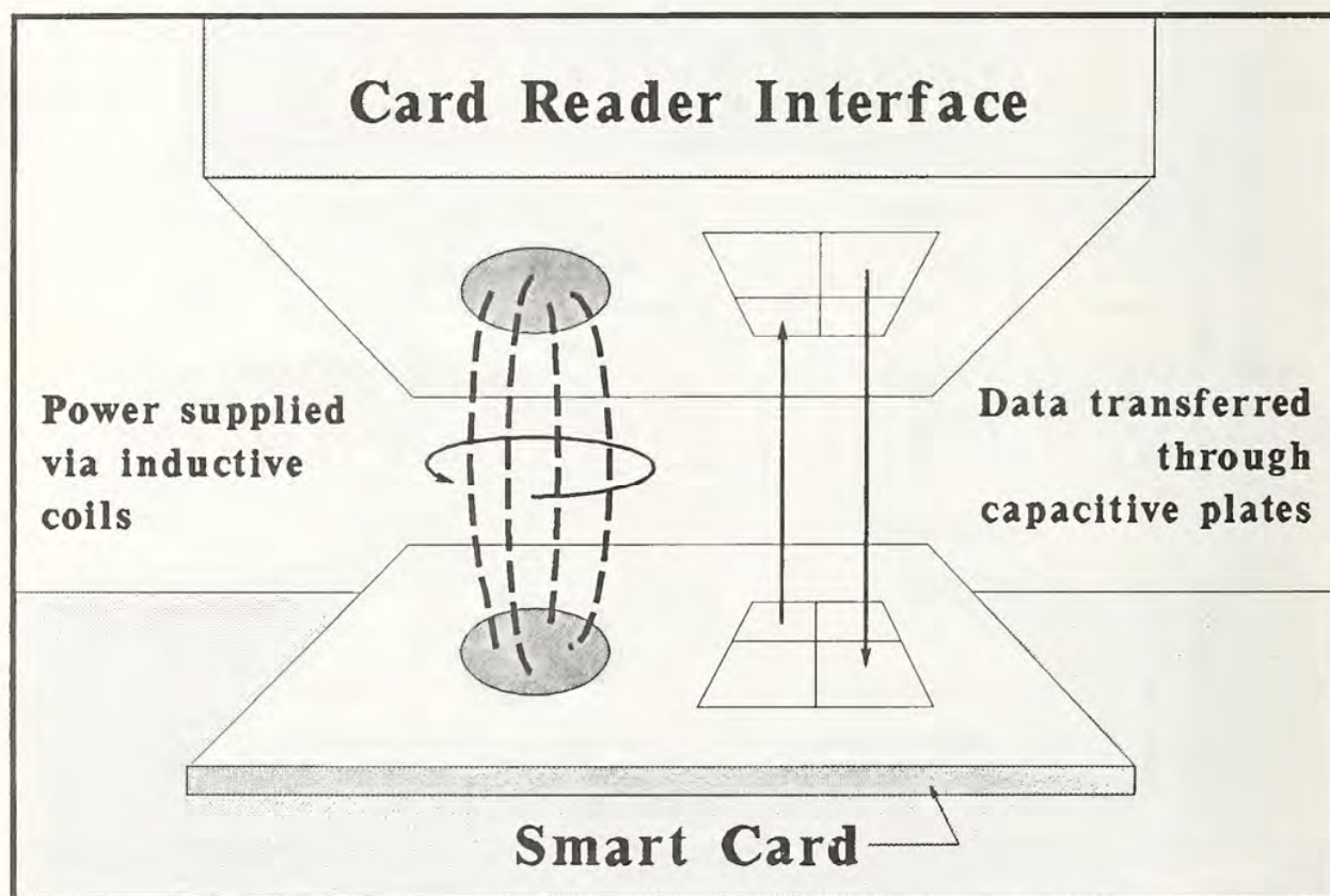
Figure 5. Non-Contact-Type Smart Card Interface
