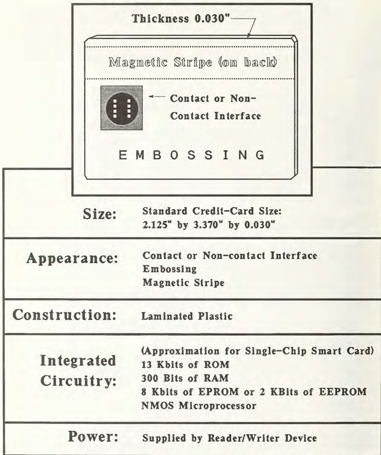
Figure 13. Current Smart Card Characteristics
