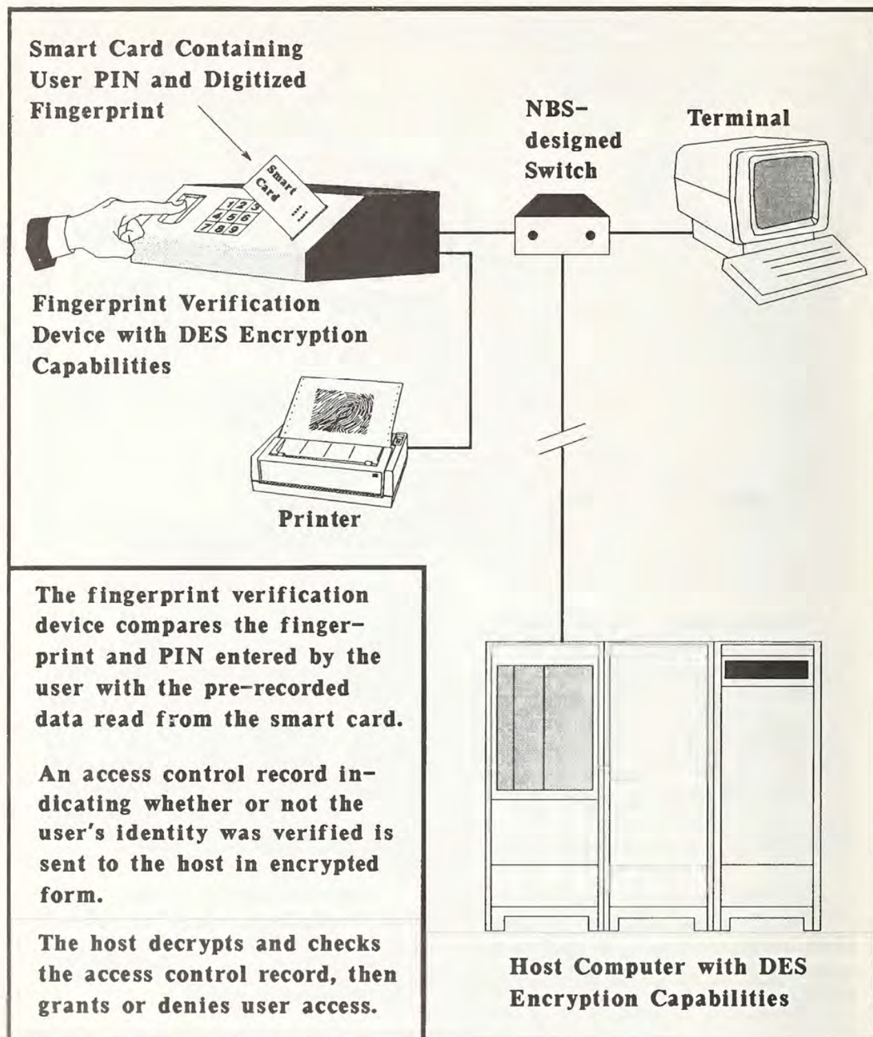
Figure 11. Biometric Smart Card Access Control System
