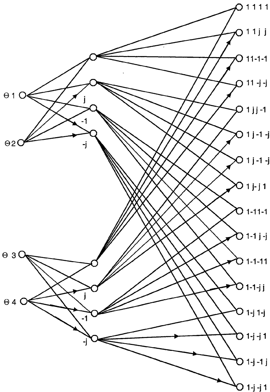
PSK Fast Hadamard Transform
