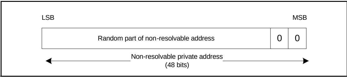
Figure 10.5: Format of non-resolvable private address
