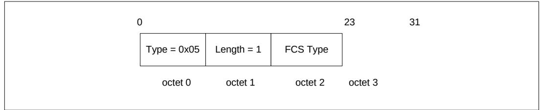
Figure 5.6: FCS option format
