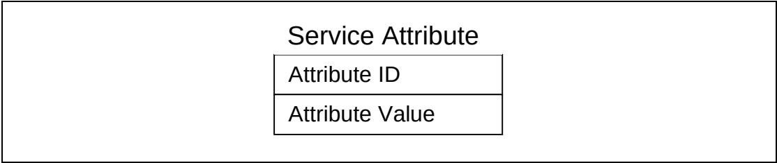
Figure 2.4: Service Attribute
