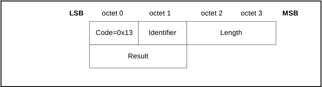
Figure 4.23: Connection Parameters Update Response packet
