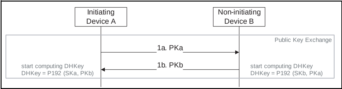
Figure 7.2: Public Key Exchange Details
