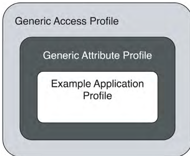
Figure 1.1: Profile dependencies
