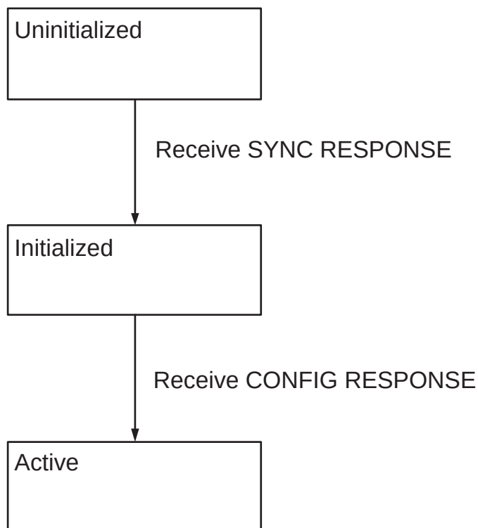
Figure 8.1: Link Establishment State Diagram
