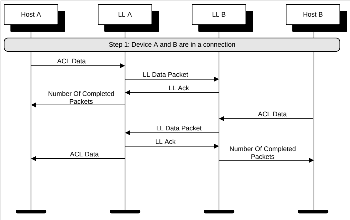
Figure 6.1: Sending Data
