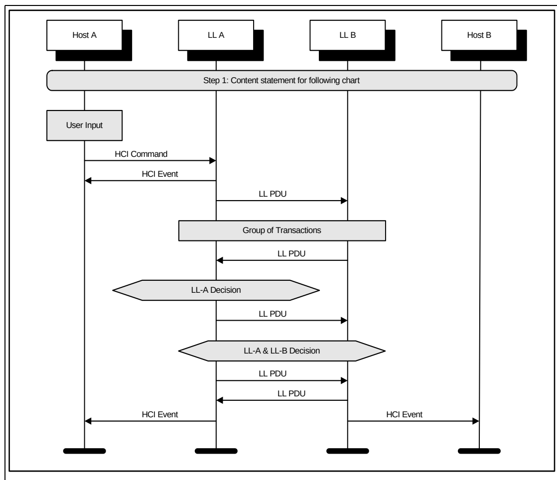
Figure 1.1: Example MSC
