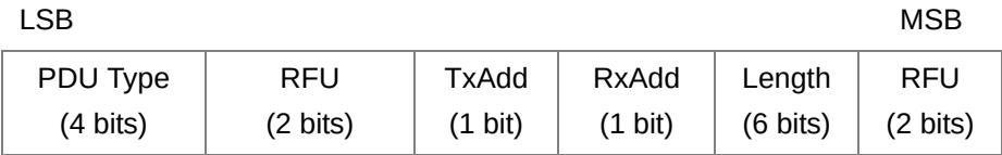
Figure 2.3: Advertising channel PDU Header
