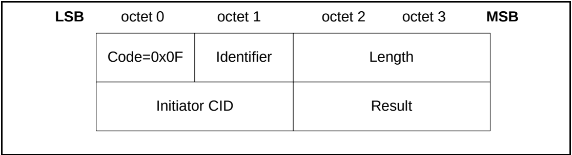
Figure 4.19: Move Channel Response Packet
