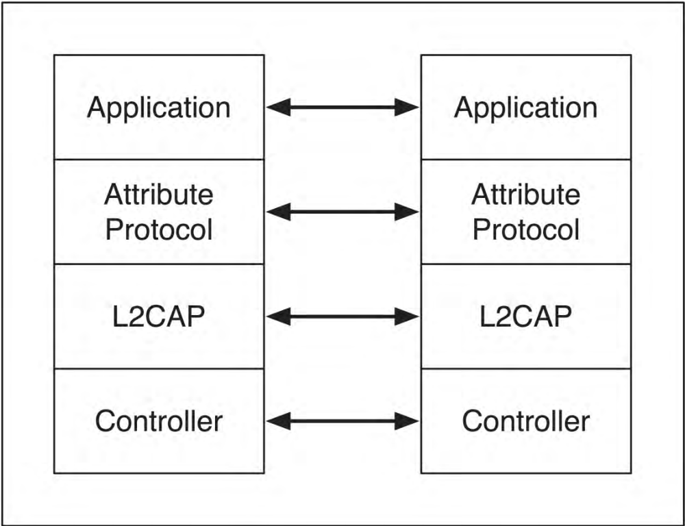
Figure 2.1: Protocol model
