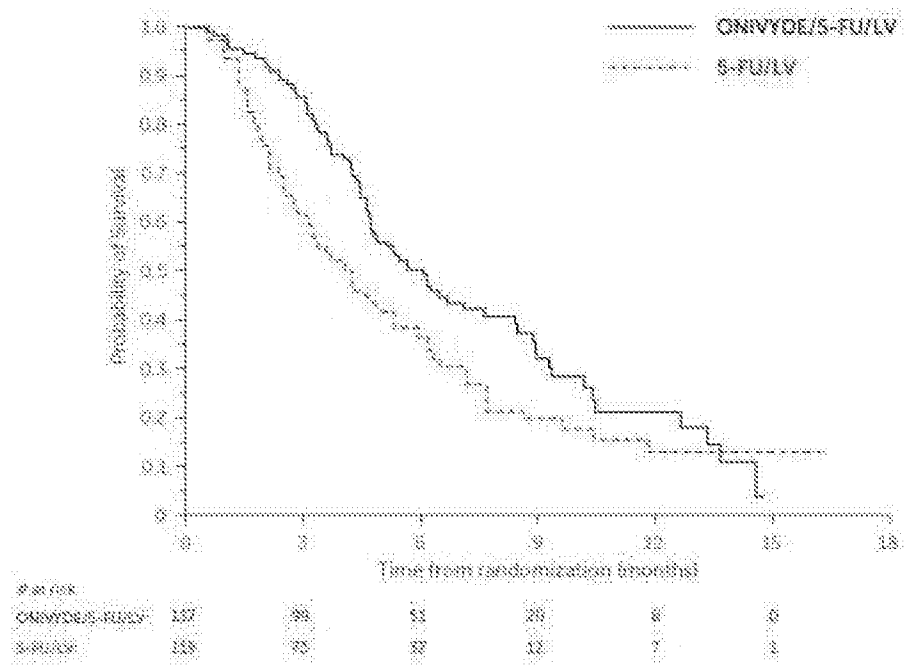
Figure 1: Overall Survival
