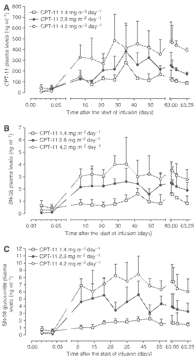
Figure 2 Plasma levels of irinotecan (CPT-11) (A), SN-38 (B) and SN-38 glucuronide (C) in 20 mCRC patients receiving an iv. continuous infusion of CPT-11 at three different dose levels. Symbols and bars represent mean and s.d.
