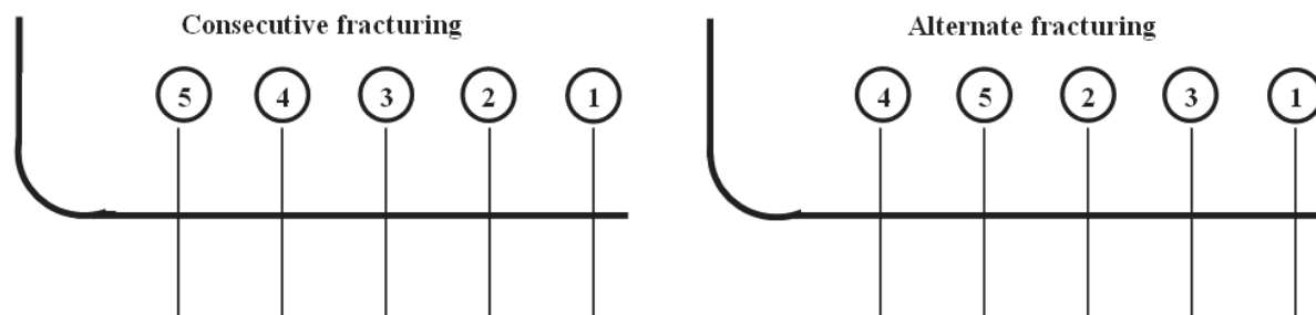
Figure 12 – Two fracturing sequences (a) consecutive (1-2-3-4-5) and (b) alternate (1-3-2-5-4)
