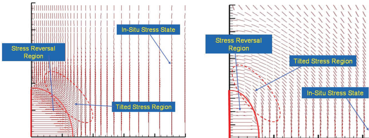
Figure 4 – Comparison of stress reorientation due to mechanical and poroelastic effects (direction of maximum horizontal stress)
