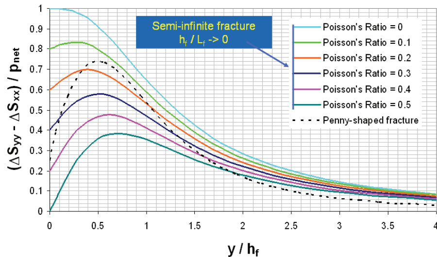
Figure 7 – Effect of Poisson's ratio in the pay zone on the generated stress contrast for semi-infinite and penny-shaped fractures
