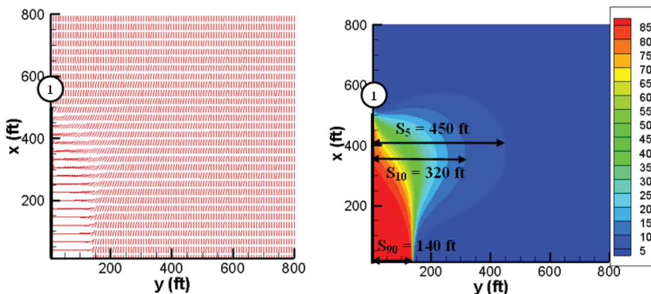
Figure 11 – Direction of maximum horizontal stress and angle of stress reorientation for a single transverse fracture
