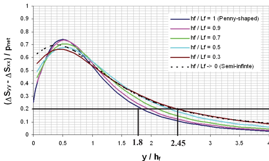
Figure 6 – Effect of fracture aspect ratio ( h_f/L_f ) on the generated stress contrast
