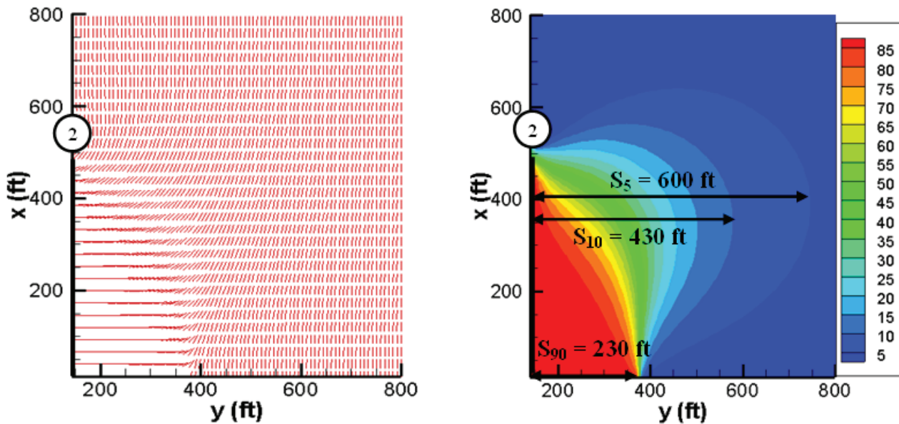
Figure 15 – Direction of maximum horizontal stress and angle of stress reorientation after placing 2 nd fracture at isotropic point (least favorable case)
