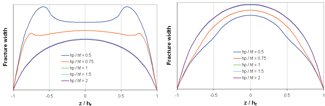
Figure 9 – Effect of fracture penetration on fracture width for a penny-shaped fracture ( h_f/L_f = 1 ) and (a) E_b/E_p = 0.6 , (b) E_b/E_p = 3
