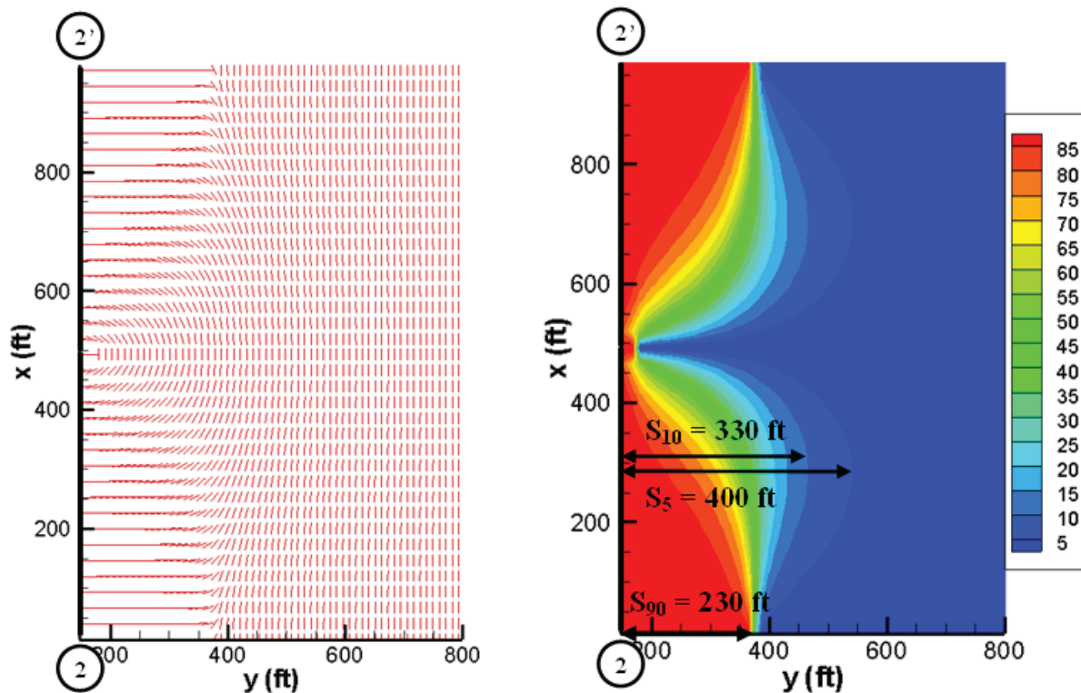
Figure 20 – Direction of maximum horizontal stress and angle of stress reorientation after placing 2 nd fractures at isotropic point (zipper-fracs)
