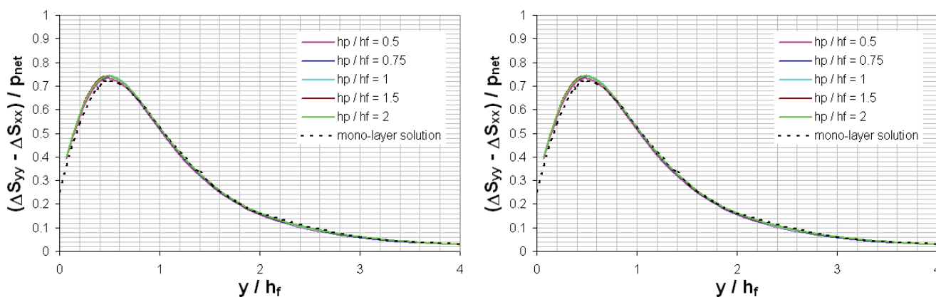
Figure 10 – Effect of fracture penetration on the generated stress contrast for a penny-shaped fracture ( h_f/L_f = 1 ) and (a) \nu_b/\nu_p = 2 , (b) \nu_b/\nu_p = 0.67
