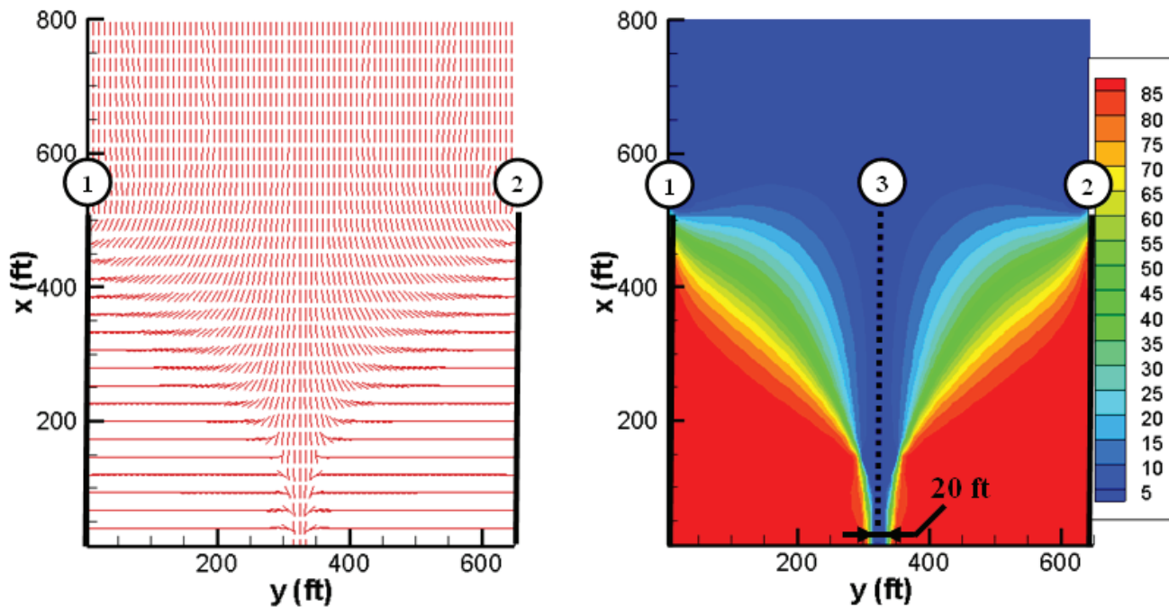
Figure 17 – Direction of maximum horizontal stress and angle of stress reorientation for a fracture spacing of 650 ft
