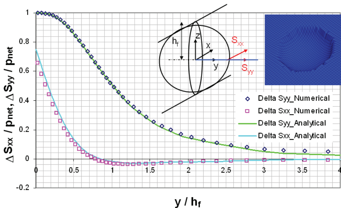
Figure 3 – Comparisons of analytical (Sneddon et al. , 1946) and numerical stress distributions for a penny-shaped fracture ( \nu = 0.2 )
