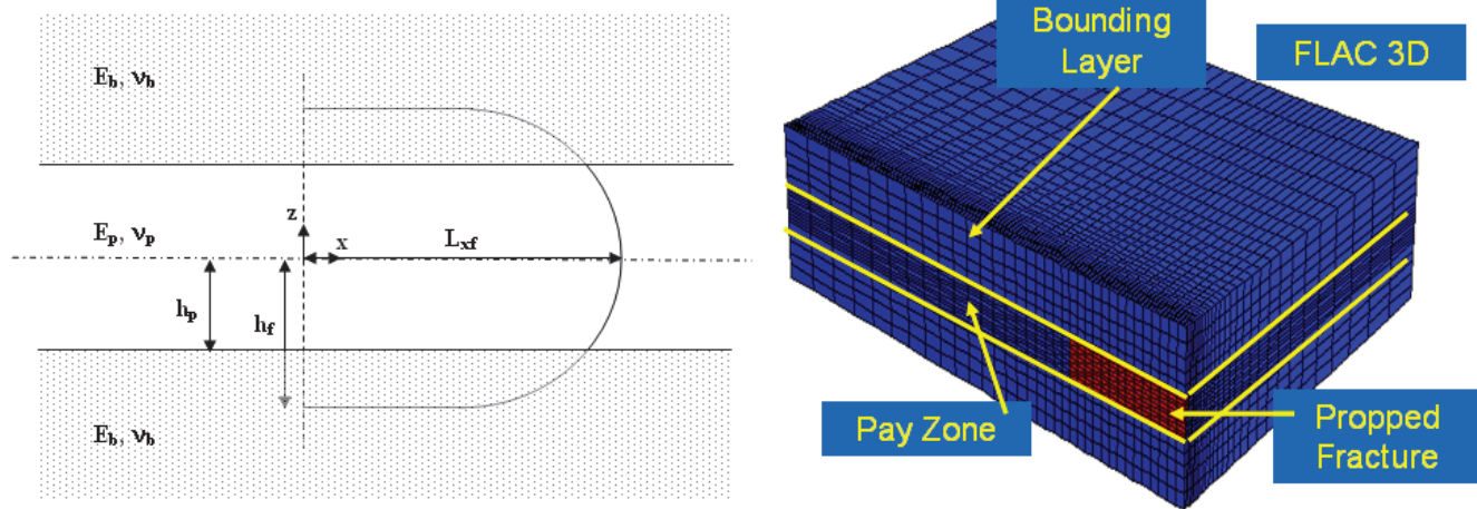
Figure 1 – Three-dimensional model of a transverse fracture
