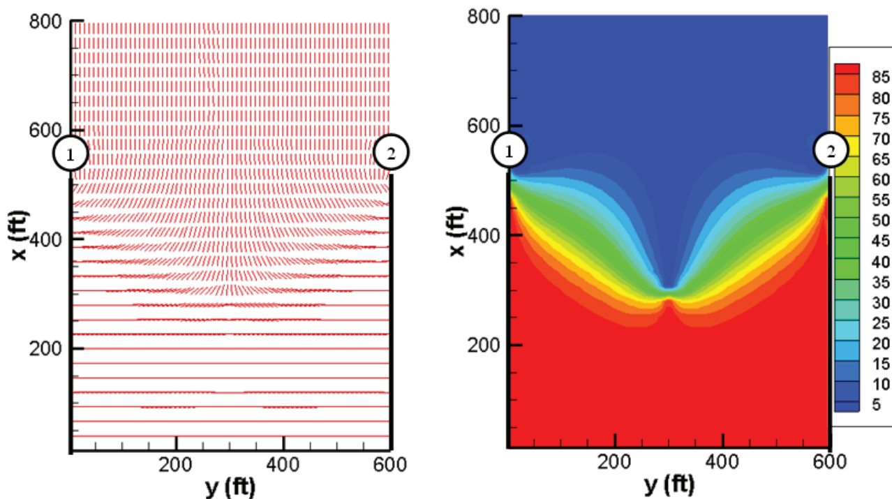
Figure 16 – Direction of maximum horizontal stress and angle of stress reorientation for a fracture spacing of 600 ft
