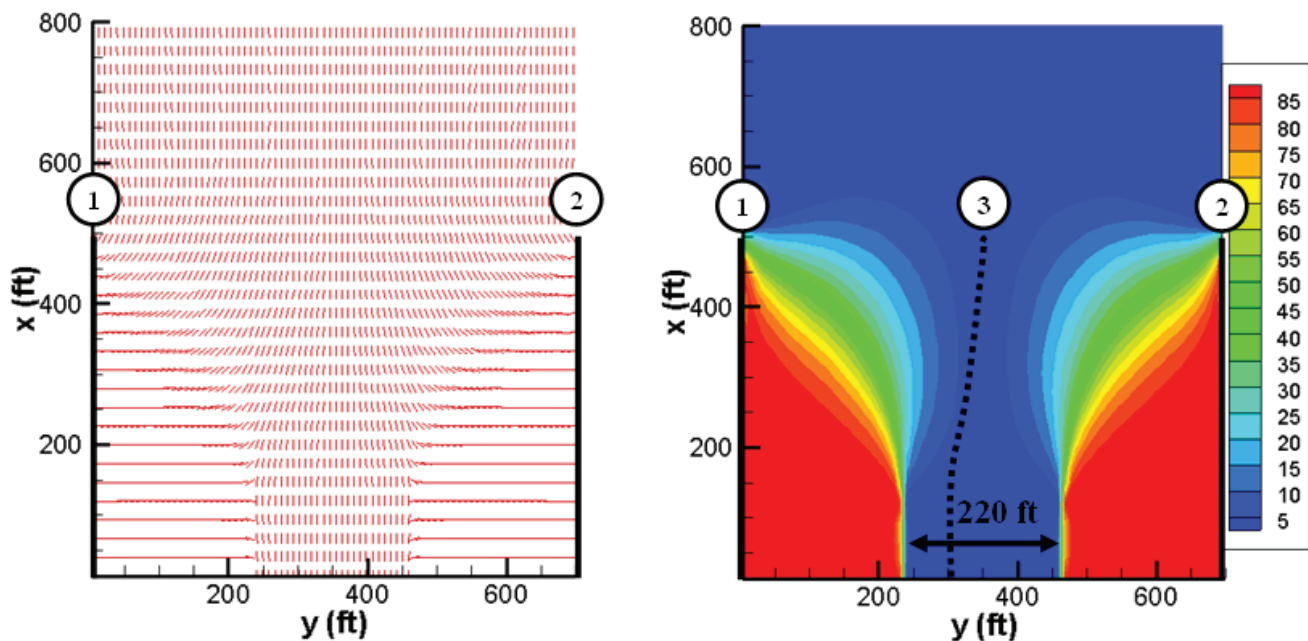
Figure 18 – Direction of maximum horizontal stress and angle of stress reorientation for a fracture spacing of 700 ft
