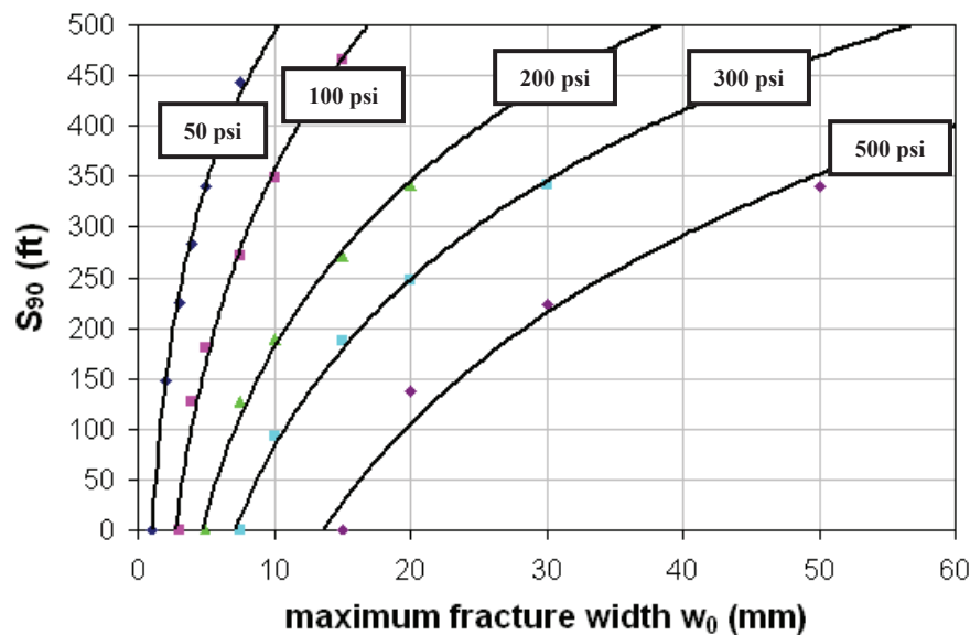
Figure 13 – Minimum fracture spacing S_{90} versus maximum fracture width for different values of the horizontal stress contrast
