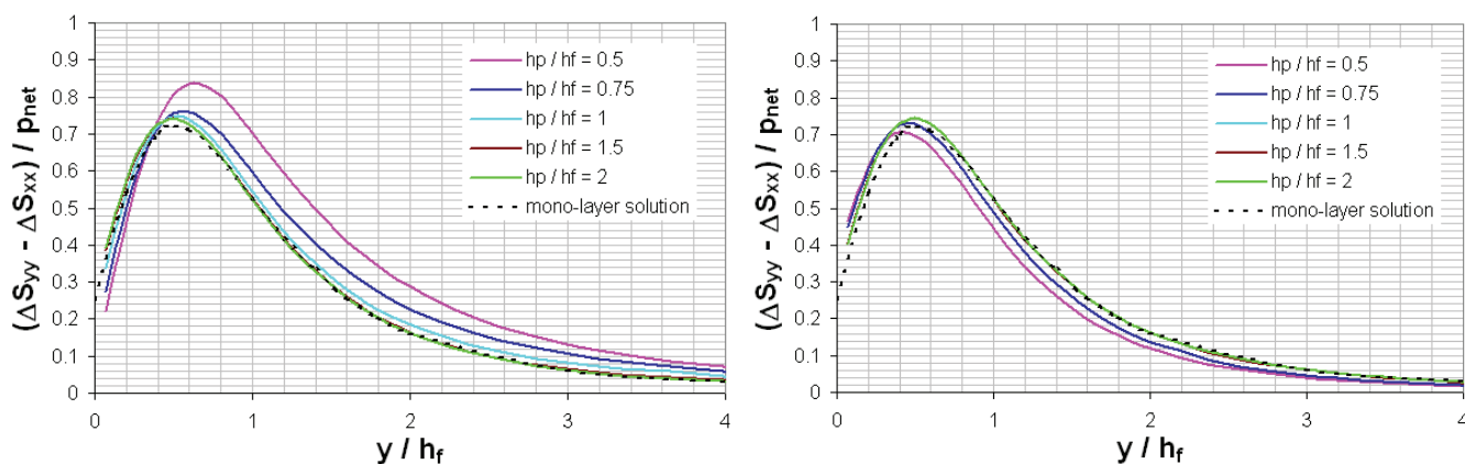
Figure 8 – Effect of fracture penetration on the generated stress contrast for a penny-shaped fracture ( h_f/L_f = 1 ) and (a) E_b/E_p = 0.6 , (b) E_b/E_p = 3
