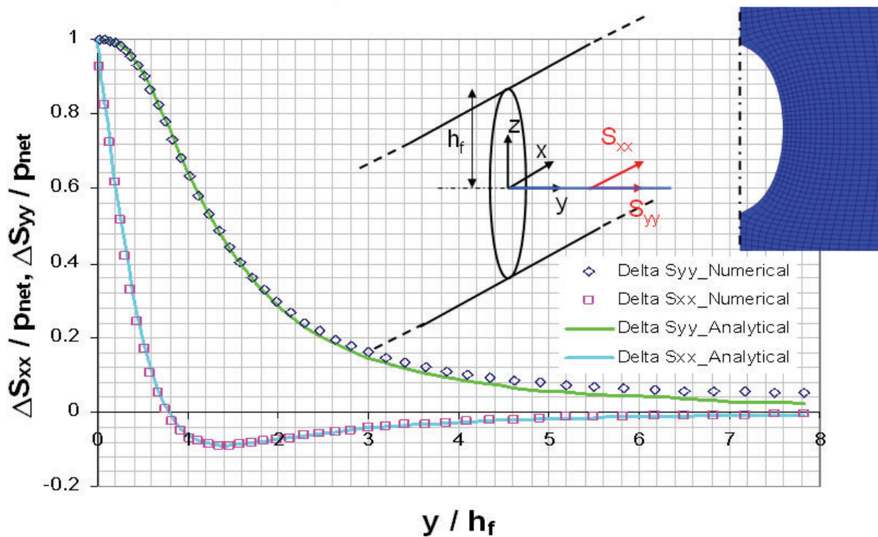
Figure 2 – Comparisons of analytical (Sneddon et al. , 1946) and numerical stress distributions for a semi-infinite fracture ( \nu = 0.2 )
