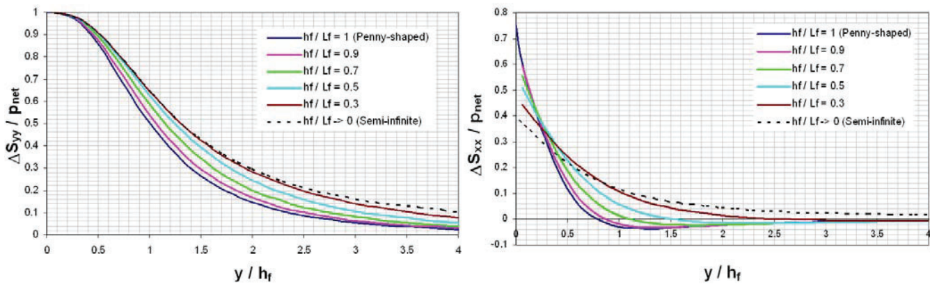
Figure 5 – Effect of fracture aspect ratio ( h_f/L_f ) on the stress perturbation
