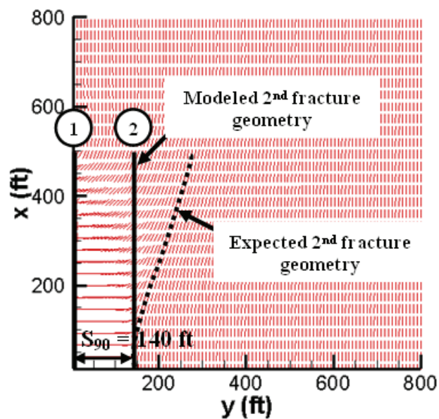
Figure 14 – Worst case scenario for stress reorientation ahead of the last fracture in the sequential fracturing of horizontal wells (2 nd fracture at isotropic point)
