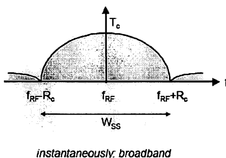
Figure 3. Message signal energy spread on bandwidth (DSSS)
