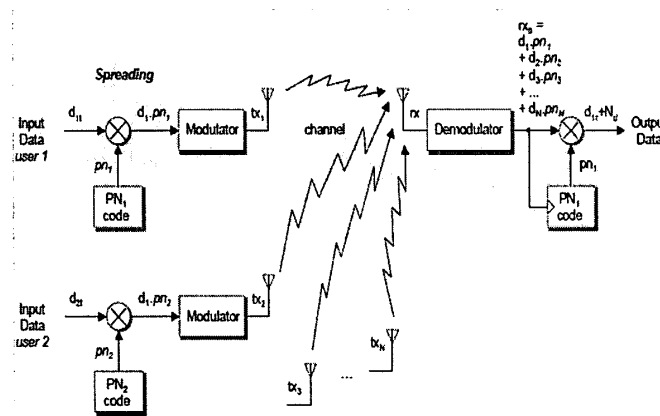
Figure 8. CDMA Network Concept
