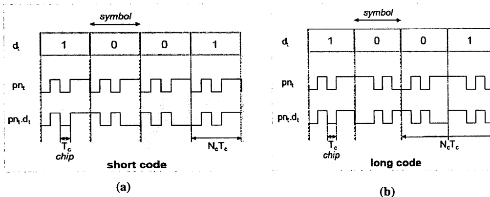
Figure 5. DSSS –a) Short-Code –b) Long-Code systems
