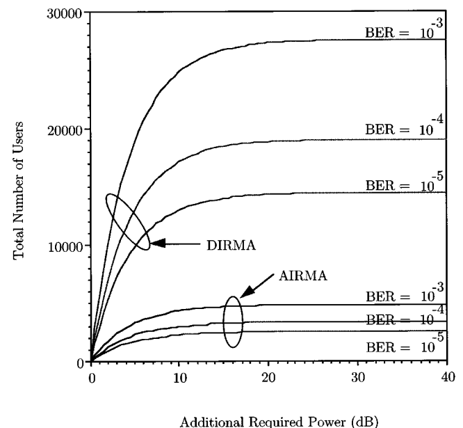
Fig. 6. Total number of users versus additional required power (decibels) for AIRMA and DIRMA receivers. This figure is plotted for three different performance levels with the data rate of 19.2 kbps.
