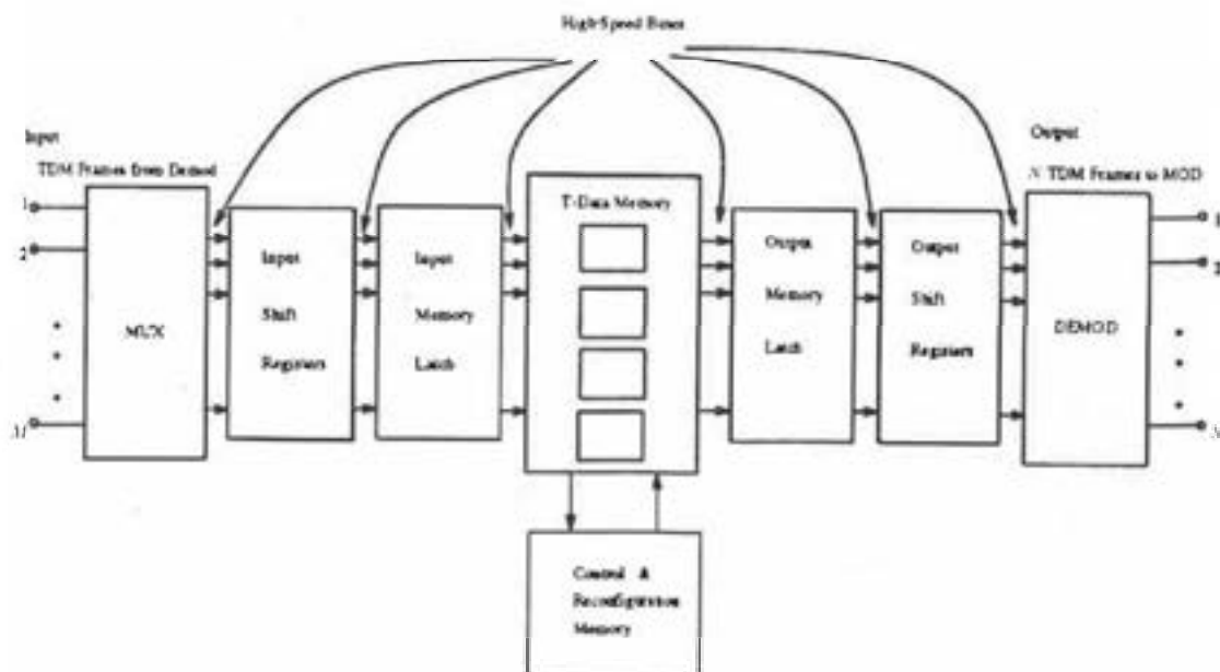
FIGURE 72.7 A baseband memory switch.
