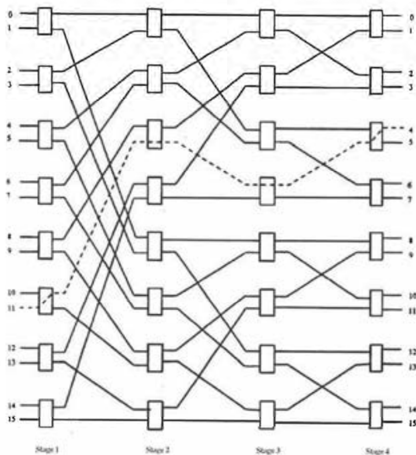
FIGURE 72.9(b) Banyan network with four stages and 16 input terminals. The dotted path corresponds to a packet header of 0100.
