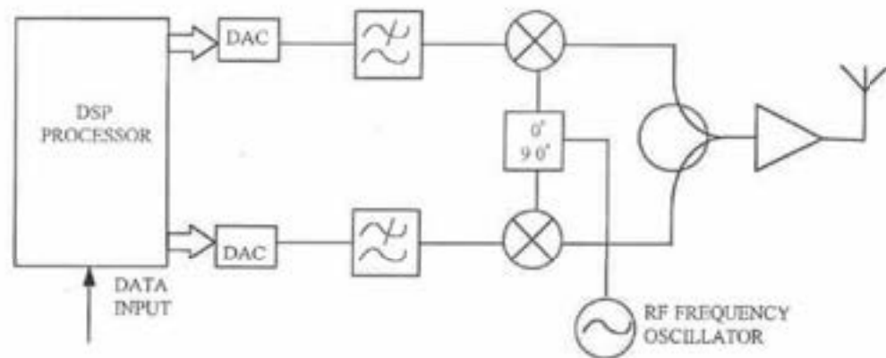
FIGURE 92.14 Transmit section.
