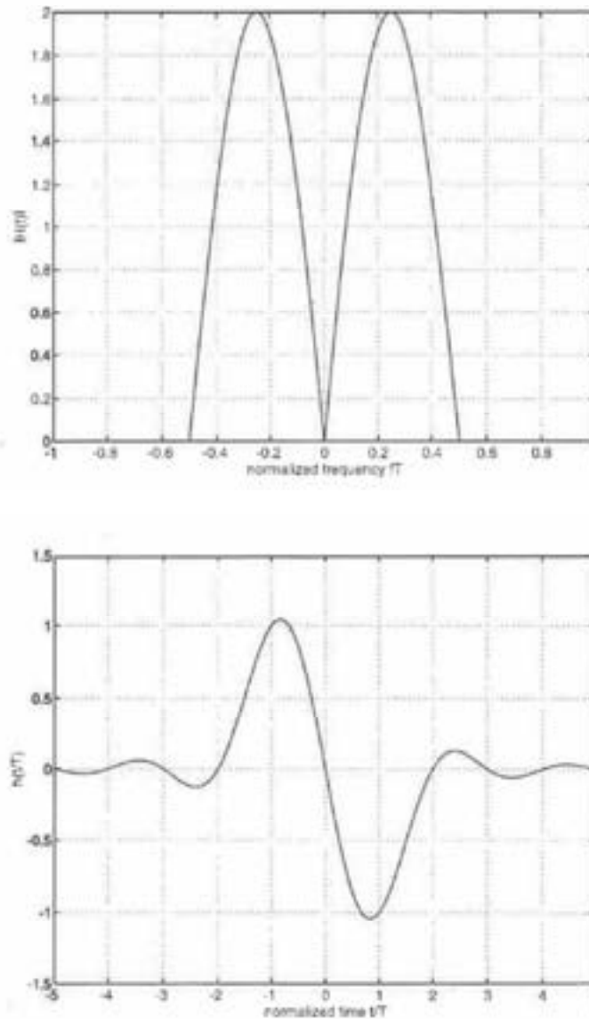
FIGURE 25.10 Modified duobinary frequency response and minimum bandwidth pulse.
