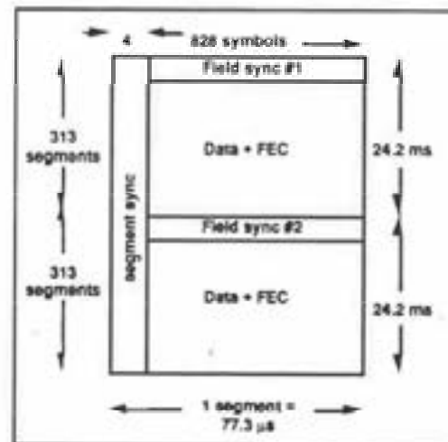
FIGURE 103.5 VSB data frame.
