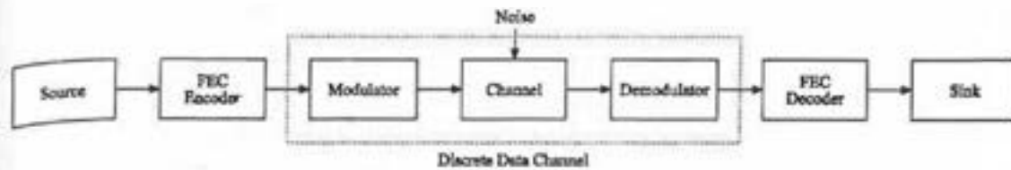
FIGURE 14.1 Block diagram of a digital communication system with forward error correction.
