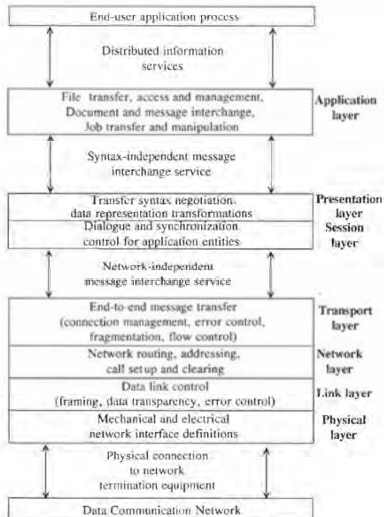
FIGURE 41.4 Protocol layer summary.
