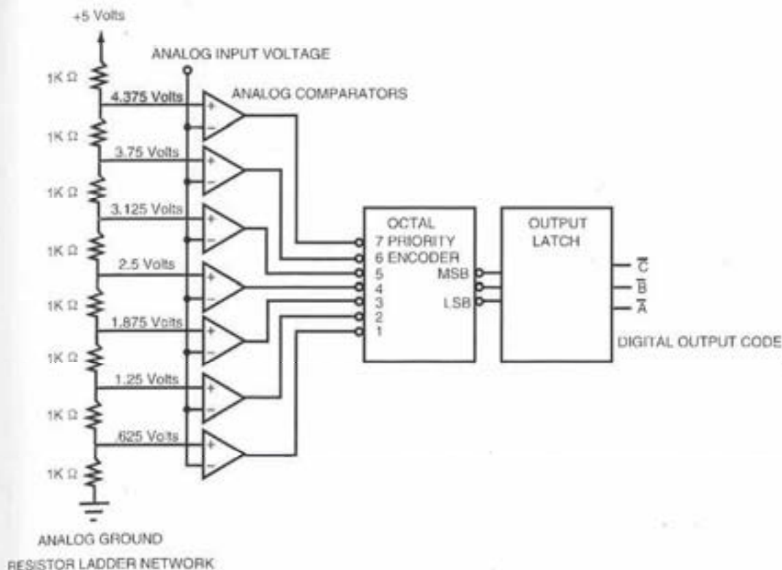
FIGURE 9.2 Flash A/D converter block diagram. (Source: Garrod, S. and Borns, R. Digital Logic: Analysis, Application, and Design , p. 928. Copyright ©1991 by Saunders College Publishing, Philadelphia, PA. Reprinted by permission of the publisher.)
