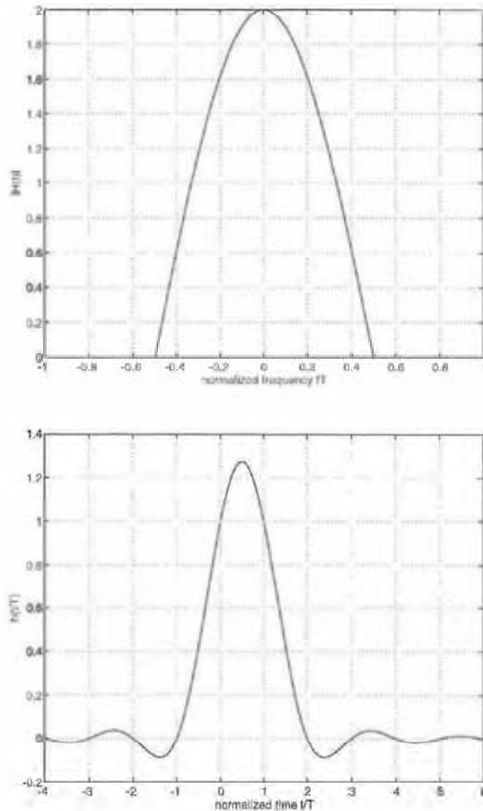
FIGURE 25.9 Duobinary frequency response and minimum bandwidth pulse.
