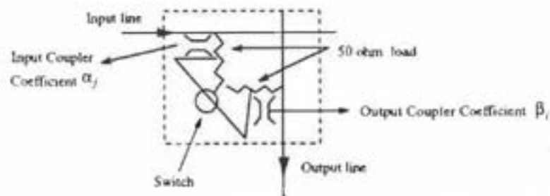
FIGURE 72.3(b) Switch module units; \alpha_j = coupling coefficient of j th output cross point on the same input line; \beta_i = coupling coefficient of i th cross point on the same output line.
