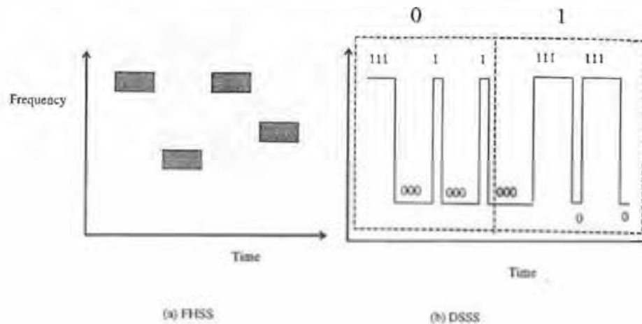
FIGURE 96.2 Spread spectrum.
