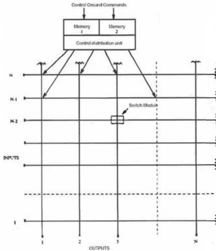
FIGURE 72.3(a) N \times N IF switch matrix using crossbar configuration.
