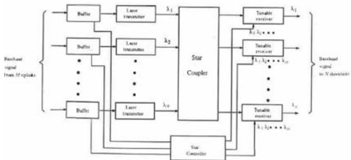
FIGURE 72.13 A WDM-based onboard baseband switch.
