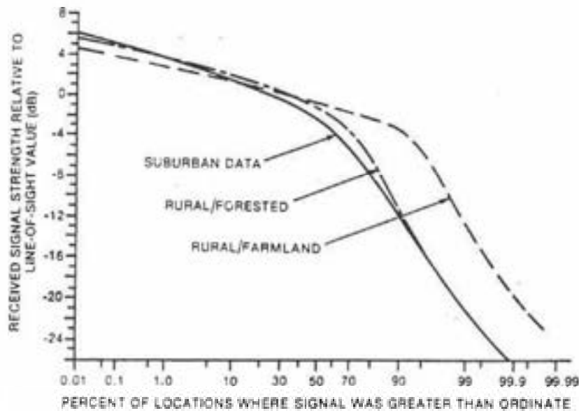
FIGURE 74.2 Distribution functions for data recorded near Ottawa, Canada, in June 1983. The measurements were made with an omnidirectional antenna at a frequency of 1542 MHz. The elevation angle (the angle between a plane parallel to the Earth's surface and the line-of-sight path to the satellite) was approximately 20^\circ . (Source: Butterworth, 1984.)
