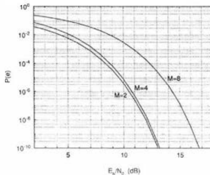
FIGURE 21.5 Symbol error probability of coherently demodulated PSK.
