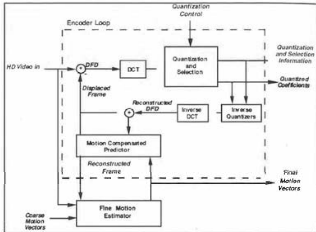
FIGURE 103.2 Video encoder loop.
