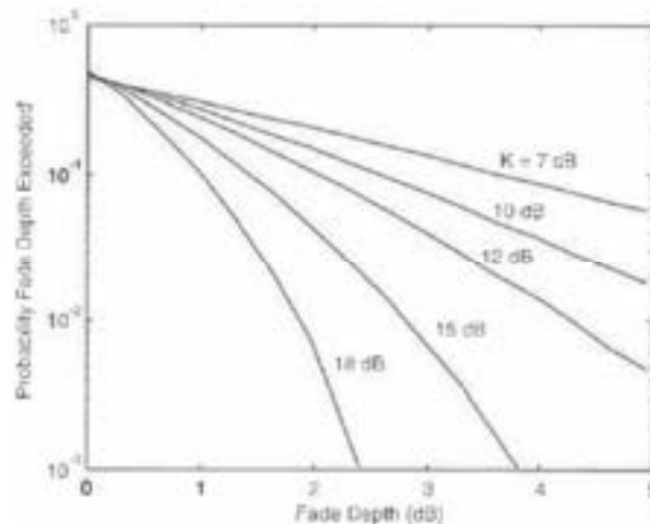
FIGURE 74.3 Cumulative fade distribution for the Rician channel as a function of K factor.
