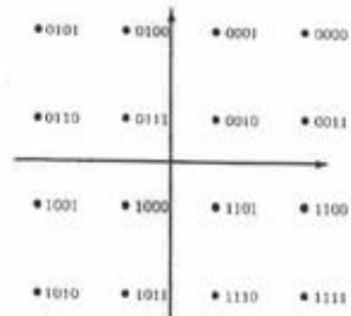
FIGURE 21.6 A 16-QAM constellation.
