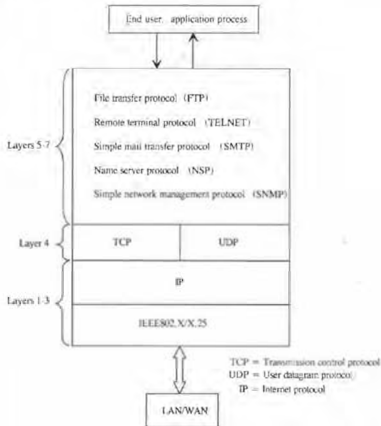
FIGURE 41.5 TCP/IP protocol suite.
