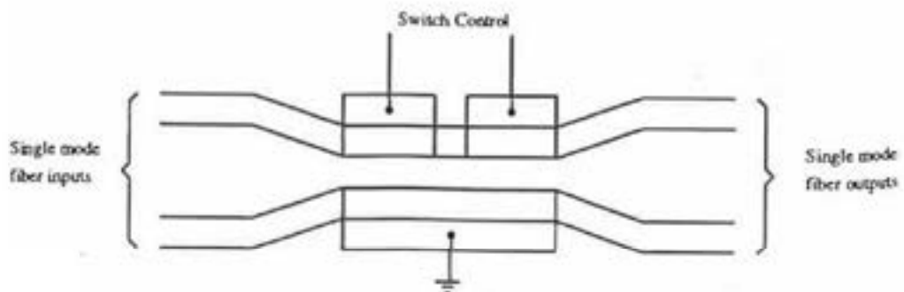
FIGURE 72.4(a) A 2 \times 2 all optical switch module using directional coupler.
