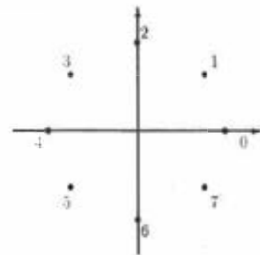
FIGURE 21.4 An 8-PSK constellation.
