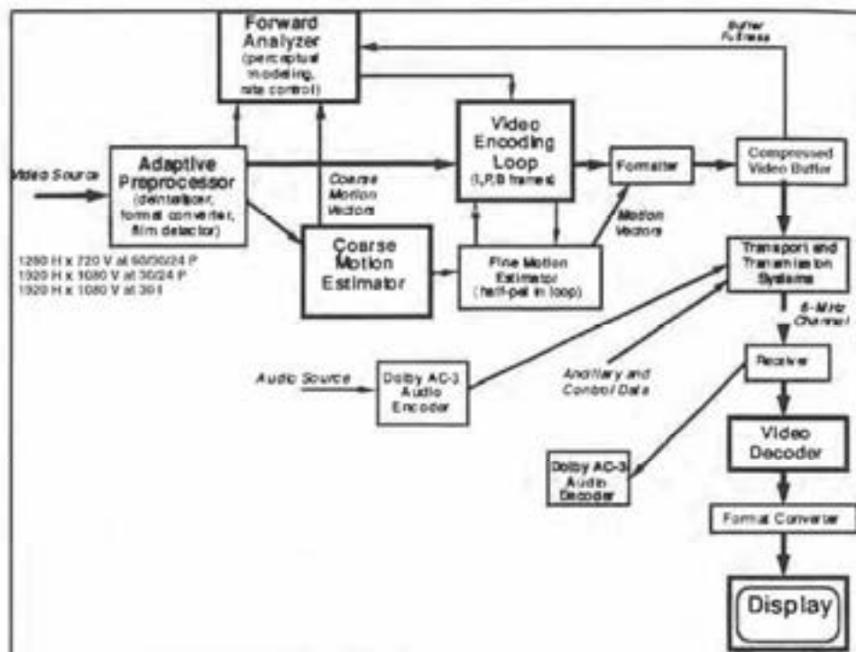
FIGURE 103.1 Grand Alliance system overview.
