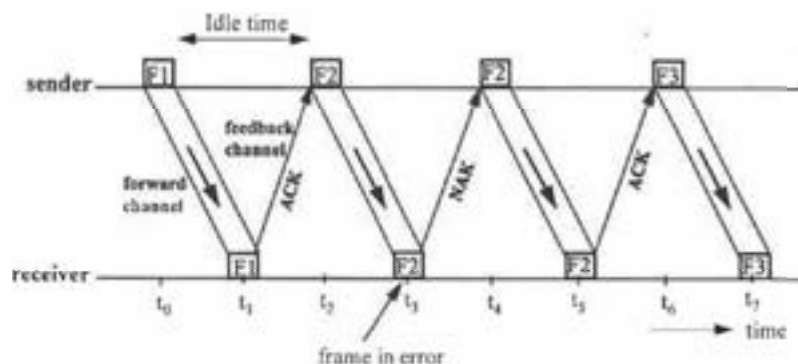
FIGURE 15.2 Stop-and-wait ARQ.
