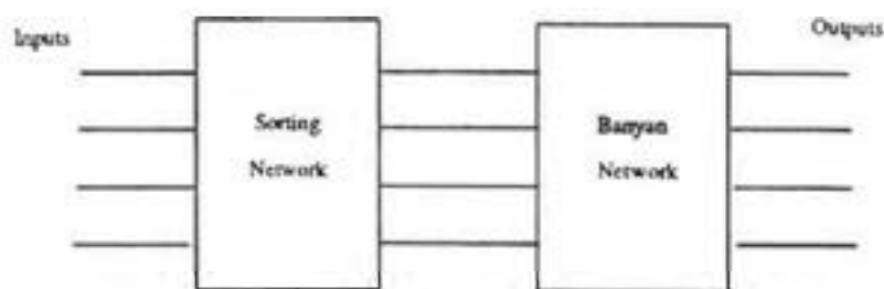
FIGURE 72.9(a) A sorter-Banyan baseband switch.
