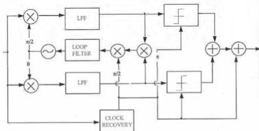
FIGURE 92.12 Costas Loop.
