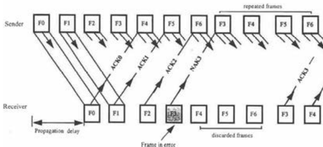
FIGURE 15.4 Go-back- N ARQ.
