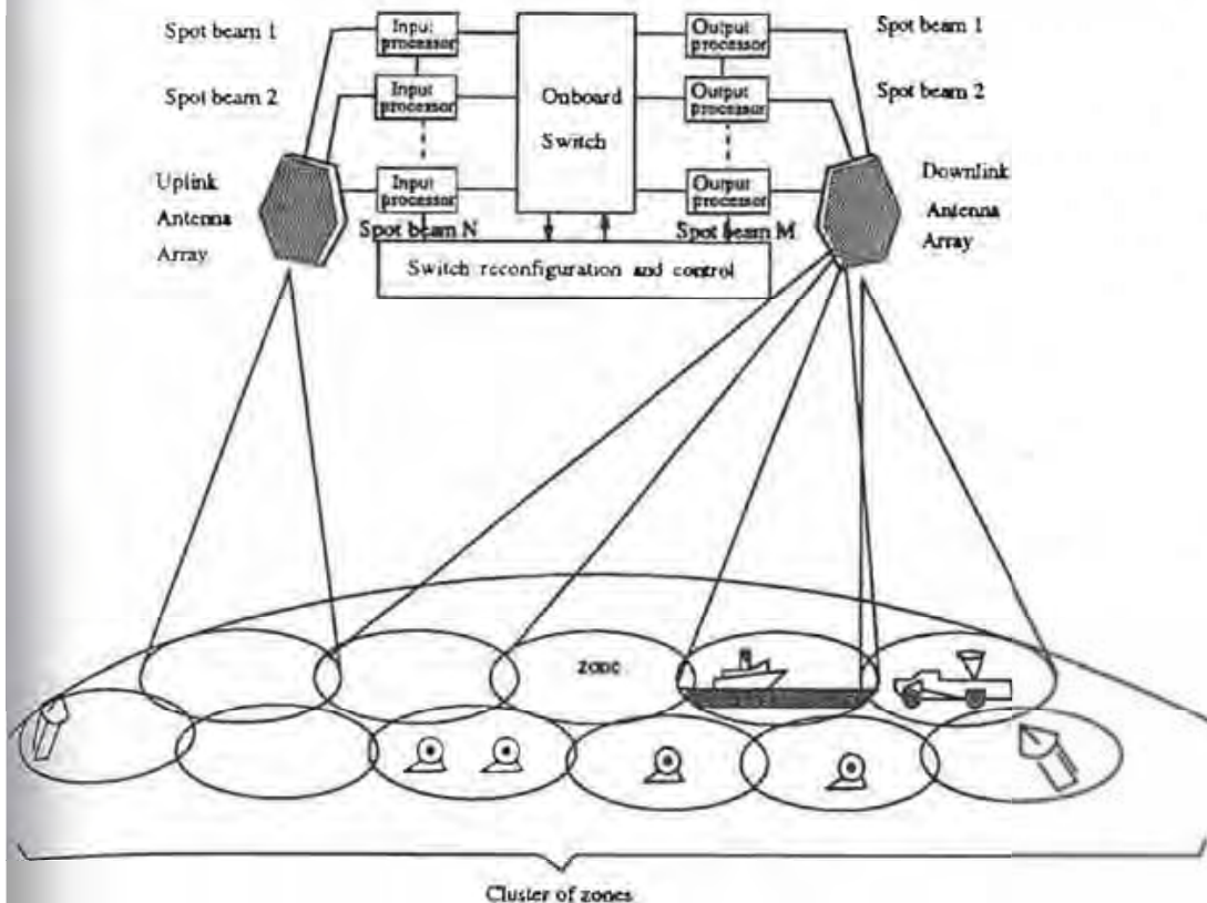
FIGURE 72.1 Onboard (OB) processing satellite using multiple-beam antennas and onboard switching.
