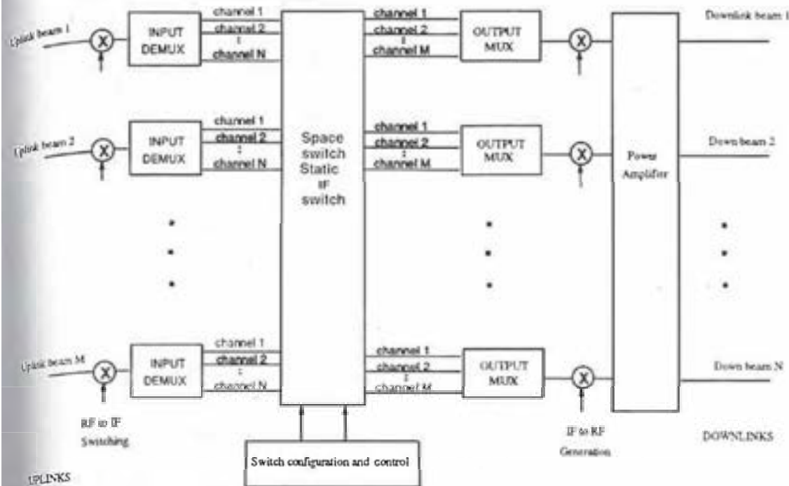
FIGURE 72.2 Nonregenerative onboard IF switching.
