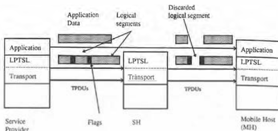
FIGURE 96.7 LPTSL, an approach to handle dynamic bandwidth variations.
