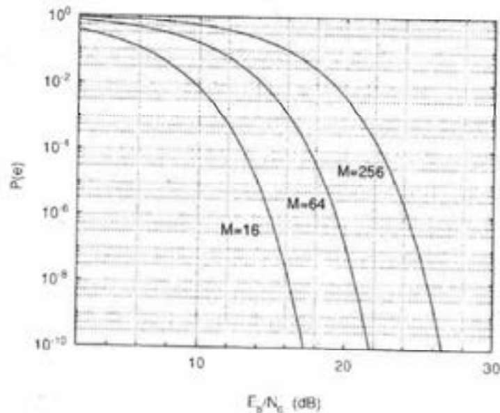
FIGURE 21.7 Symbol error probability of coherently demodulated QAM.
