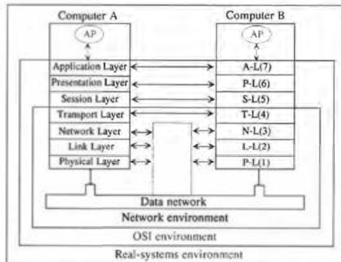
FIGURE 41.3 Overall structure of the ISO reference model.
