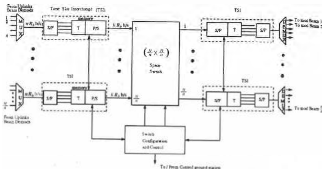
FIGURE 72.6(a) T-S-T baseband switching.
