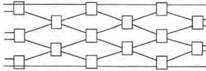
FIGURE 72.4(b) Multistage implementation of an optical N \times N switch using N(N-1)/2 .
