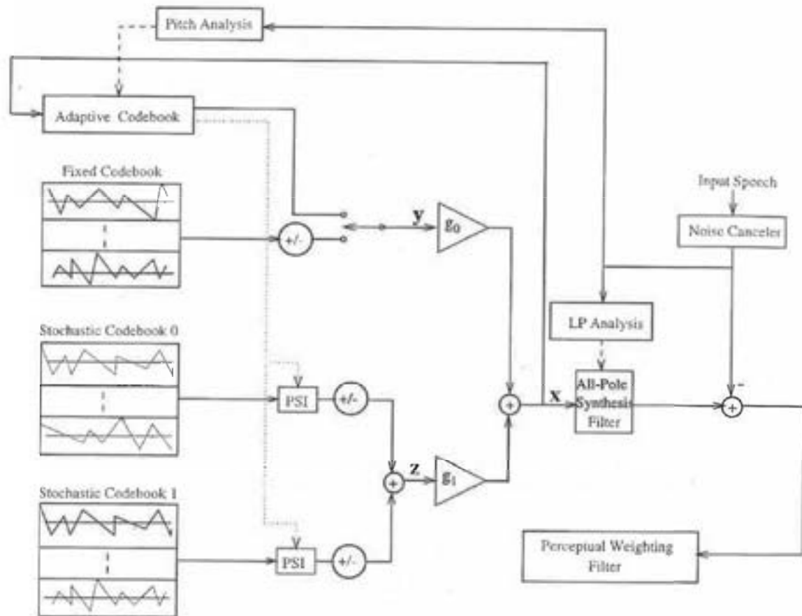
FIGURE 94.2 Basic structure of the PSI-CELP encoder.
