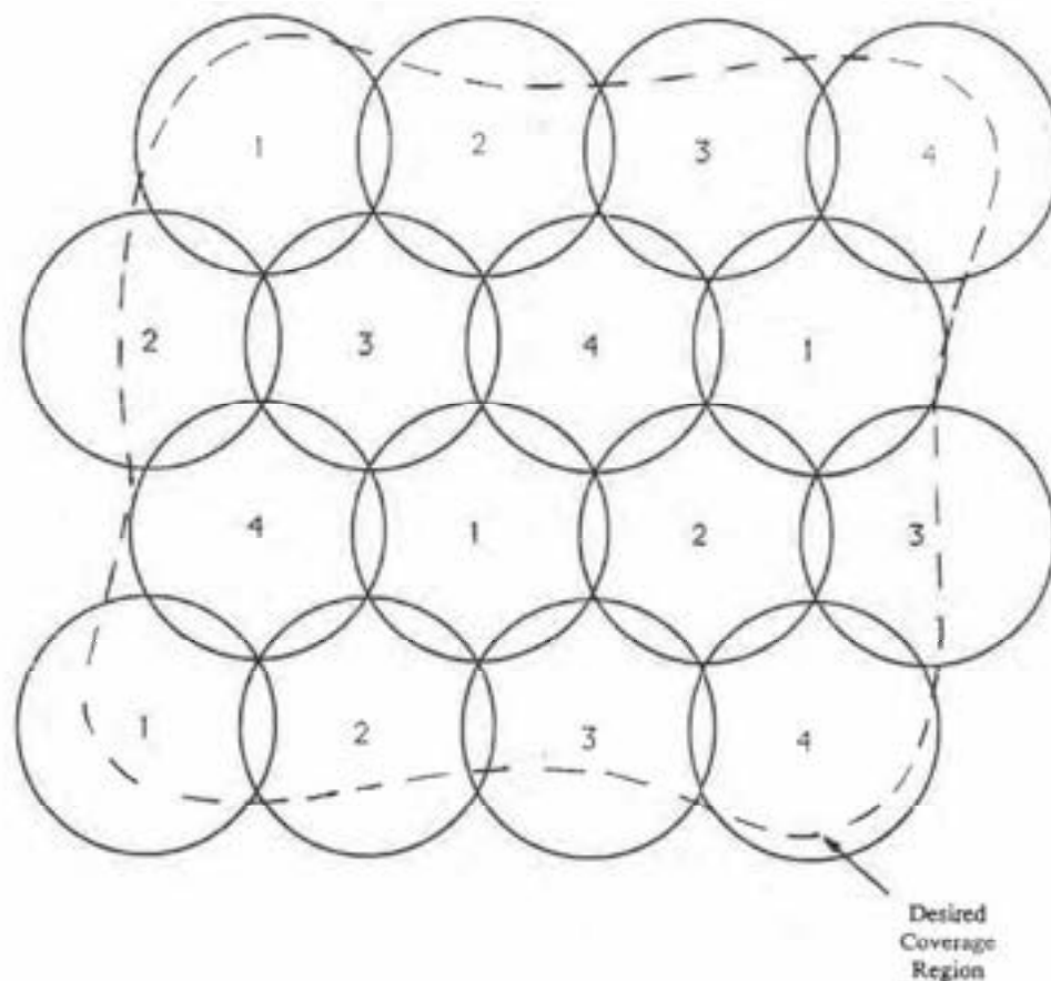
FIGURE 74.1 An example illustrating frequency reuse with a multiple-beam satellite. Here, the total allocated system frequency band is divided into four subbands. The assignment of the subbands to the beams is denoted by the number shown in each beam.
