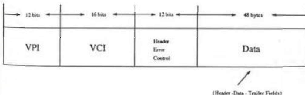
FIGURE 72.14 ATM cell/user network interface (UNI).
