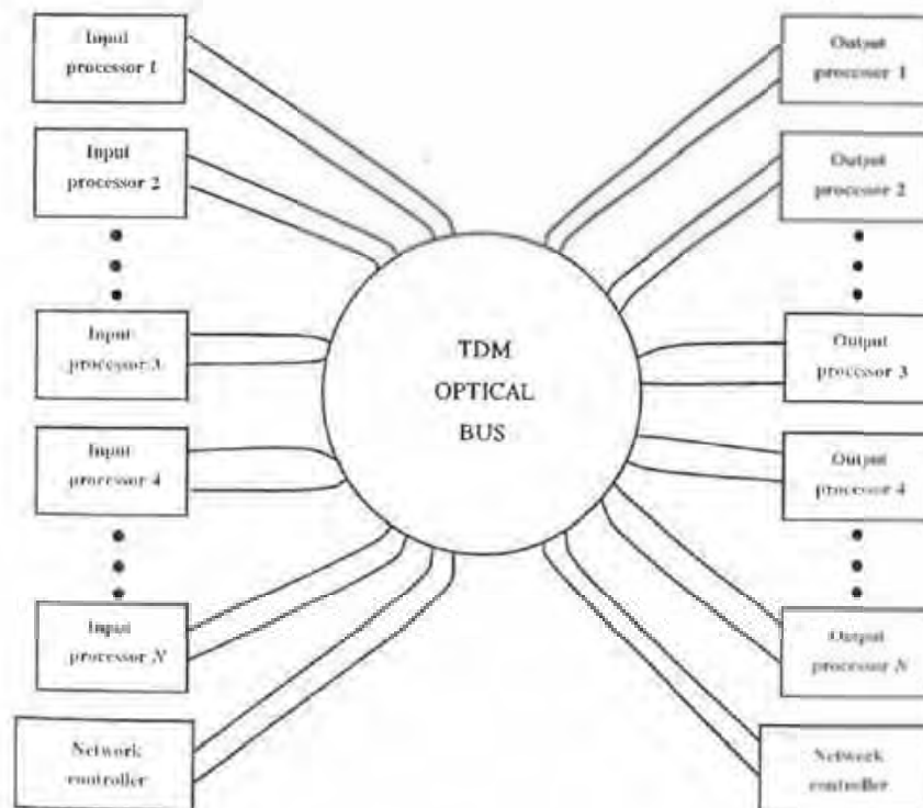
FIGURE 72.12 Onboard TDM optical ring switch.
