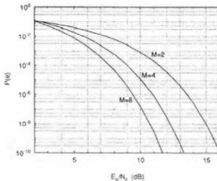
FIGURE 21.8 Symbol error probability of coherently demodulated orthogonal FSK.
