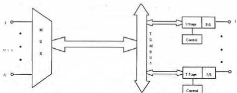
FIGURE 72.8 Distributed memory switch (DMS).
