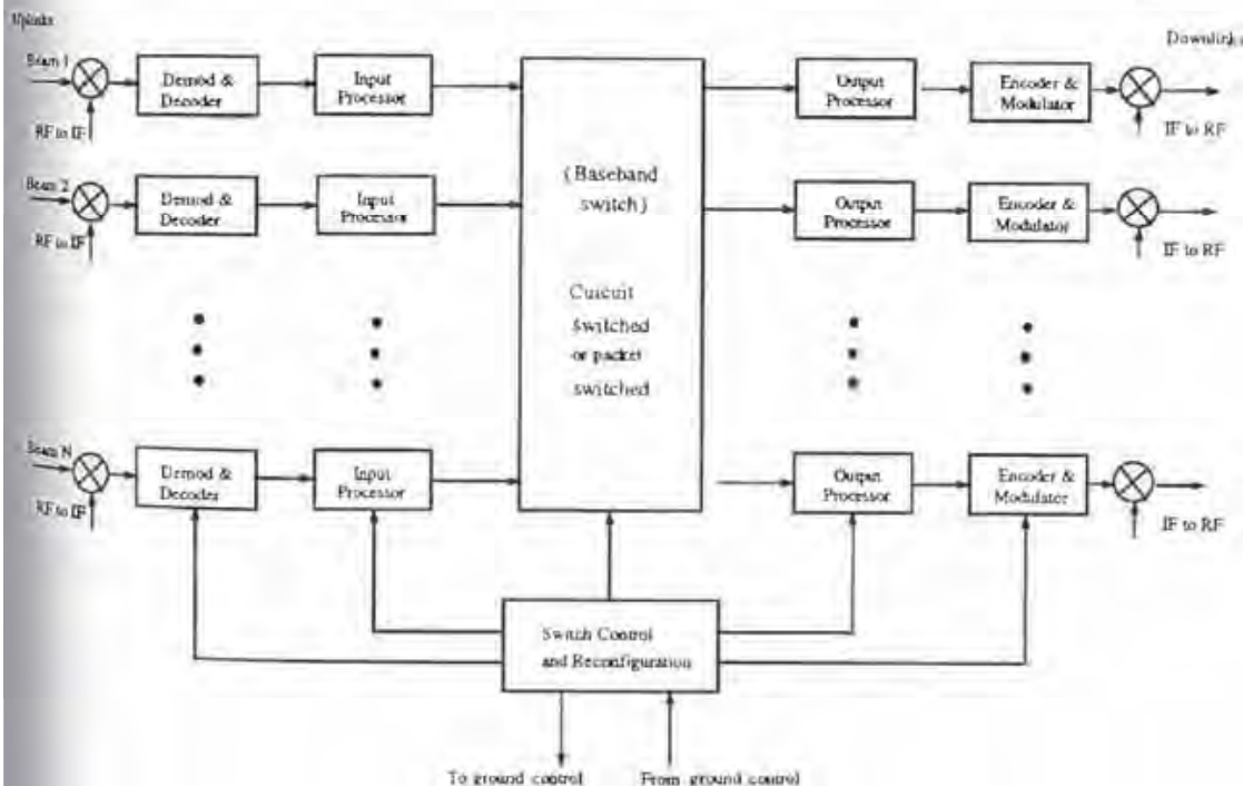
FIGURE 72.5 Building blocks of onboard baseband switching.
