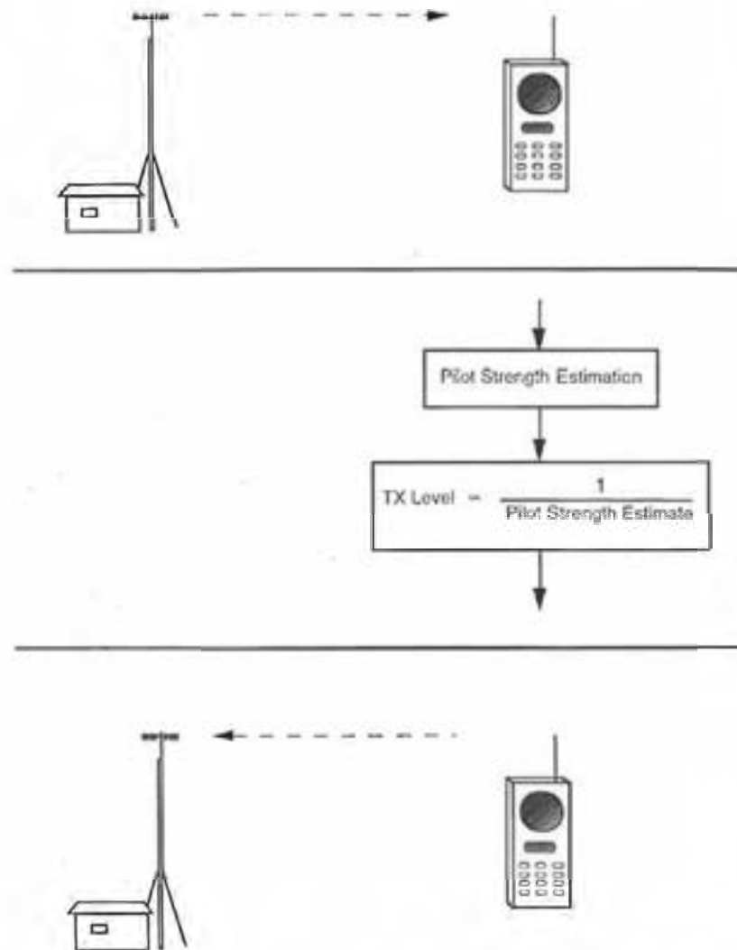
FIGURE 85.1 Reverse link open-loop power control.
