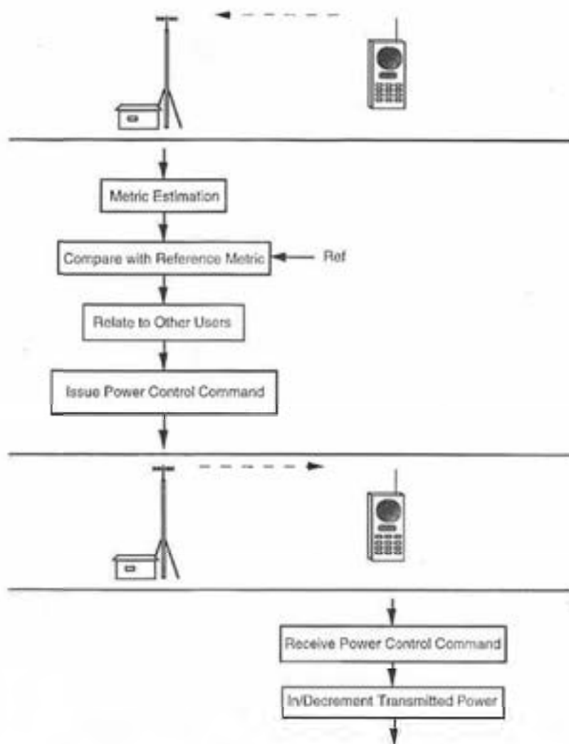
FIGURE 85.2(a) Reverse link closed-loop power control.
