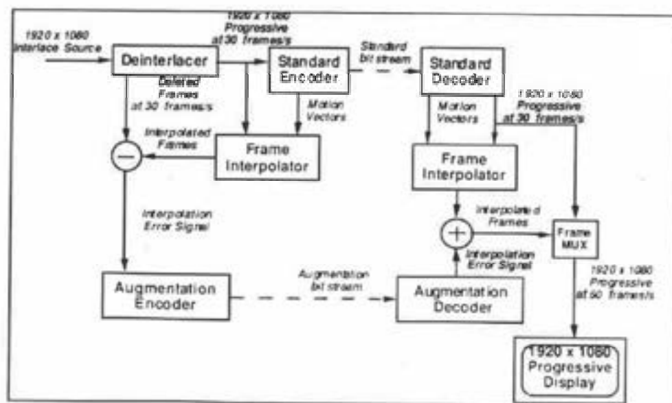
FIGURE 103.6 Possible migration scenario from interlaced source to 1080 progressive display.
