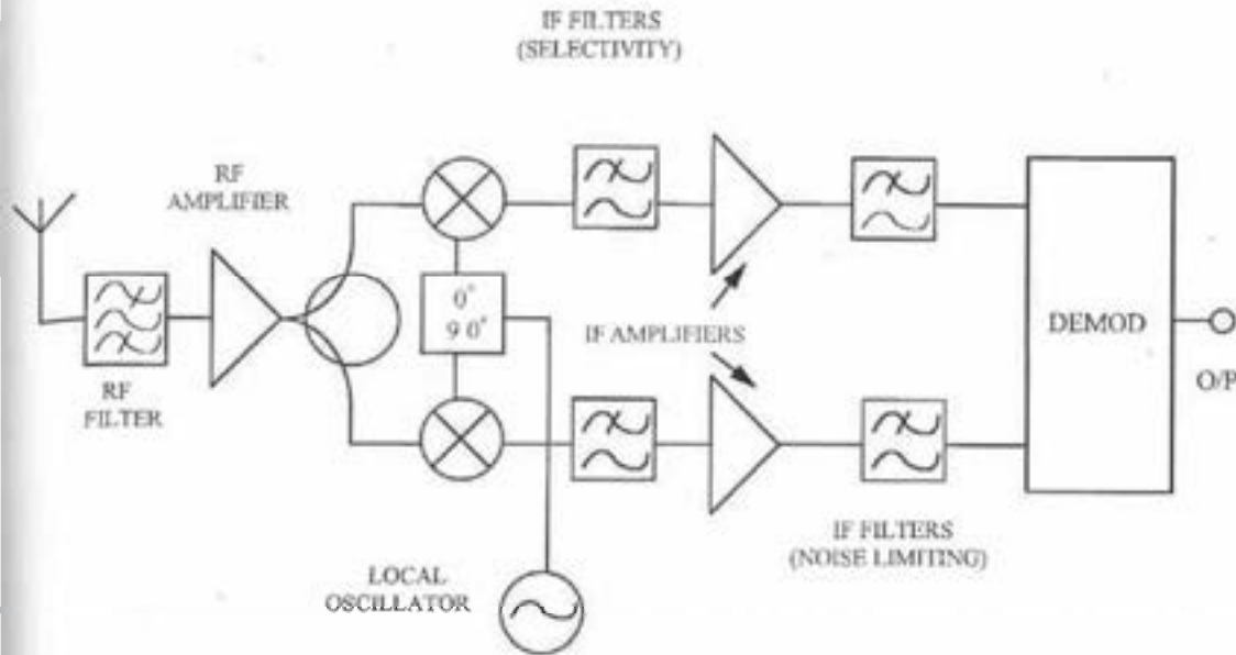
FIGURE 92.13 Direct conversion receiver architecture.
