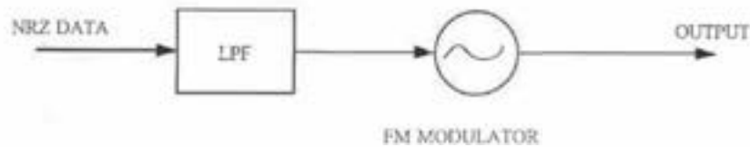
FIGURE 92.10 Premodulation baseband-filtered MSK.
