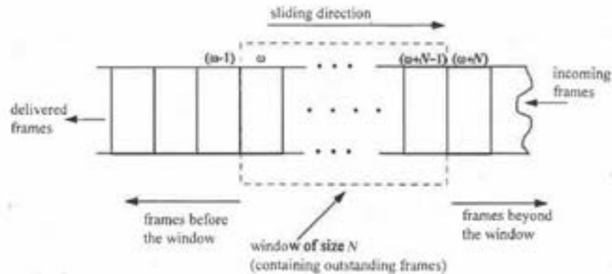
FIGURE 15.3 Frame sequencing in a sliding window protocol (sender side).
