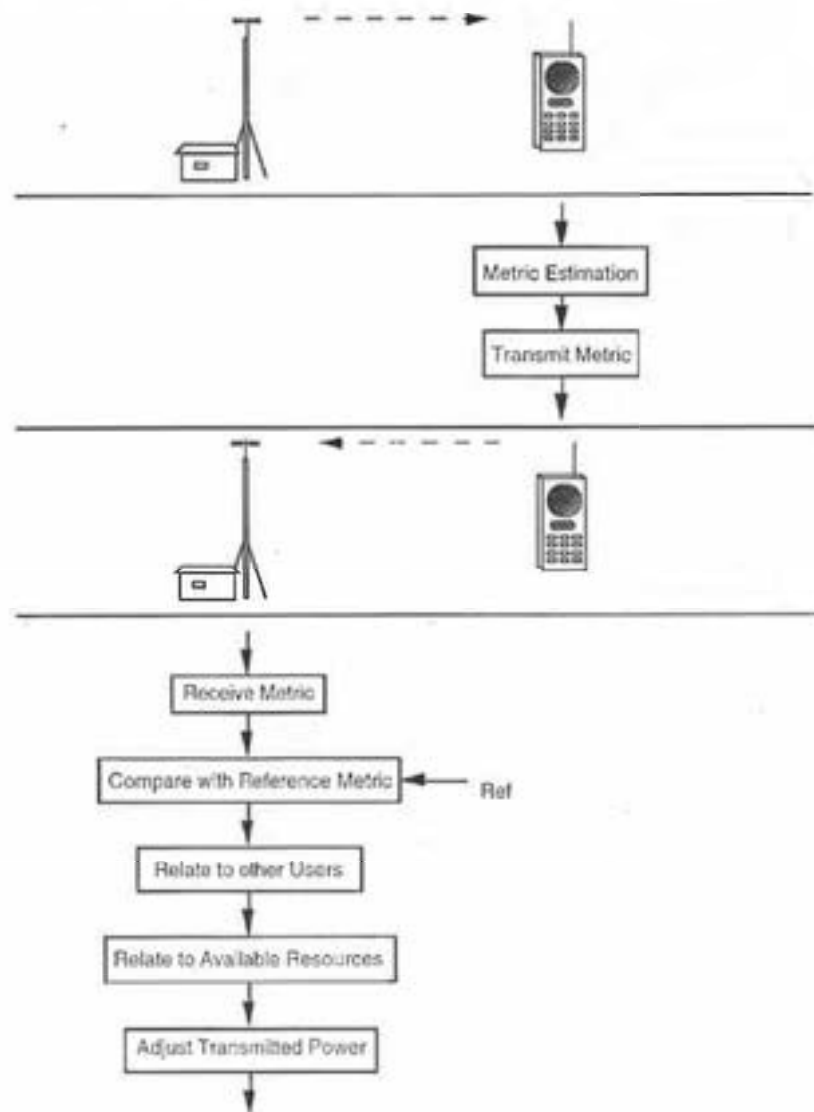
FIGURE 85.2(b) Forward link closed-loop power control.
