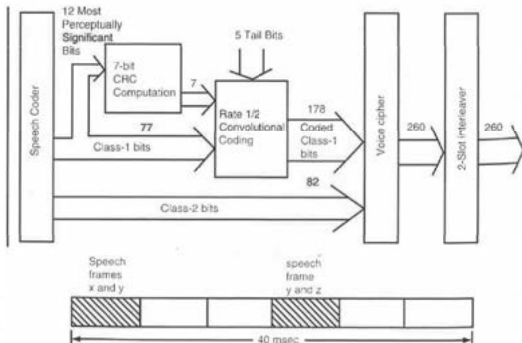
FIGURE 88.5 Error correction insertion for speech coder. Source TIA, 1992. Cellular Systems Dual-Mode Mobile Station-Base Station Compatibility Standards. TIA/EIA IS-54. With permission.
