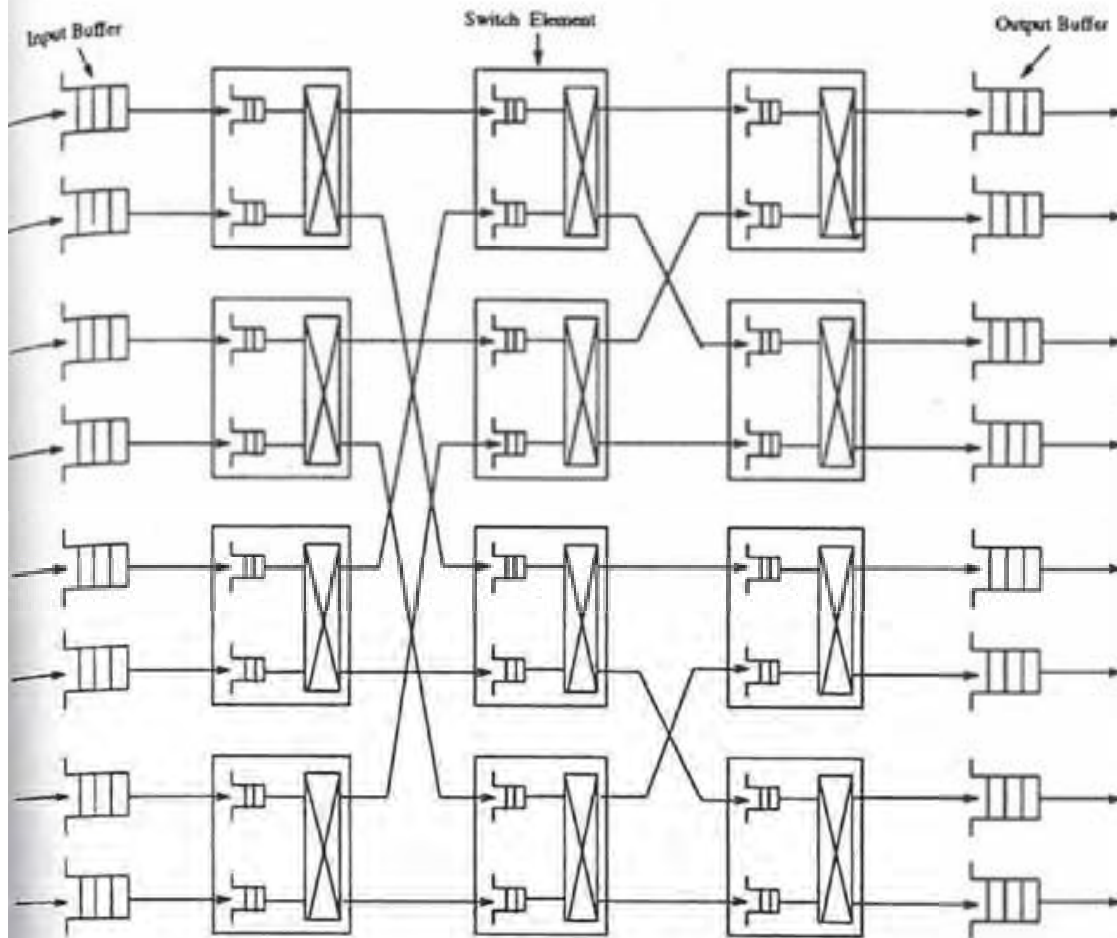
FIGURE 72.10 A buffered Banyan network.
