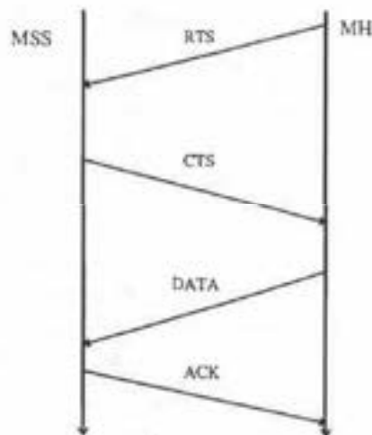
FIGURE 96.3 CSMA/CA and four-way handshaking protocol.
