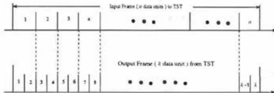
FIGURE 72.6(b) Time slot interchange (TSI) reading from T-stage is at least twice as fast as writing into this stage ( k \geq 2n - 1 ).
