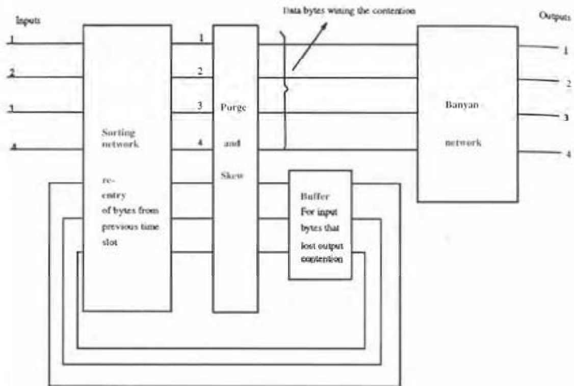
FIGURE 72.11 A Starlite network.
