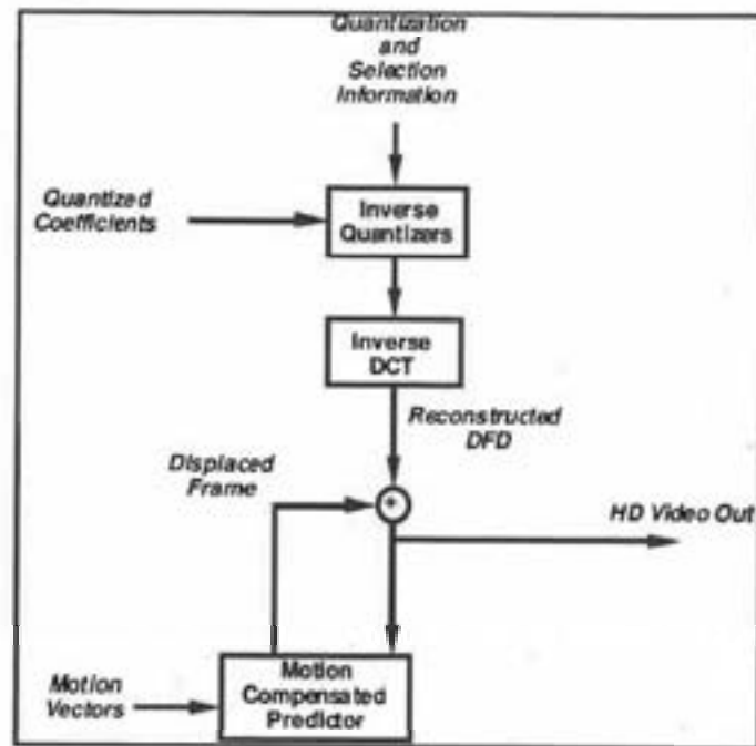
FIGURE 103.3 Video decoder loop.
