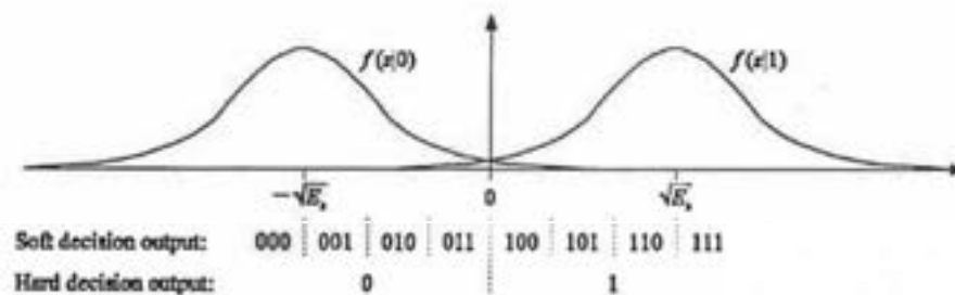
FIGURE 14.2 Hard and soft decision demodulation of a coherently demodulated BPSK signal corrupted by AWGN. f(z|1) and f(z|0) are the Gaussianly distributed conditional probability density functions at the threshold device.
