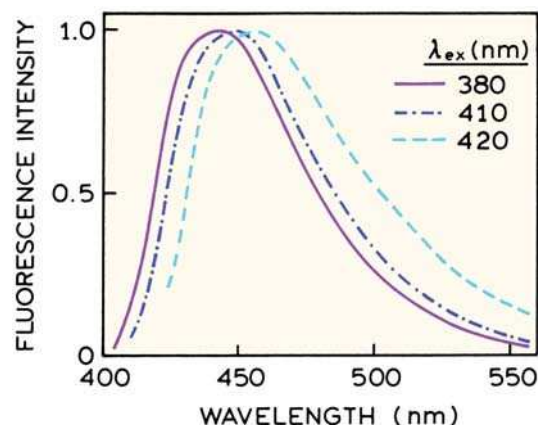
Figure 7.38. Fluorescence emission spectra 8-anilinnaphthalene-1-sulfonic acid in 1-propanol at 77°K. Excitation and emission bandpass are both 5 nm. Revised from [95].
