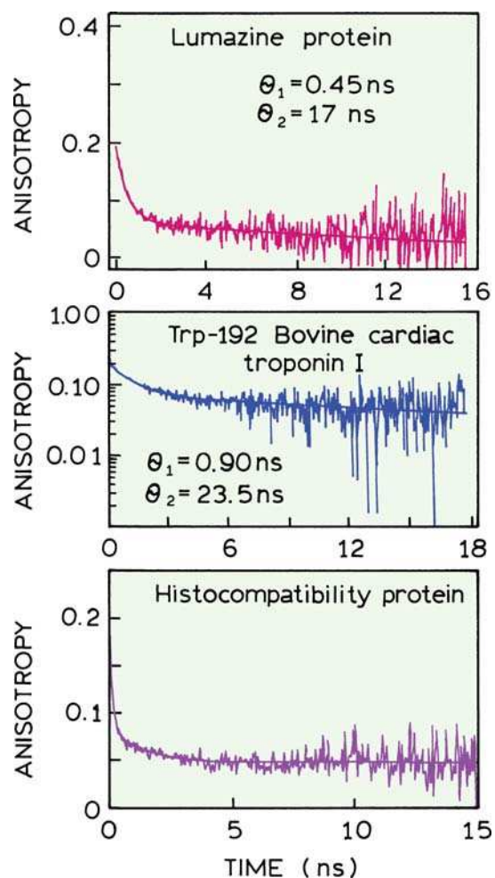
Figure 17.24. Anisotropy decay for the single-tryptophan residue in the lumazine protein (top), for trp-192 in bovine cardiac troponin I (middle) and for a histocompatibility protein (bottom). Revised from [74], [75], and [76].
