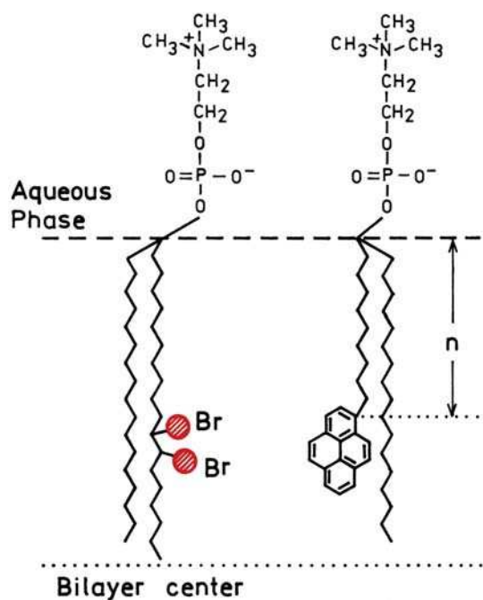
Figure 8.30. Schematic representation of the structures of Pyr n PC and Br x,y PC species used to study depth-dependent quenching of the pyrene moiety. Revised and reprinted with permission from [63]. Copyright © 1995, American Chemical Society.
