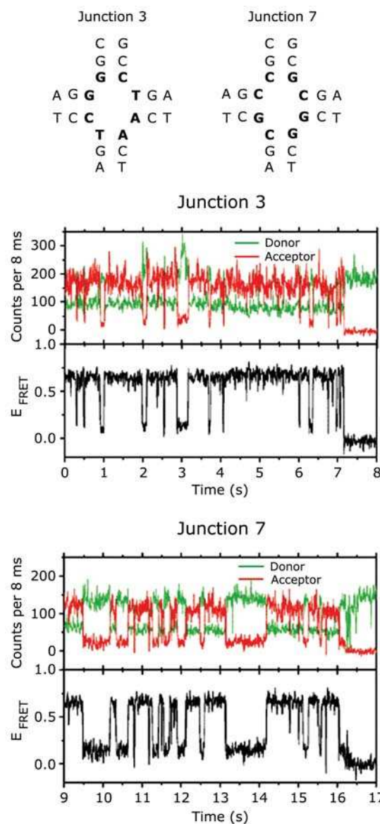
Figure 23.48. Single-molecule conformational changes in two Holliday junctions. Junctions 3 and 7 refer to different sequences; E_{\text{FRET}} = I_A / (I_A + I_D) . Reprinted with permission from [83].
