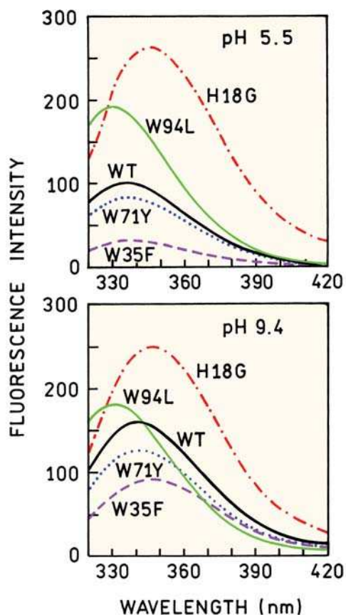
Figure 16.50. Fluorescence emission spectra of the wild-type (WT) barnase and its mutants in buffer at pH 5.5 (top), where histidine 18 is protonated and at pH 9.4 where histidine is neutral (bottom). Also shown are the emission spectra of the single-tryptophan mutants at these pH values. Revised and reprinted with permission from [139]. Copyright © 1991, American Chemical Society.
