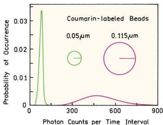
Figure 24.27. Photon-count histogram for a mixture of 0.05 and 0.115 \mu\text{m} coumarin-labeled beads. Revised from [87].
