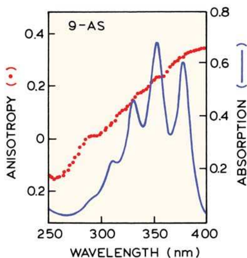
Figure 10.8. Excitation anisotropy spectrum of 9-anthroxystearic acid (9-AS) in propylene glycol at -52^{\circ}\text{C} . The same excitation anisotropy spectrum was observed for 2-AS, 7-AS, 12-AS and 16-AP. Revised and reprinted with permission from [16]. Copyright © 1982, American Chemical Society.
