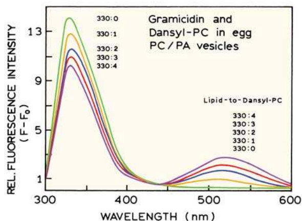
Figure 13.30. Emission spectra of gramicidin and dansyl-PC in vesicles composed of egg PC and egg PA. \lambda_{\text{ex}} = 282 nm. Dansyl-PC is 1-acetyl-2-[11-N-[5-dimethylamino naphthalene-1-sulfonyl]amino] undecanoyl phosphatidylcholine. The lipid-to-dansyl PC ratios are shown on the figure. Revised and reprinted with permission from [72]. Copyright © 1988, American Chemical Society.
