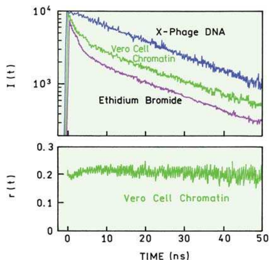
Figure 11.30. Intensity and anisotropy decays of EB-stained chromatin from S2 phase Vero cells. Also shown as a control is the intensity decay of EB bound to x-phase DNA. Revised from [95].
