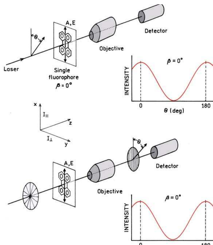
Figure 23.33. Polarization properties of a single fluorophore with colinear ( \beta = 0^\circ ) absorption (A) and emission (E) dipoles.
