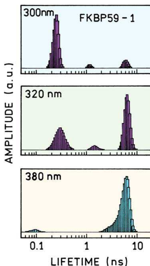
Figure 4.64. Lifetime distribution of the immunophilin FKBP59-1 recovered by the MEM. Revised from [219].
