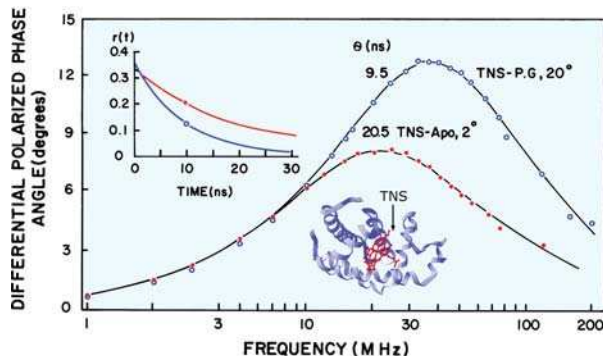
Figure 11.15. Frequency-domain anisotropy decays of 2-p-toluidinyl-6-naphthalene sulfonic acid in propylene glycol (PG) and bound to apomyoglobin (Apo). Insert: TD anisotropy decays. From [67].
