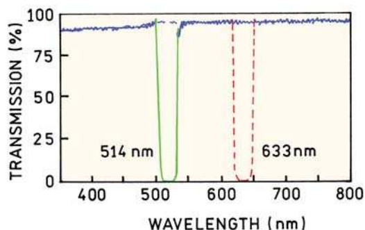
Figure 23.15. Transmission profiles of laser notch filters.
