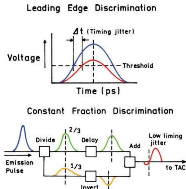
Figure 4.22. Constant fraction discrimination in TCSPC. Top: Timing error due to pulse height variations using leading edge discrimination. Bottom: Operation of a constant fraction discriminator.
