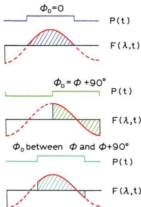
Figure 5.49. Phase-sensitive detection of fluorescence. The detector phase ( \phi_D ) can be in phase with the emission \phi_D = \phi (top), out of phase with the emission ( \phi_D = \phi + 90^\circ , middle), or at some intermediate value (bottom).
