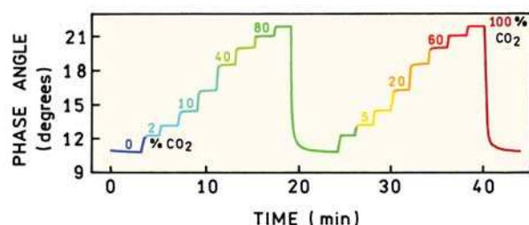
Figure 19.22. \text{CO}_2 -dependent phase angles of [\text{Ru}(\text{dpp})_3]^{2+} in the sensor matrix containing Sudan III. The output of the LED was modulated at 20 kHz. Revised from [69].
