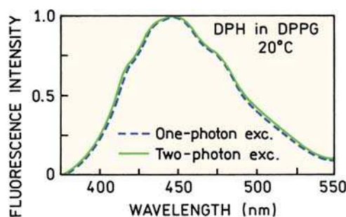
Figure 18.12. Fluorescence emission spectra of DPH in DPPG bilayers for excitation at 358 nm (dashed) and 716 nm (solid). From [36].
