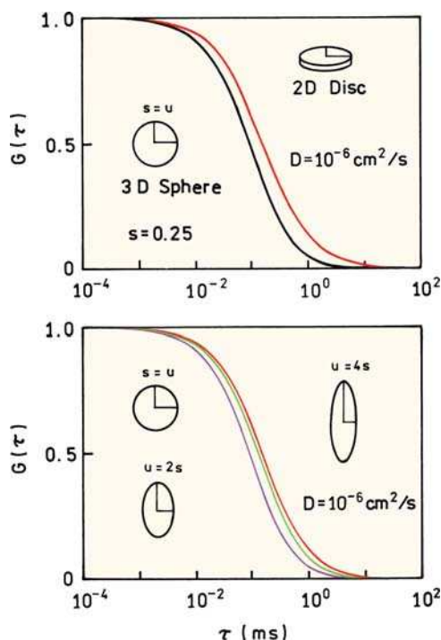
Figure 24.18. Simulated autocorrelation functions for a sphere in three dimensions and a disk in two dimensions (top), and for spherical and elongated 3-dimensional shapes (bottom). D = 10^{-6} cm 2 /s and s = 0.25 \mu m.
