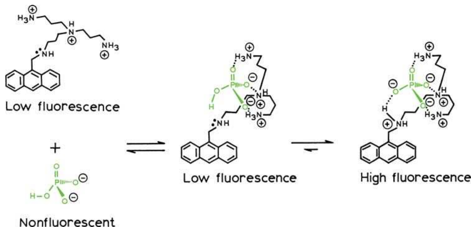
Figure 19.42. Phosphate sensing with an alkylamino anthracene derivative. Revised and reprinted with permission from [134]. Copyright © 1989, American Chemical Society.
