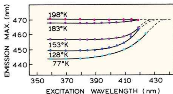
Figure 7.39. Temperature dependence of fluorescence excitation red shift for 8-anilinnaphthalene-1-sulfonic acid in 1-propanol. Revised from [95].
