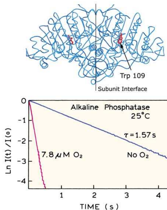
Figure 8.70. Phosphorescence decay of alkaline phosphatase, 25^\circ\text{C} , in the absence of oxygen and in the presence of 7.8\ \mu\text{M} oxygen. Revised and reprinted with permission from [174]. Copyright © 1987, Biophysical Society.
