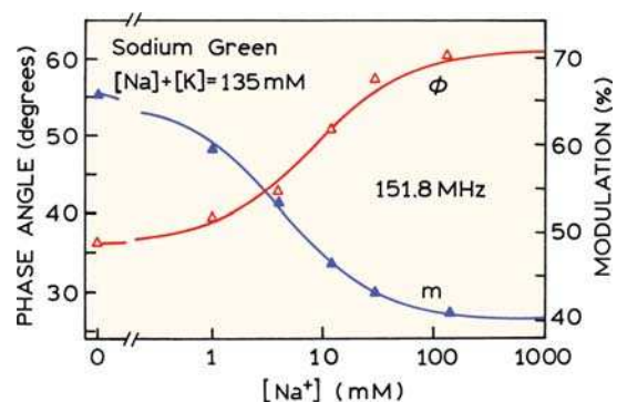
Figure 19.48. Sodium-dependent phase ( \phi ) and modulation ( m ) of Sodium Green. Excitation was at 514 nm, and emission was observed above 530 nm. Data from [151].
