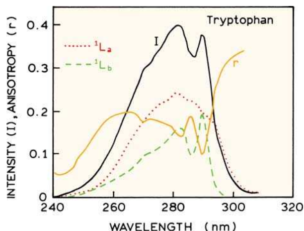
Figure 16.4. Excitation anisotropy spectra of tryptophan in propylene glycol at -50^{\circ}\text{C} . Also shown are the anisotropy-resolved spectra of the ^1\text{L}_a (dotted) and ^1\text{L}_b (dashed) transitions. Data from [18].
