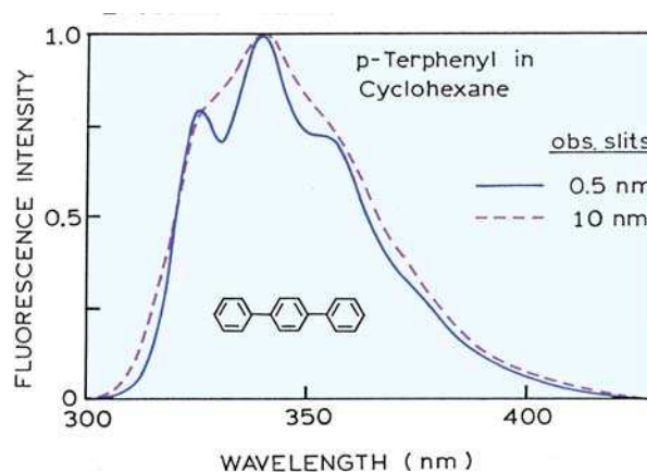
Figure 2.13. Emission spectra of p-terphenyl collected with a spectral resolution of 0.5 and 10 nm. From [10].
