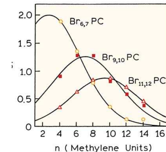
Figure 8.31. Dependence of K_{SV}^{app} , the apparent Stern-Volmer quenching constant, on n , the number of methylene units in the pyrenylacyl chains, for bilayers with different Br x,y PC quenchers. The subscripts x and y indicate the location of the bromine atoms. The bilayers consisted of 1-palmitoyl-2-oleoylphosphatidylcholine (POPC) with 50 mole% cholesterol. Revised and reprinted with permission from [63]. Copyright © 1995, American Chemical Society. Structure courtesy of Dr. Alexey S. Ladokhin from University of Kansas.
