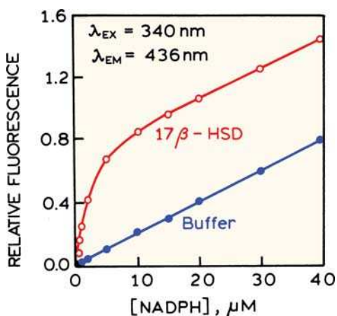
Figure 3.7. Fluorescence intensity of NADPH titrated into buffer (●) or a solution of 17β-HSD (○). Revised from [29].
