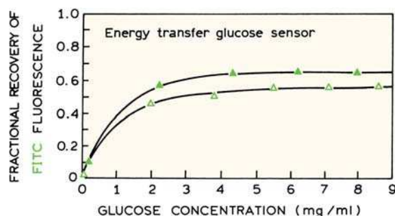
Figure 19.25. Recovery of FITC fluorescence during glucose titration for two weight ratios of Rh-ConA/FITC-dextran, 217 (▲) and 870 w/w (Δ). Revised from [81].
