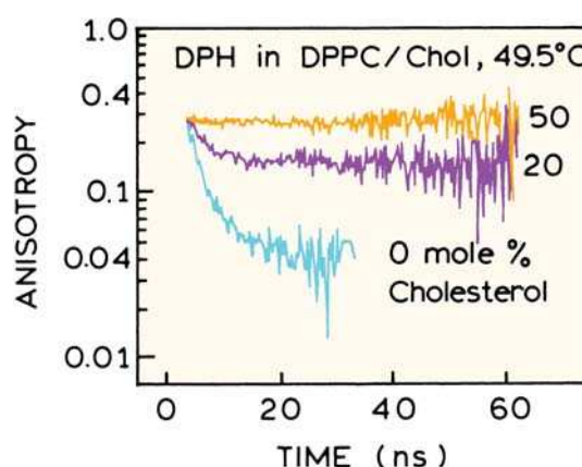
Figure 11.20. Anisotropy decays of DPH in DPPC vesicles at 49.5°C, containing 0, 20, and 50 mole% cholesterol. At 49.5°C the DPPC membranes are above their phase transition temperature, which is near 37°C. Revised and reprinted with permission from [69]. Copyright © 1978, American Chemical Society.
