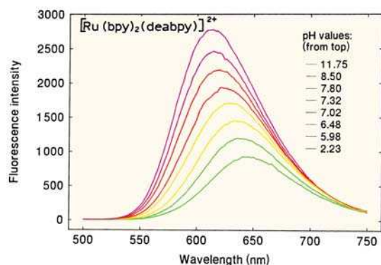
Figure 20.44. pH-dependent emission spectra of \text{Ru}(\text{bpy})_2(\text{deabpy})(\text{PF}_6)_2 . Excitation at 414 nm. Revised from [181].
