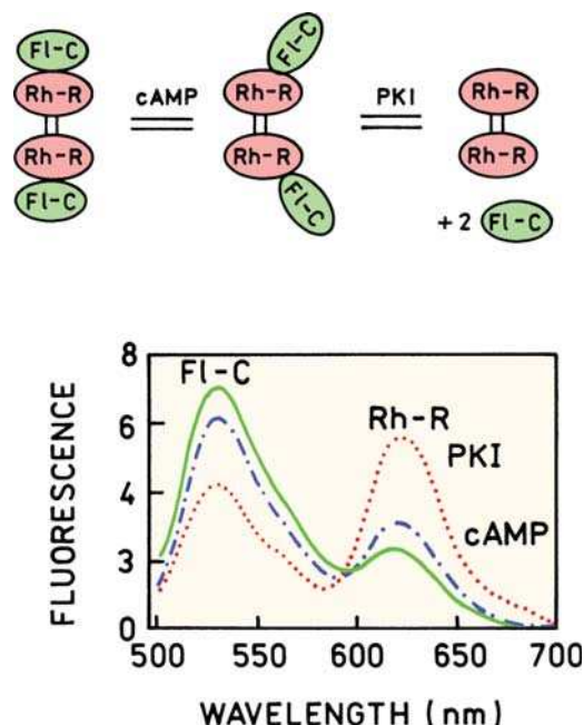
Figure 13.40. Emission spectra and schematic for the effect of cAMP and PKI on the emission spectra of the (Rh-R) 2 -(Fl-C) 2 complex. Revised and reprinted with permission from [99]. Copyright © 1993, American Chemical Society.
