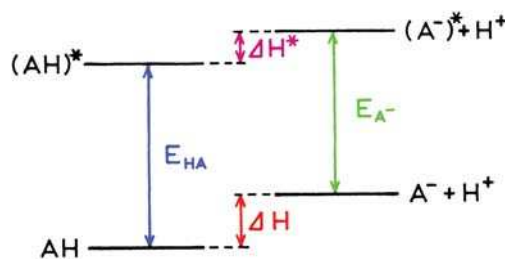
Figure 7.44. Electronic energy levels of an acid AH and its conjugate base A^- in the ground and excited states (the Förster cycle). Reprinted with permission from [131], the Journal of Chemical Education , Vol. 69, No. 3, 1992, pp. 247–249. Copyright © 1992, Division of Chemical Education Inc.
