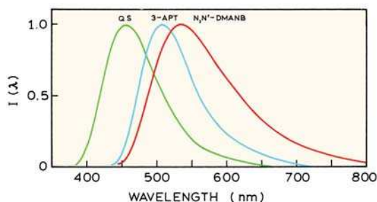
Figure I.7. Corrected emission spectra in relative quanta per wavelength interval I(\lambda) . The quinine sulfate (QS) was in 0.1 N H_2SO_4 . 3-aminophthalimide (3-APT) was in 0.1 N H_2SO_4 . N,N-dimethylamino-m-nitrobenzene (N,N-DMANB) was in 70% n-hexane, 30% benzene. Modified from [4].
