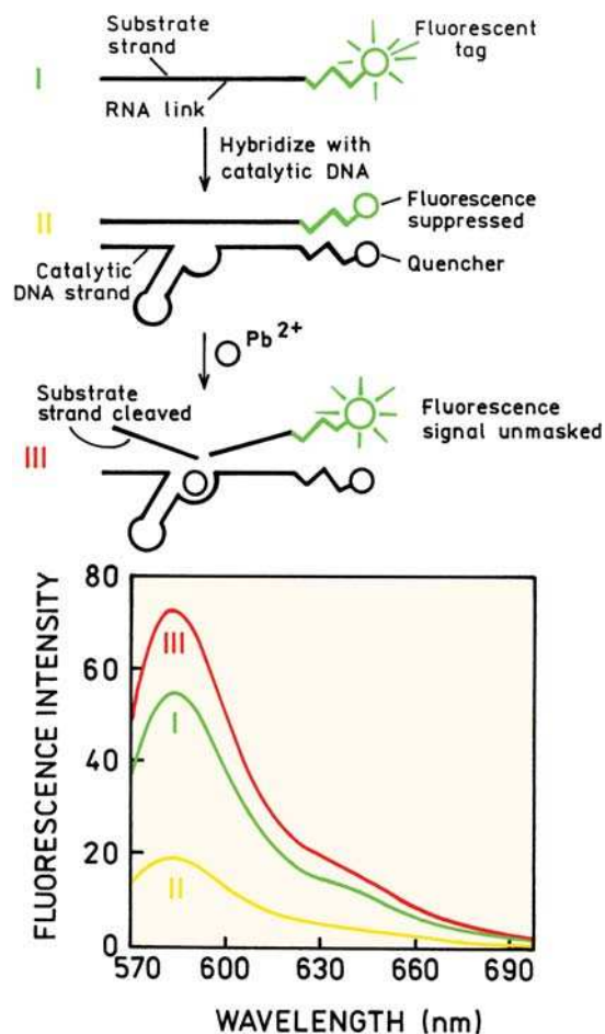
Figure 21.45. Detection of Pb^{2+} using a DNzyme. The fluorophore is TAMRA and the quencher is dabcyI. From [142].
