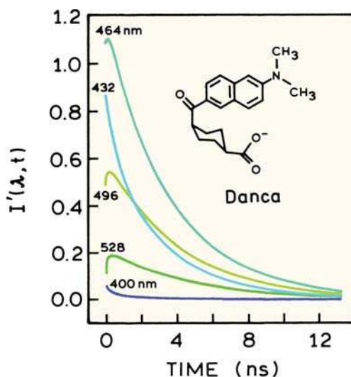
Figure 7.9. Deconvolved fluorescence decays of Danca-apomyoglobin complex from 400 to 528 nm at 298°K. The area under each trace has been scaled to the steady-state intensity at that wavelength. Note the intensity decays show a rise time at longer wavelengths. Revised and reprinted with permission from [17]. Copyright © 1992, American Chemical Society.
