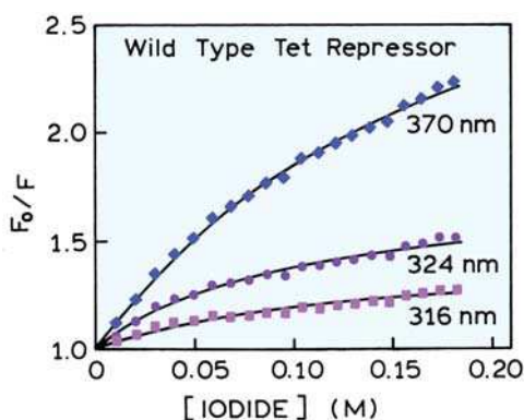
Figure 8.40. Iodide Stern-Volmer plots for the wild type tet repressor. The solution contained 1 mM sodium thiosulfate to prevent formation of I_2 . From [107].
