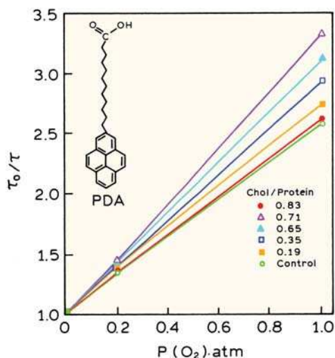
Figure 8.23. Oxygen quenching of pyrene dodecanoic acid in erythrocyte ghost membranes with various cholesterol/protein ratios: ○, control, no added cholesterol; ■, 0.19; □, 0.35; ▲, 0.65; △, 0.71; ●, 0.83. Revised from [59].
