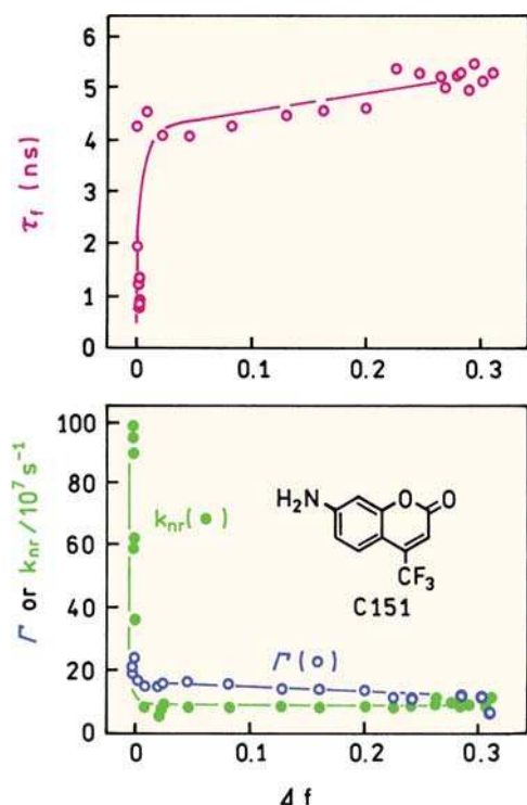
Figure 6.32. Lifetimes, radiative, and non-radiative decay rates for C151 in various solvents. Revised and reprinted with permission from [78]. Copyright © 2001, American Chemical Society.
