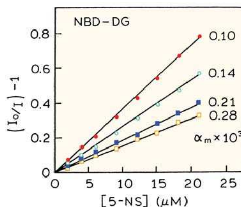
Figure 8.33. Quenching of 1-oleoyl-2-hexanoyl-NBD-glycerol (NBD-DG) by 5-doxylstearate (5-NS). \alpha_m refers to the volume fraction of the egg PC phase. Revised from [92]. Copyright © 1994, with permission from Elsevier Science.
