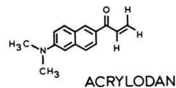
Figure 6.22. Derivatives of Prodan.
