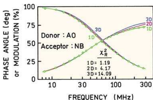
Figure 15.13. Frequency-domain intensity decay of AO-DNA with 0.058 NB/base pair. From [18]: Maliwal BP, Kusba J, Lakowicz JR. 1994. Fluorescence energy transfer in one dimension: frequency-domain fluorescence study of DNA-fluorophore complexes. Biopolymers 35:245–255. Copyright © 1994. Reprinted with permission from John Wiley and Sons Inc.
