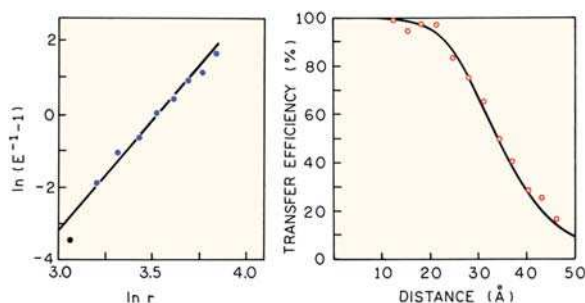
Figure 13.41. Distance dependence of the energy transfer efficiencies in dansyl-(L-propyl)- \alpha -naphthyl; n = 1-12 . Revised from [18].
