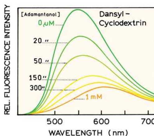
Figure 6.45. Emission spectra of dansyl-cyclodextrin with increasing concentrations of 1-adamantanol. Probe concentrations = 10 M. Revised from [98].
