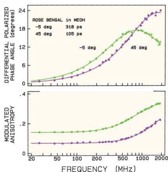
Figure II.8. Rose Bengal as a picosecond correlation time standard. For additional data on Rose Bengal see [4].
