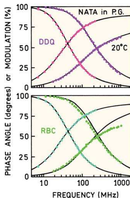
Figure 9.28. Frequency-domain intensity decays of NATA in propylene glycol at 20°C in the presence of increasing (left to right) concentrations of acrylamide (1.5 M). The solid lines (top) show the best fit to the DDQ model using a = 5 \text{ \AA} and r_c = 0.319 \text{ \AA} . The solid lines (bottom) show the best fit to the RBC model using a = 5 \text{ \AA} . Revised with permission from [78]. Copyright © 1994, American Society for Photobiology.
