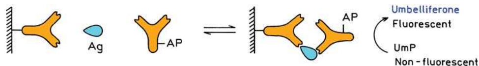
Figure 19.69. Schematic of an enzyme-linked immunosorbent assay (ELISA). AP is alkaline phosphatase. Ag is an antigen, and UmP is umbelliferoyl phosphate.
