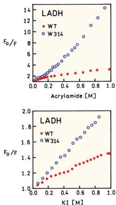
Figure 16.77. Stern-Volmer plots for acrylamide and iodide quenching of WT-LADH and the W314L tryptophan mutant.
