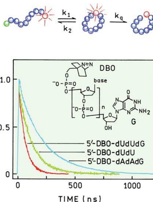
Figure 8.67. Intramolecular quenching of a DBO-labeled oligomer by a terminal guanine residue. Revised and reprinted with permission from [156]. Copyright © 2004, American Chemical Society.
