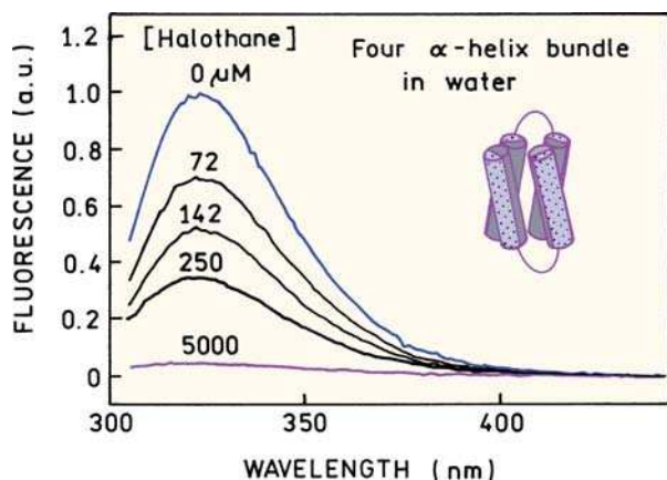
Figure 8.43. Emission spectra of a four \alpha -helix bundle in water in the presence of halothane. Each peptide chain contains one tryptophan residue. Revised from [114].
