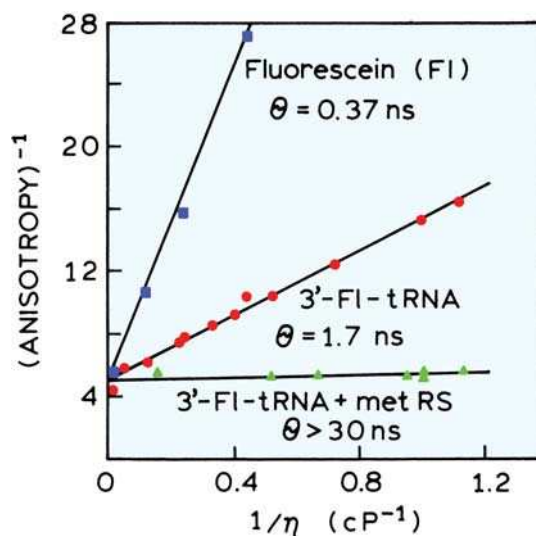
Figure 10.16. Perrin plot of fluorescein (FI, ■) and tRNA Met labeled at the 3' end with fluorescein (●). Also shown is the labeled t-RNA when bound to methionyl-tRNA synthetase (met RS, ▲). The experiments were performed at 20°C. The viscosity \eta was varied by adding sucrose. Excitation at 480 nm and emission at 520 nm. Revised and reprinted with permission from [43]. Copyright © 1986, American Chemical Society.
