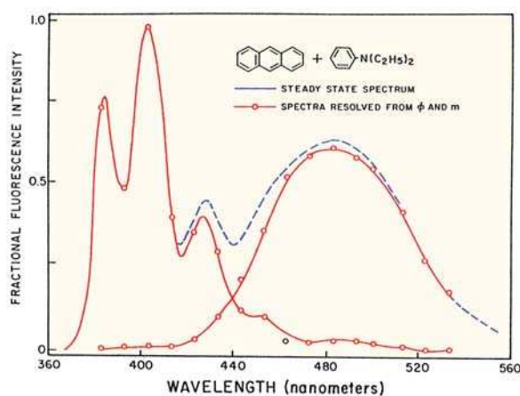
Figure 5.54. Resolution of the monomer and exciplex emission of anthracene. The spectra were calculated using eqs. 5.81 and 5.82 and the data shown in Figure 5.53. Reprinted from [169], Copyright © 1982, with permission from Elsevier Science.
