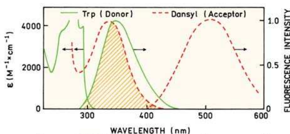
Figure 13.9. Overlap integral for energy transfer from a tryptophan donor to a dansyl acceptor on melittin R_0 = 23.6 Å. Data from [31].
