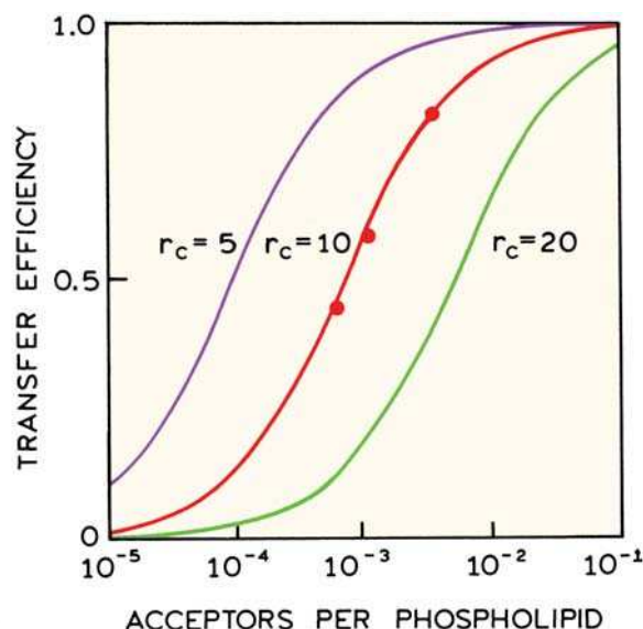
Figure 15.24. Diffusion-limited energy transfer from \text{Tb(DPA)}_3 trapped in the inner volume of egg PC vesicles labeled with eosin-phosphatidylethanolamine as the acceptor. The solid lines were calculated using eq. 15.23 assuming R_0 = 45.6 Å and b = 150 Å, and assuming an area of 70 Å 2 per phospholipid. Revised from [58].
