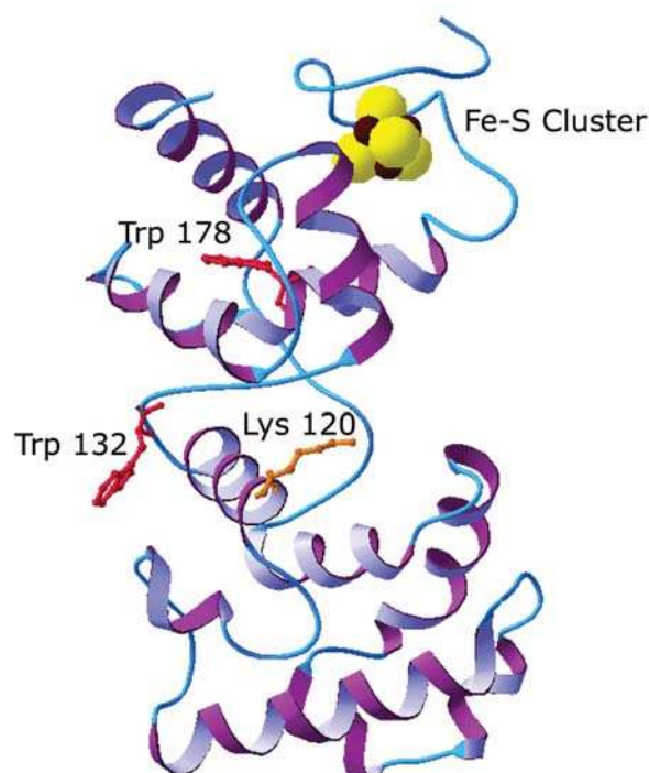
Figure 8.15. Structure of Endo III showing the exposed residue trp 132 and the buried residue trp 178 near the iron-sulfur cluster.
