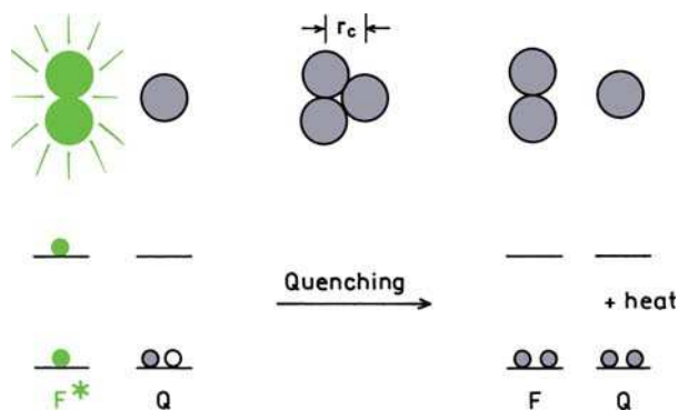
Figure 9.2. Schematic of fluorescence quenching.
