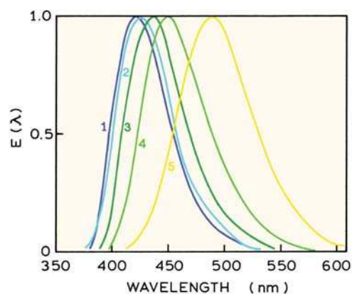
Figure I.4. Corrected and normalized fluorescence spectra for some \beta -carboline derivatives: (1) harmine 0.1 N \text{H}_2\text{SO}_4 ; (2) 2-methyl harmine 0.1 N \text{H}_2\text{SO}_4 ; (3) harmine 0.1 N \text{H}_2\text{SO}_4 ; (4) nor-harmine 0.1 N \text{H}_2\text{SO}_4 ; (5) harmaline 0.01 N \text{H}_2\text{SO}_4 . Revised from [2]. Copyright © 1992, with permission from Elsevier Science.
