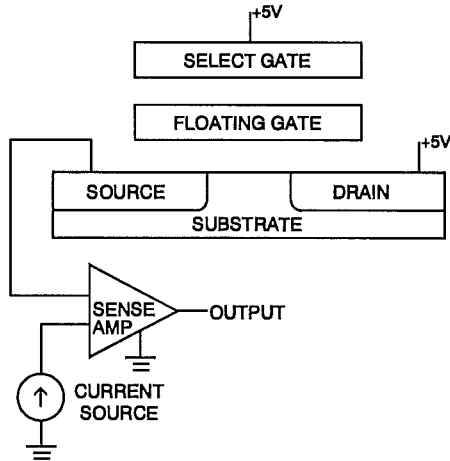
Figure 3.3: ETOX™ Flash Memory Cell Being Read
