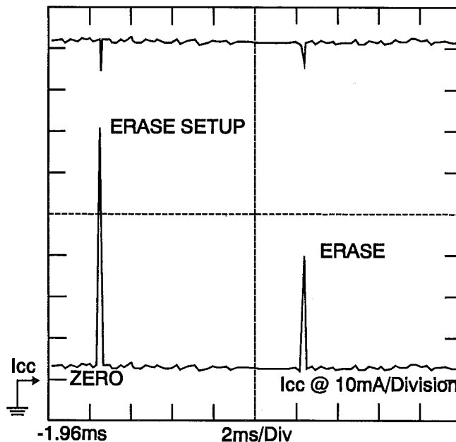
Figure 6.3: V_{CC} Current (Typical) - Erase Mode
