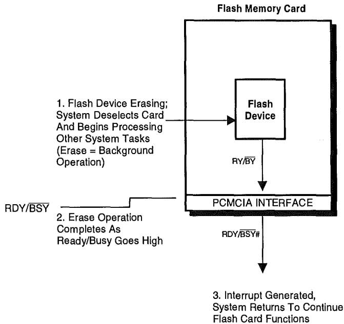
Figure 8.8: RDY/BSY Background Sequence
