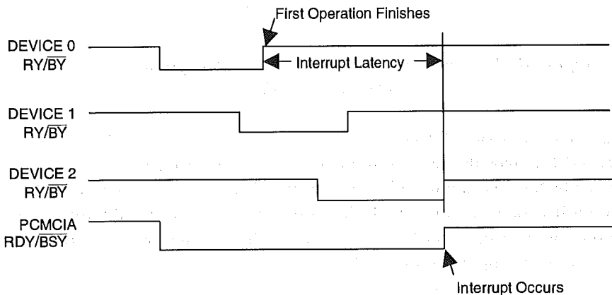
Figure 8.10: Standard PCMCIA RDY/ \overline{\text{BSY}} Waveform
