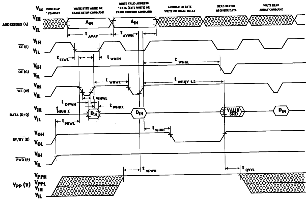
Figure 5.13: AC Waveforms for Write Operation
