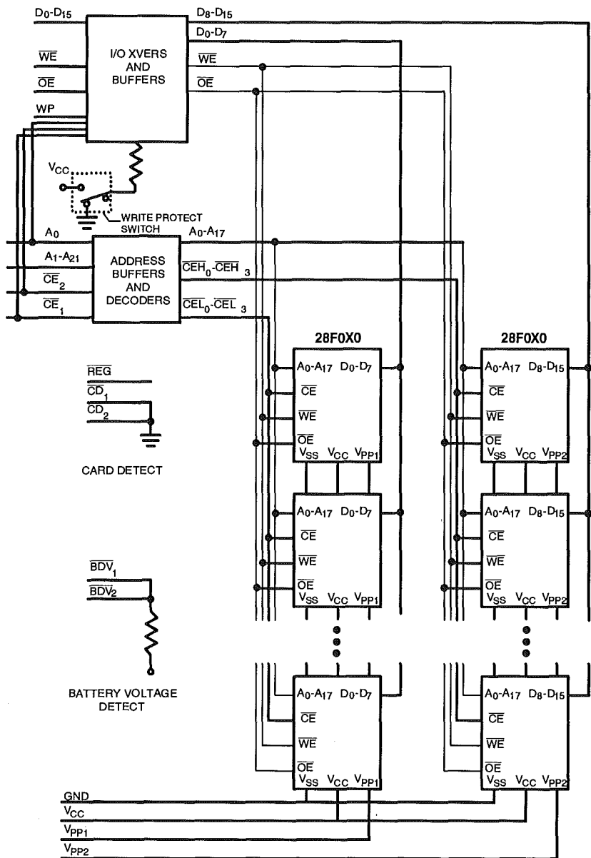
Figure 8.1: PCMCIA 1.0 Flash Memory Card
