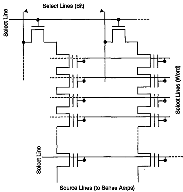
Figure 3.14: NAND Flash Memory Array Interconnect
