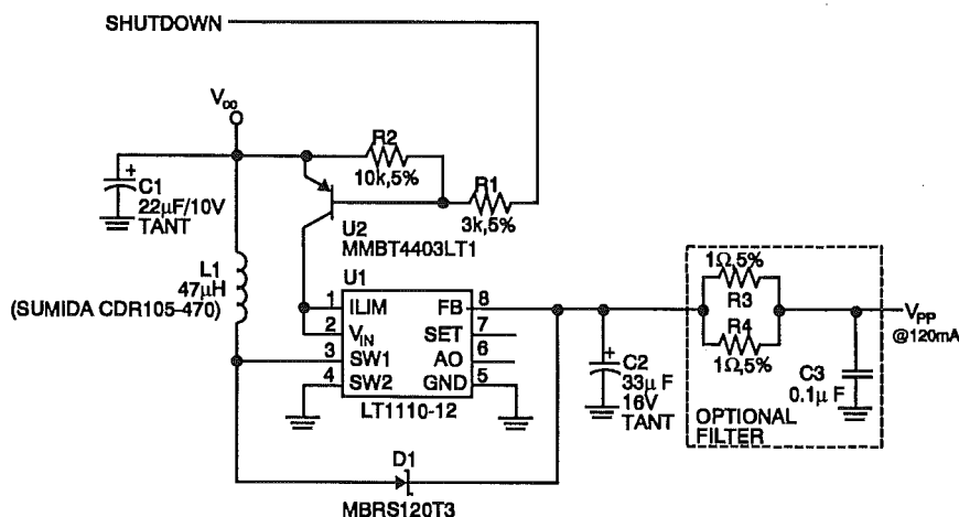
Figure 6.7: Linear Technology LT1110 5V to 12V Converter
