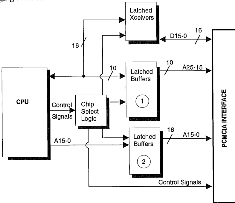
Figure 8.20: Memory Paging Circuitry
