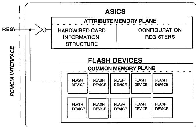
Figure 10.35: Select between a Flash Memory Card's Common and Attribute Memory Planes using the REG Signal
