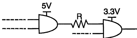
Figure 6.16: Interfacing a 5V Device to a 3.3V Device. Series Resistor Voltage Drop
