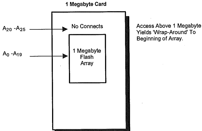
Figure 8.5: Aliasing Caused by Inadequate Address Line Decoding
