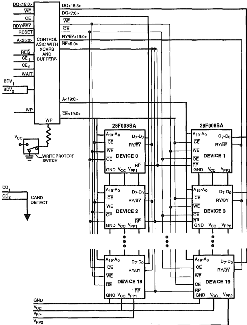
Figure 8.2: Intel Series 2 Flash Memory Card
