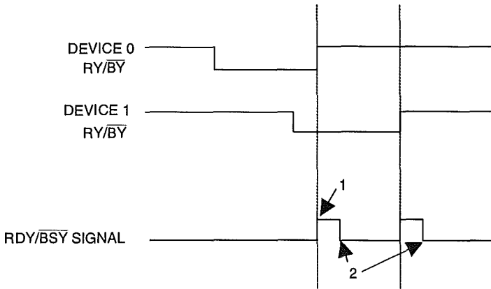
Figure 8.11: High-Performance \text{RDY}/\overline{\text{BSY}} Waveform for Multiple Device Operations
