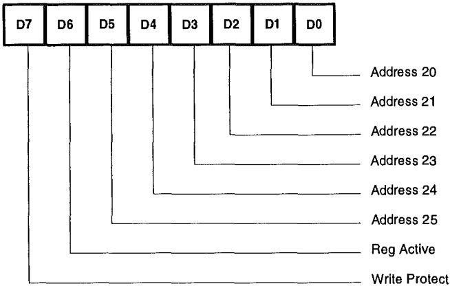
Figure 10.27: These PCIC Registers Set Up the Flash Memory Card's Offset, Enables Write Protection, and Selects the Memory Plane
