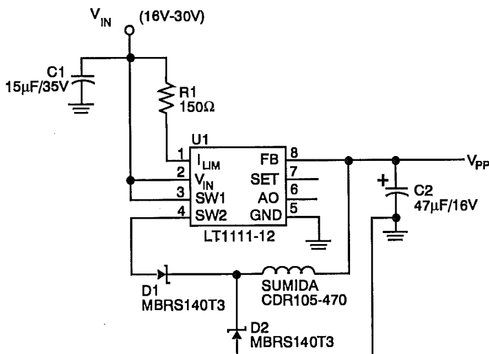
Figure 6.11: Linear Technology LT1111 Voltage Step Down Switcher
