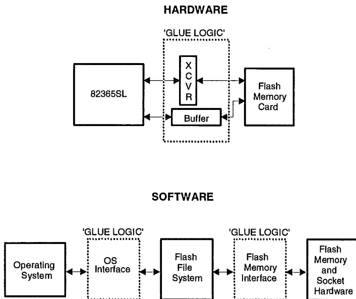
Figure 10.1: Glue Logic Holds Together the Major System Pieces
