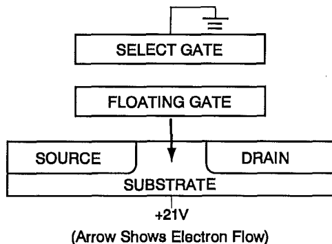
Figure 3.16: NAND Flash Memory Cell Being Erased
