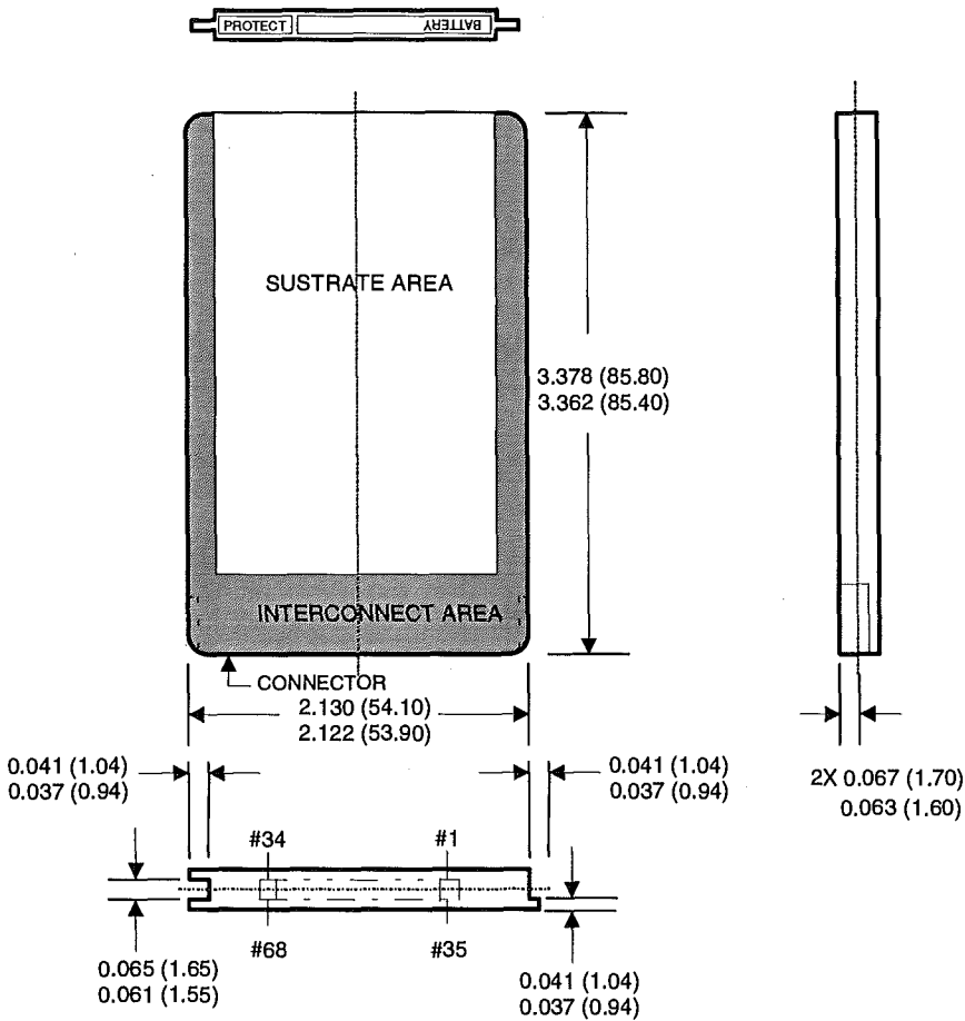
Figure 4.13: PCMCIA / JEIDA Type 2 PC Card Package Dimensions
