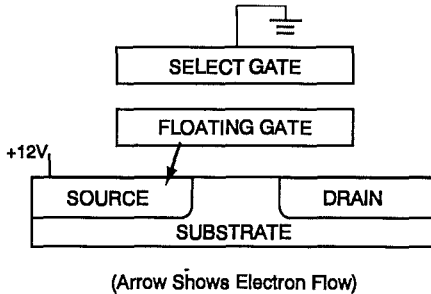
Figure 3.7: ETOX™ Flash Memory Cell Being Erased
