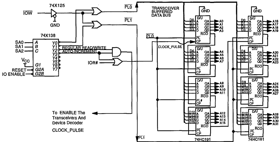
Figure 8.17: Counters Enhance I/O-Mapped Read Access
