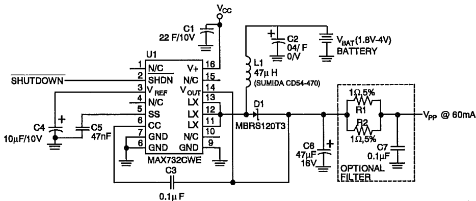
Figure 6.9: Maxim MAX732 3V to 12V Converter
