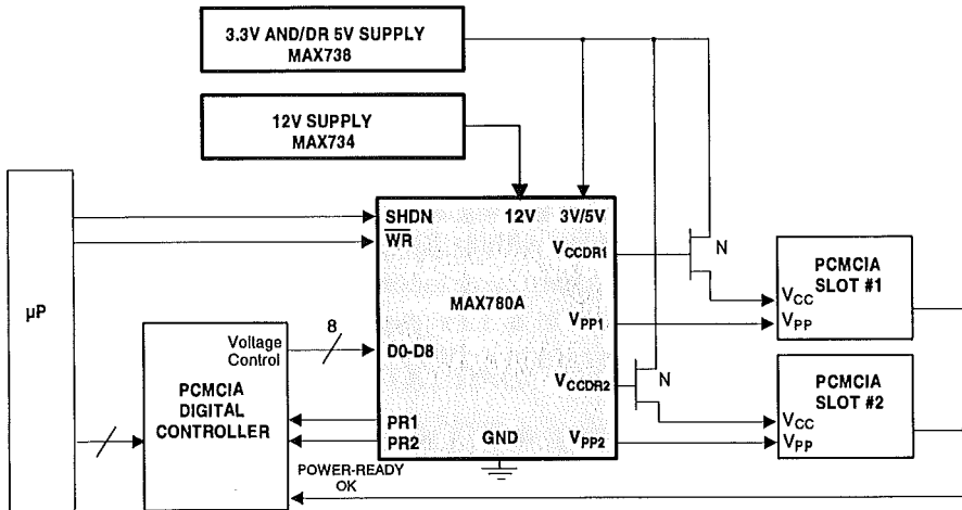
Figure 8.14: PCMCIA Controller Chip Controls Voltage Switching
