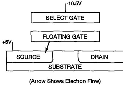
Figure 3.8: Negative Gate Erase
