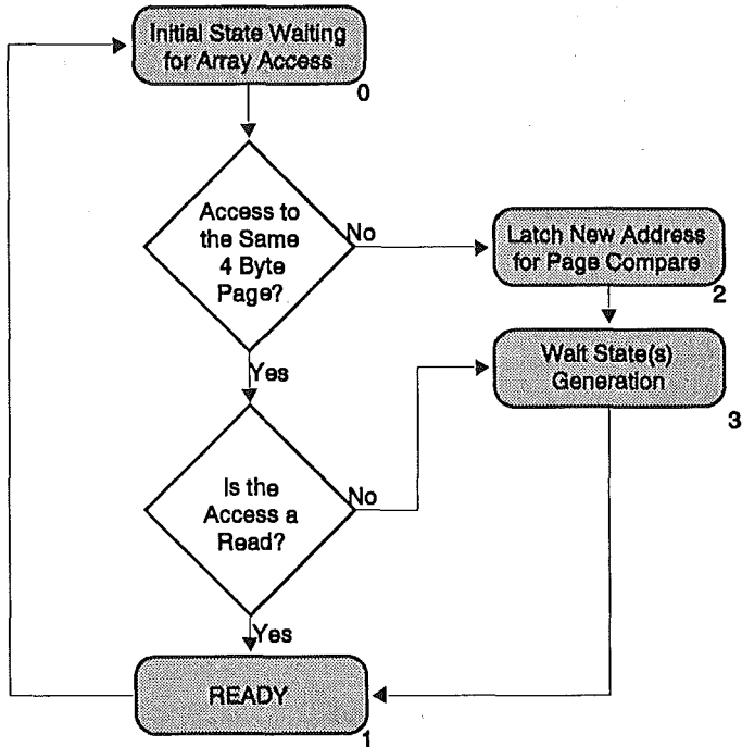
Figure 5.16: Hardware Interleaving - State Transition Diagram
