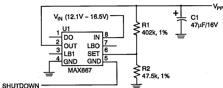
Figure 6.10: Maxim MAX667 12V Linear Voltage Regulator
