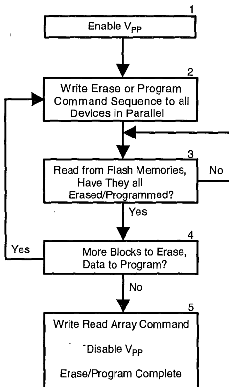
Figure 7.13: Parallel Program / Erase of Automated Flash Memories
