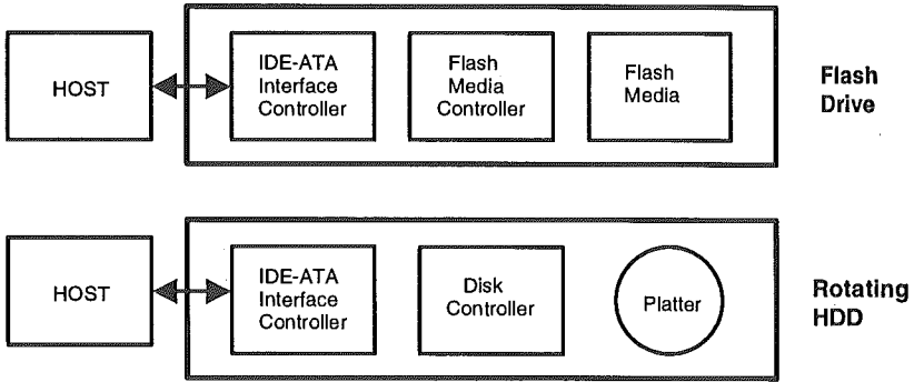
Figure 4.14: Mass Storage Architecture
