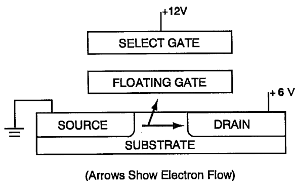
Figure 3.5: ETOX™ Flash Memory Cell Being Programmed
