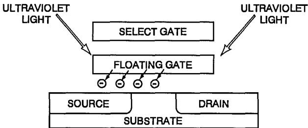
Figure 3.6: EPROM Cell Being UV Erased
