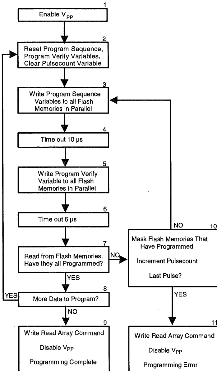
Figure 7.11: Parallel Programming of Non-Automated Flash Memories
