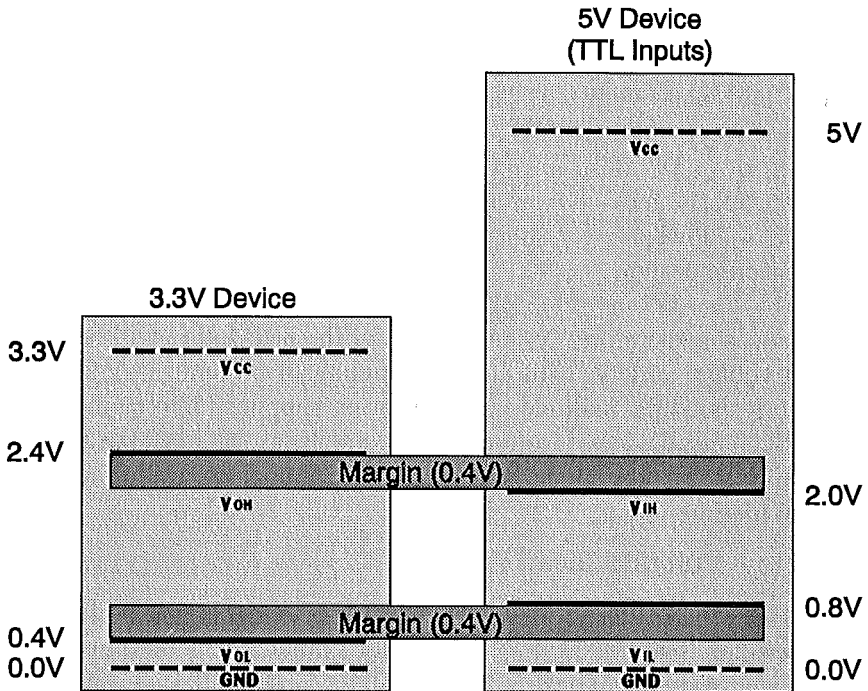
Figure 6.12: Interfacing a 3.3V Device to a 5V Device (TTL Inputs)
