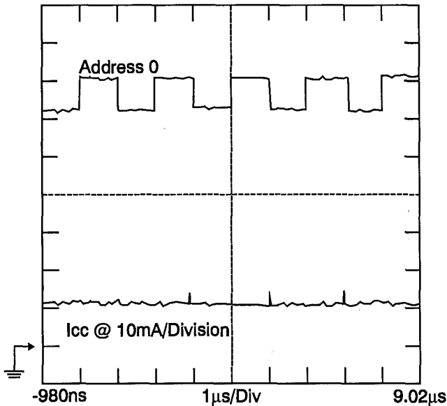
Figure 6.1: V_{CC} Current (Typical) - Read Mode
