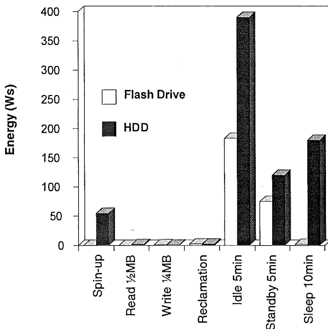
Figure 2.2: Energy Consumed During Various Activities
