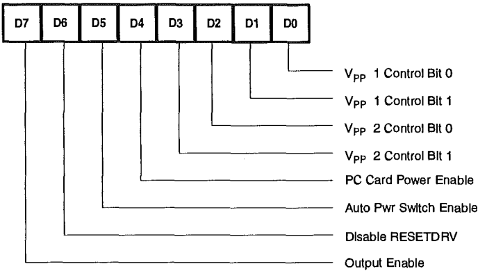
Figure 10.29: This PCIC Register, Power Control and RESETDRV, Controls a Socket's Voltage Levels
