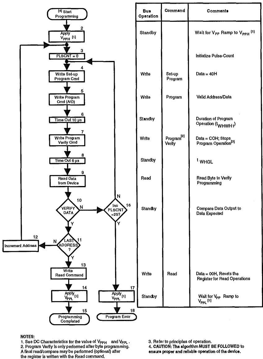
Figure 7.2: Intel First Generation Flash Memory Non-Automated Programming Algorithm
