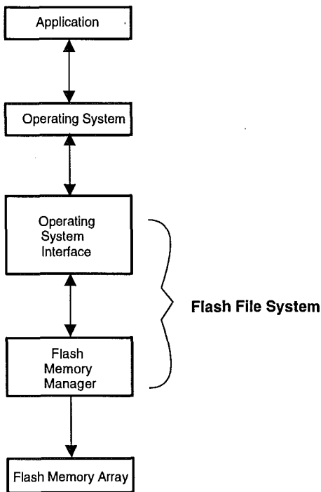
Figure 9.1: Flash Memory Manager and Operating System Interface
