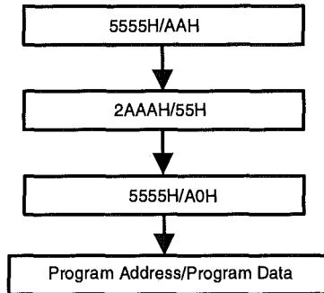
Figure 7.8: AMD "5V-Only" Automated Program Algorithm
