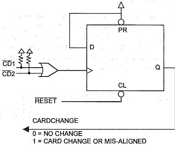
Figure 8.13: Example Card Detection Circuitry
