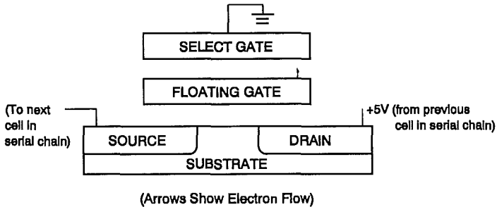
Figure 3.13: NAND Flash Memory Cell Being Read
