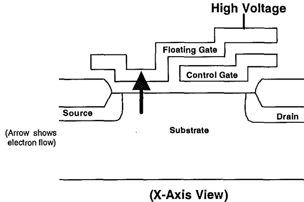
Figure 3.12: EEPROM-Based Flash Memory Cell Being Programmed
