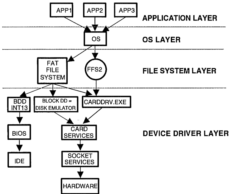
Figure 9.7: Flash Memory Solid-State Drive System Layers
