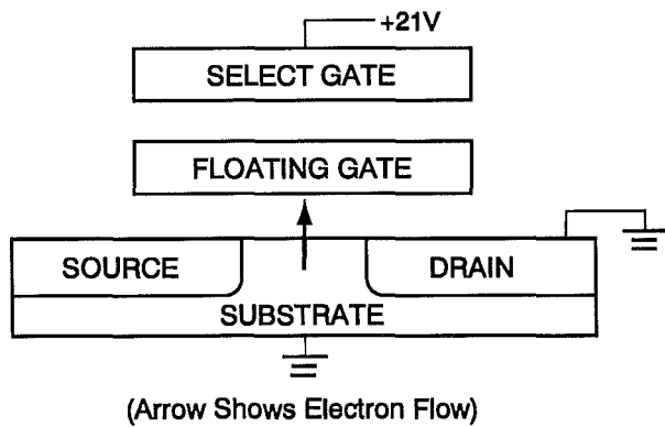
Figure 3.15: NAND Flash Memory Cell Being Programmed
