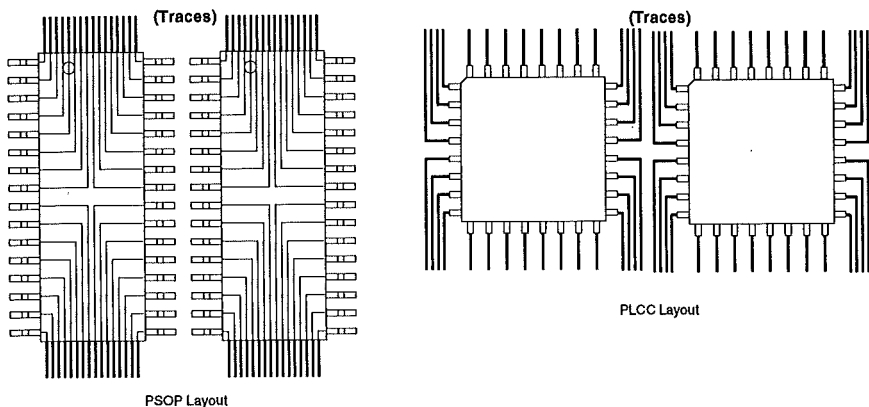
Figure 4.4: Trace Layout Comparison: PSOP vs. PLCC
