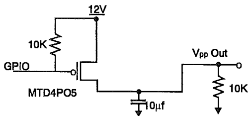
Figure 5.3: V_{PP} Switch Circuit
