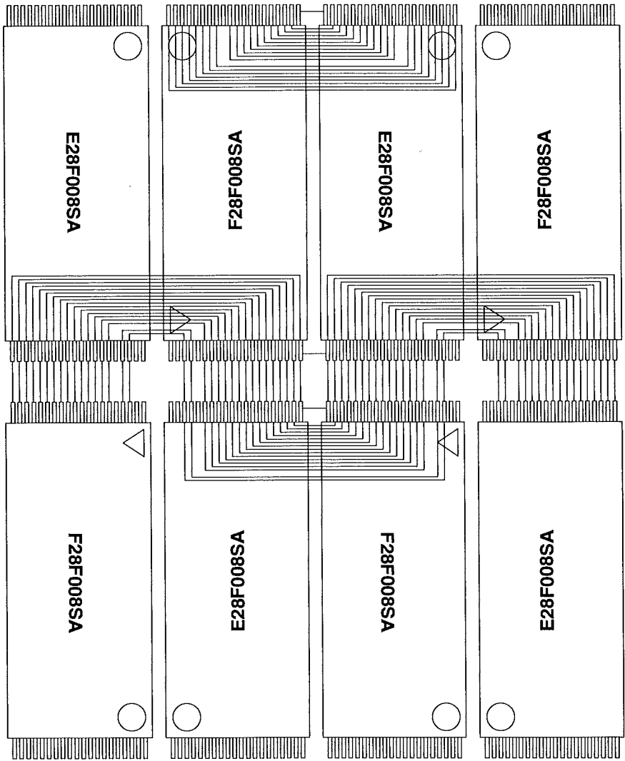
Figure 4.9: TSOP Serpentine Package Layout
