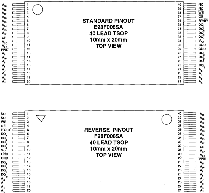
Figure 4.8: Standard and Reverse TSOP Packages
