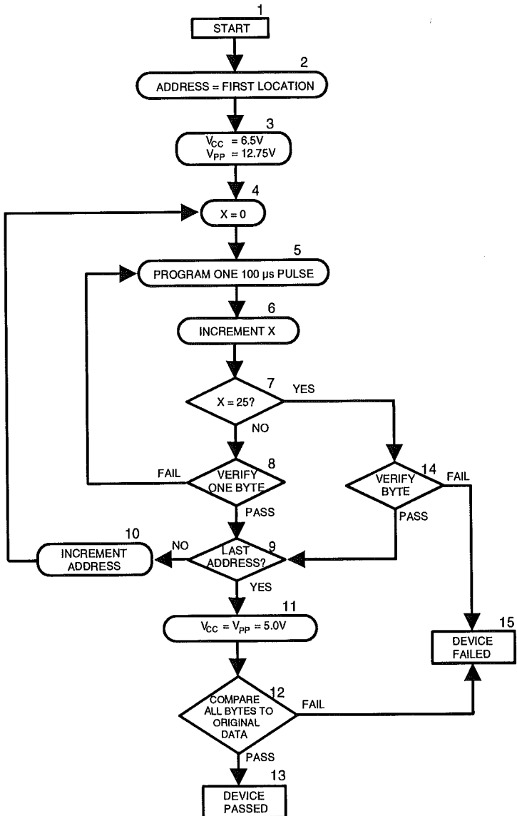
Figure 7.1: EPROM Programming Algorithm (Simplified Form)
