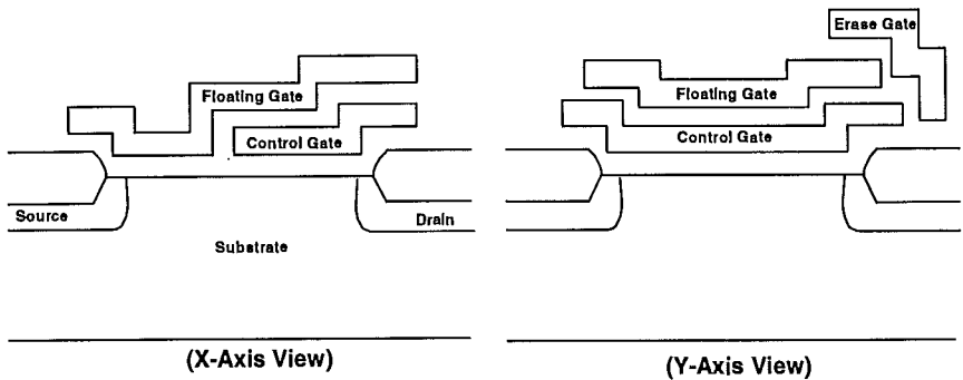
Figure 3.10: EEPROM-Based Flash Memory Cell
