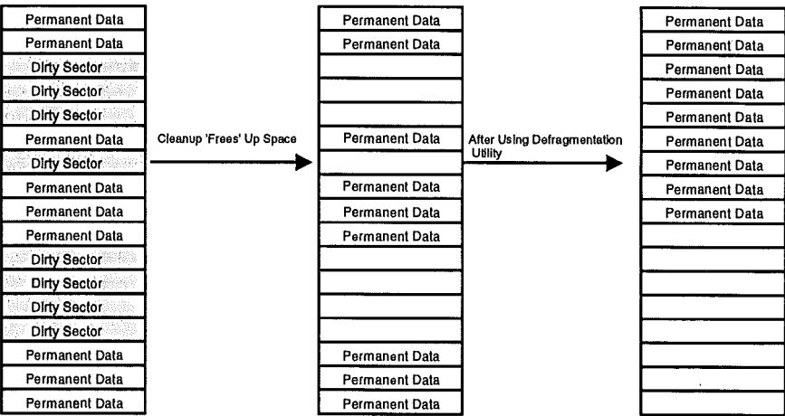
Figure 9.14: Defragmentation Utility Concatenates "Permanent Data"
