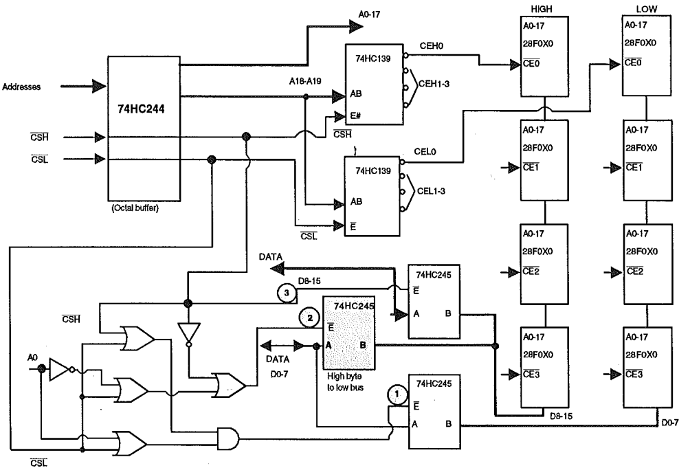
Figure 8.7: Byte-Wide Access Mode Circuitry for 8-Bit Systems
