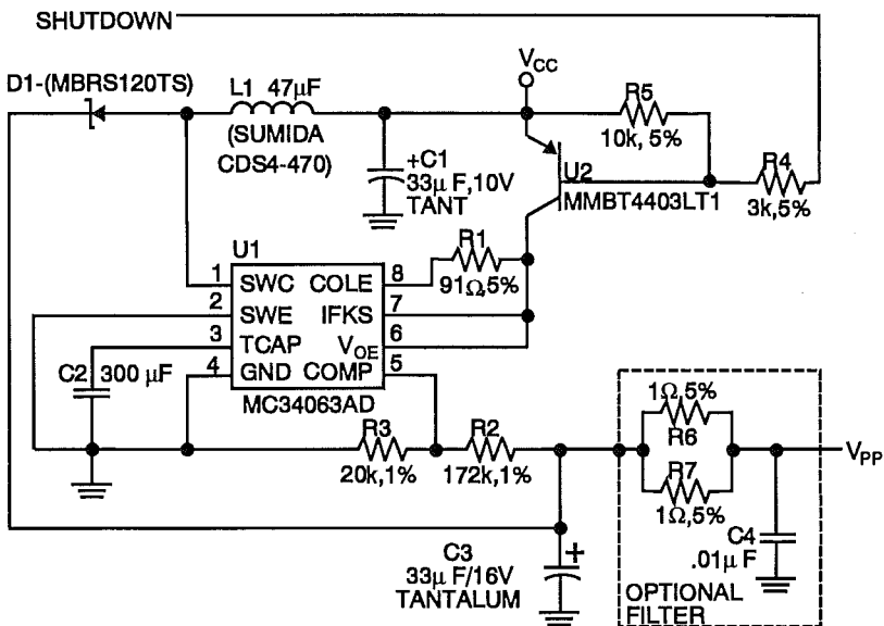
Figure 6.8: Motorola MC34063A 5V to 12V Converter
