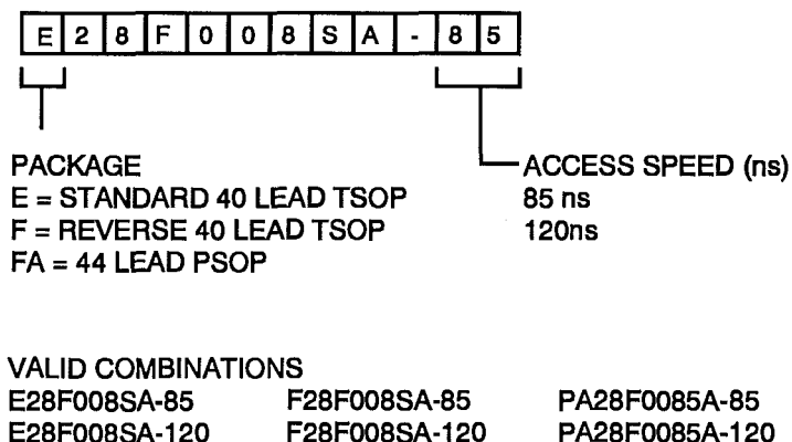
Figure 5.14: Example Ordering Information Table
