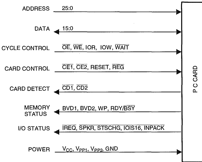
Figure 8.3: PCMCIA Electrical Interface Categories
