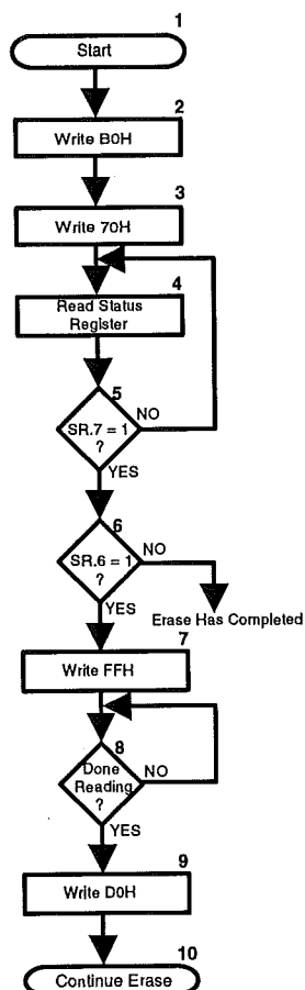
Figure 7.7: The Intel Automated Erase Suspend / Resume Algorithm
