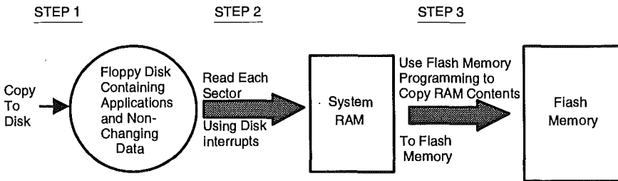
Figure 9.9: Creating a Disk Image in Flash Memory
