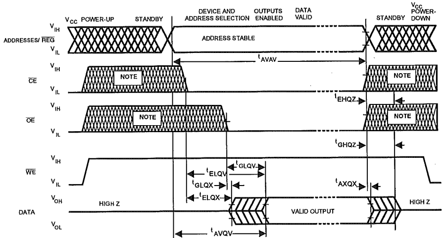
Figure 8.4: PCMCIA Read Timing Waveform
