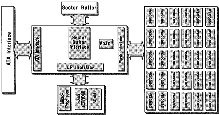
Figure 4.15: Flash Drive Architecture
