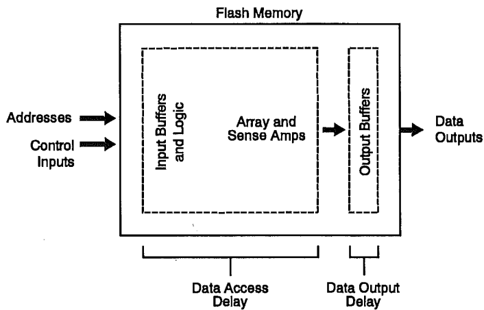
Figure 5.7: Flash Memory Read Access Time Partitioning
