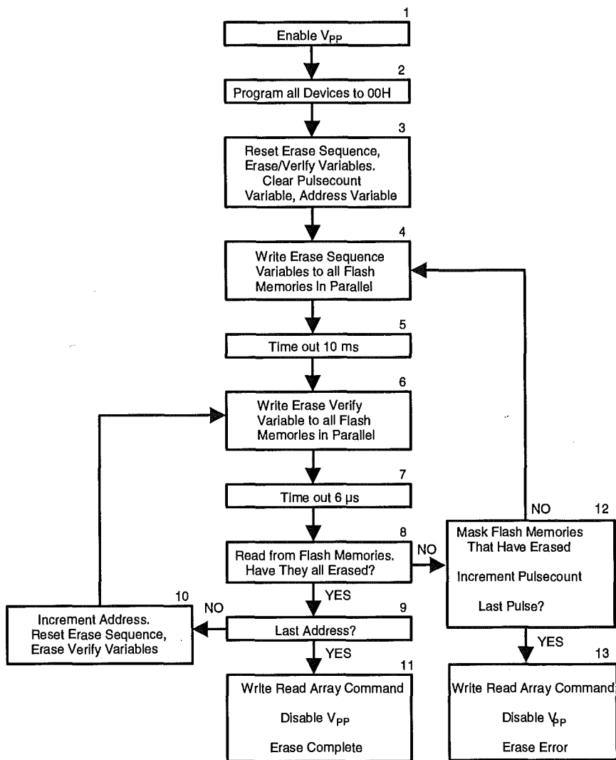
Figure 7.12: Parallel Erase of Non-Automated Flash Memories
