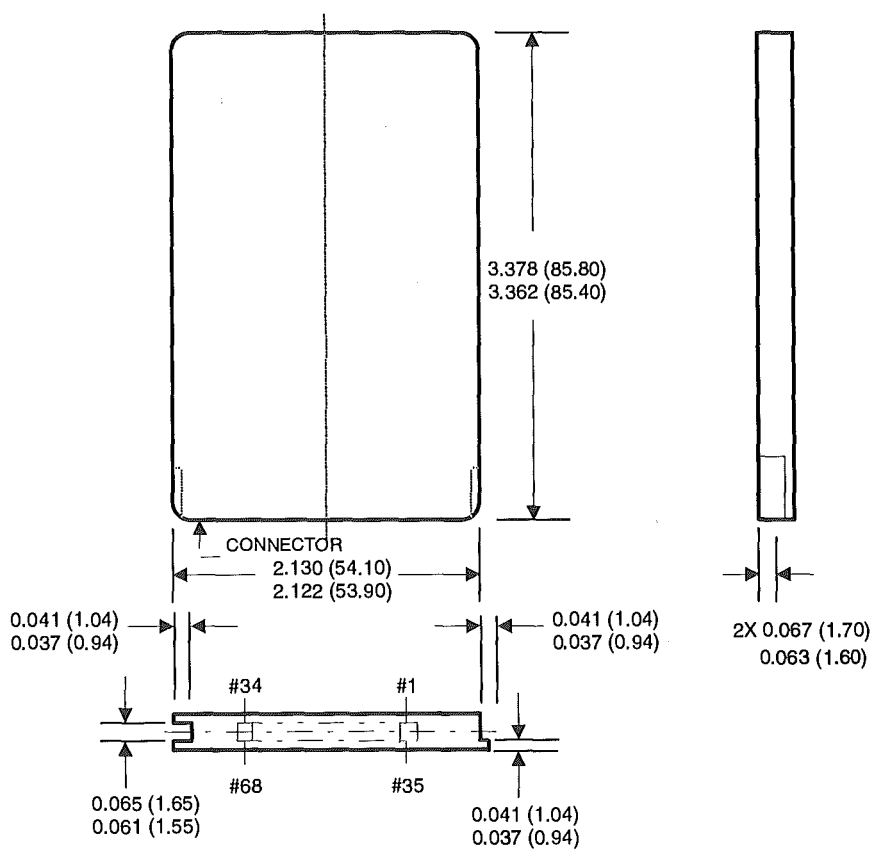
Figure 4.12: PCMCIA / JEIDA Type I PC Card Package Dimensions
