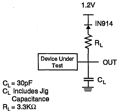
Figure 5.11: High Speed AC Testing Load Circuit
