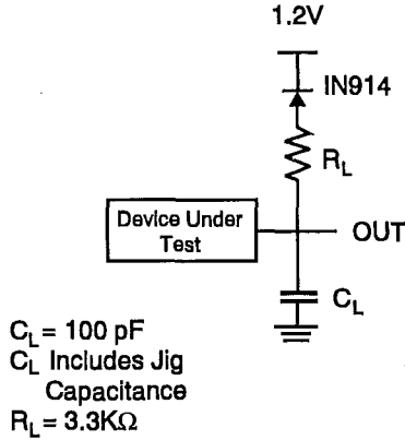
Figure 5.9: AC Testing Load Circuit
