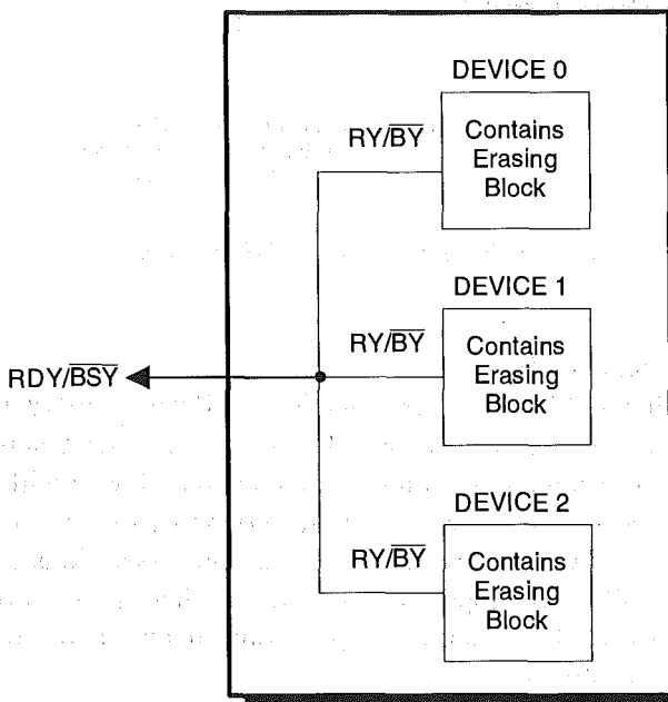
Flash Memory Card With Automated Devices
