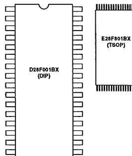
Figure 4.2: DIP / TSOP Package Comparison (Actual Size)
