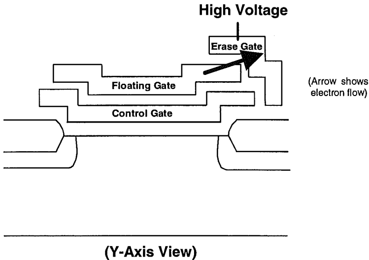
Figure 3.11: EEPROM-Based Flash Memory Cell Being Erased
