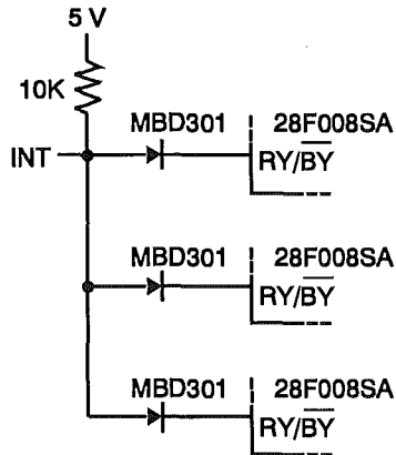
Figure 5.6: Wired-OR \overline{RY/BY} Implementation
