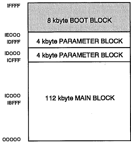
Figure 5.5: Intel 28F001BX Boot Block Flash Memory Map
