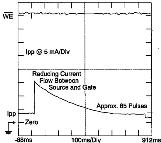
Figure 6.5: V_{PP} Current (Typical) - Erase Mode
