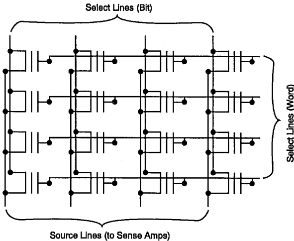
Figure 3.4: NOR Flash Memory Array Interconnect
