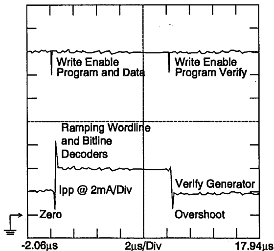
Figure 6.4: V_{PP} Current (Typical) - Program Mode
