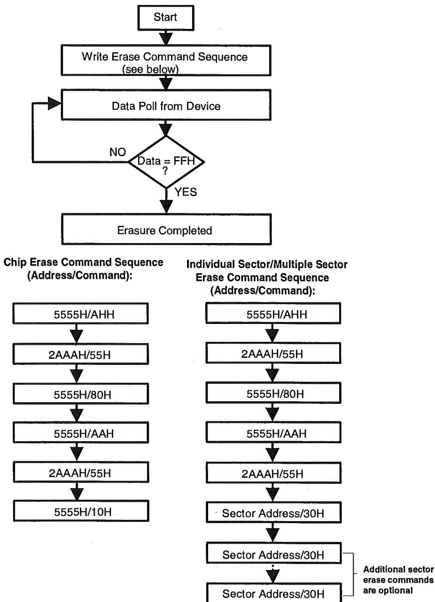
Figure 7.9: AMD "5V-Only" Automated Erase Algorithm
