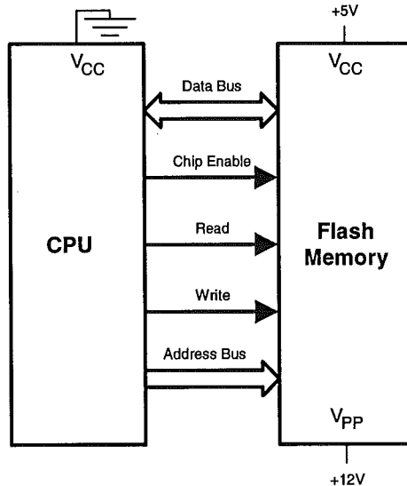
Figure 4.16: Design Considerations During On-Board Update
