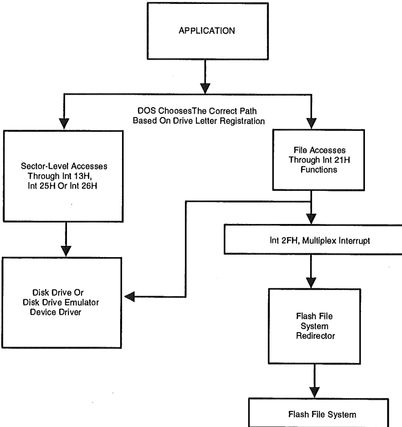
Figure 9.15: Flash Memory Solid-State Drive Accessing Methods
