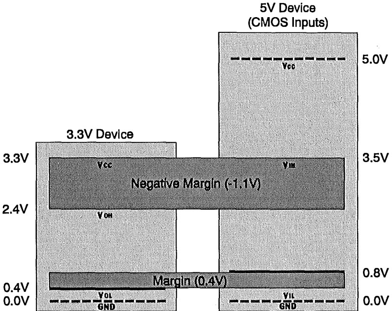
Figure 6.13: Interfacing a 3.3V Device to a 5V Device (CMOS Inputs)
