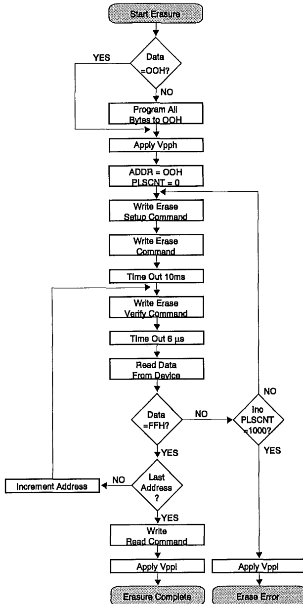
Figure 3.9: Iterative Basic Flash Memory Erase Algorithm
