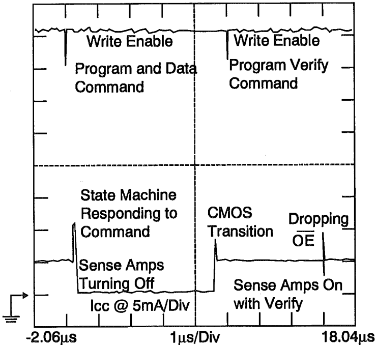
Figure 6.2: V_{CC} Current (Typical) - Program Mode
