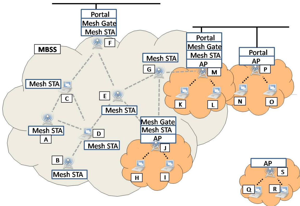
Figure 2: Mesh architecture components
