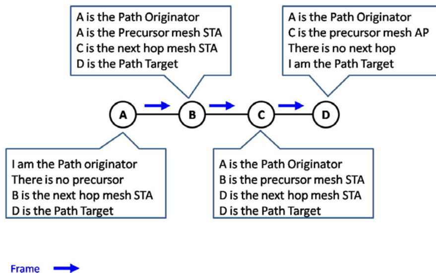
Figure 4: Terminology used with path determination
