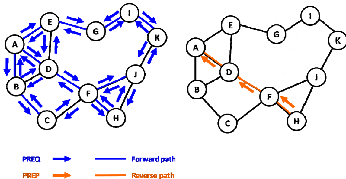
Figure 5: Using PREQ and PREP for mesh path selection
