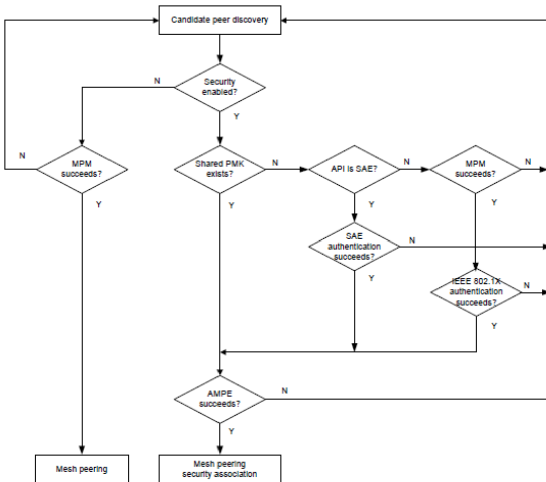
Figure 3: Mesh peering and security flowchart
