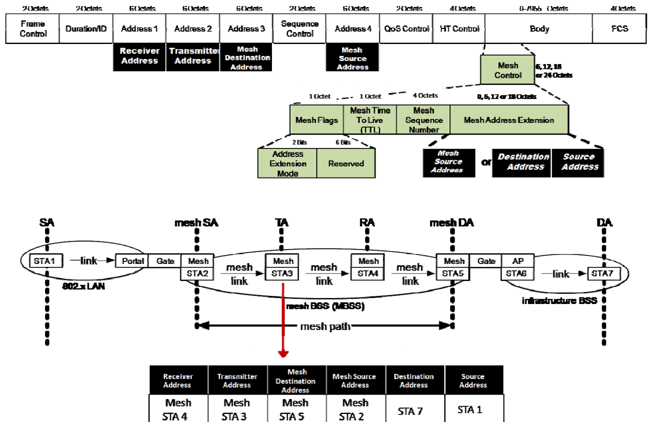
Figure 6: Addressing and the mesh frame format
