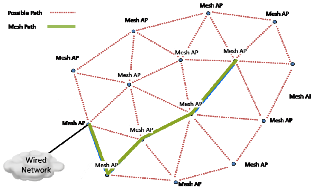
Figure 1: Basic mesh topology
