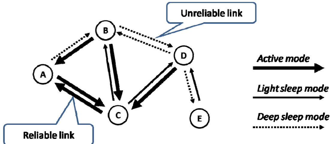
Figure 7: Example mesh power save scenario
