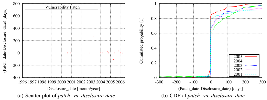
Figure 5: Patch-date vs. Disclosure-date
