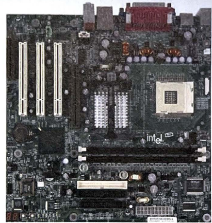
Figure 1-13 A typical motherboard.
