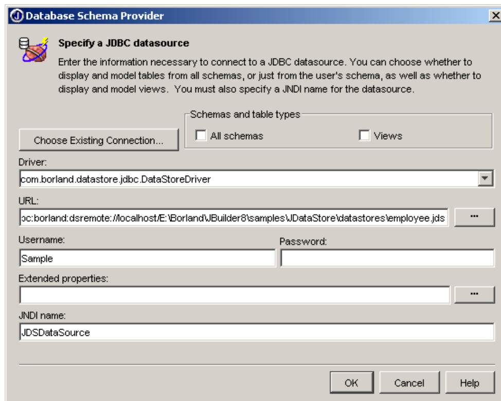
Figure 15: JBuilder Database Schema Provider—to create entity beans from database schema
