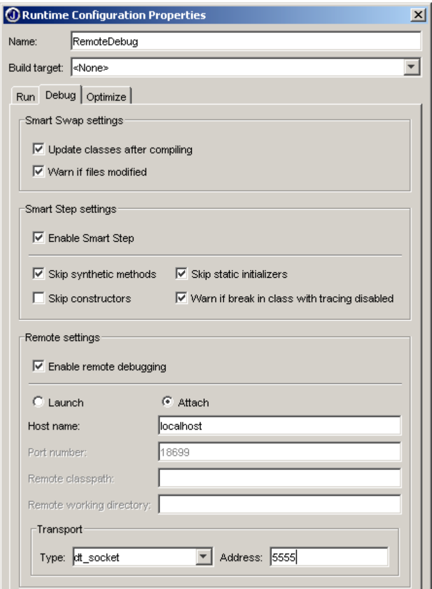
Figure 23: Runtime Configuration Properties window with remote debug parameters to remote debug EJBs
