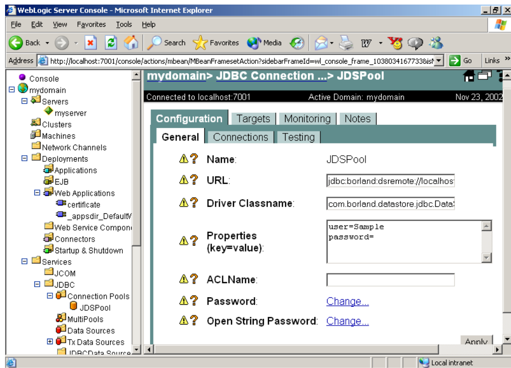
Figure 18: WebLogic console showing the connection pool JDSPool
