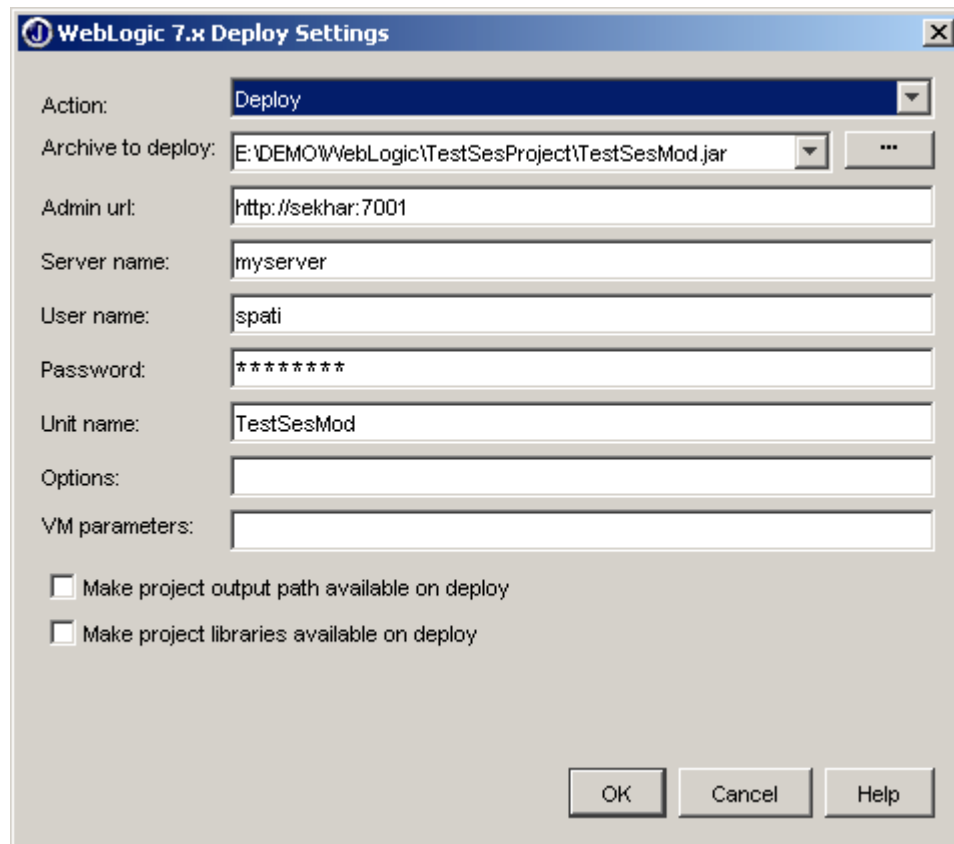
Figure 8: WebLogic 7.x Deploy Settings window for deploying to Remote WebLogic Server
