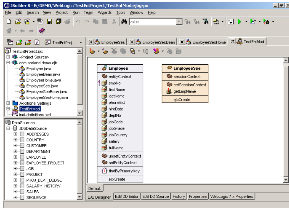
Figure 16: Visual EJBs in JBuilder displaying the fields and methods of entity and session beans
