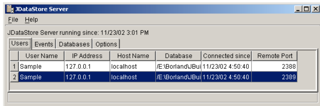
Figure 20: JDataStore server displaying two connections opened by WebLogic 7.0
