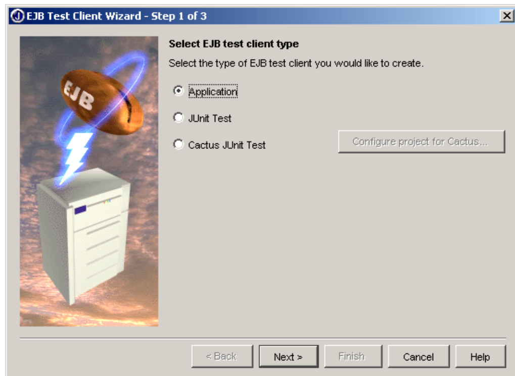
Figure 9: EJB Test Client Wizard: creating a test client for session bean TestSes
