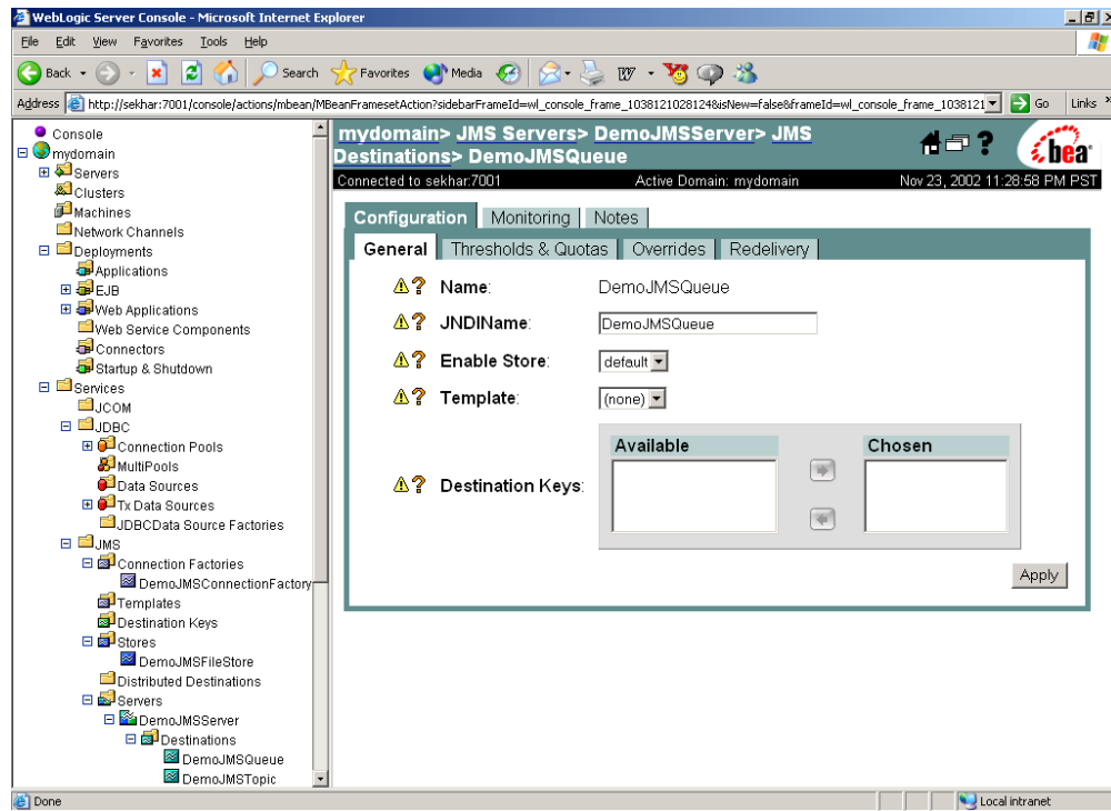
Figure 30: Creating a JMS Server using WebLogic Server Console
