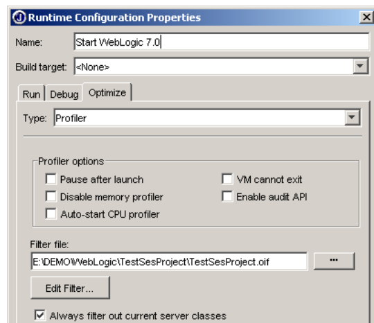
Figure 11: Runtime configuration window allows to choose which Optimizeit tool to use
