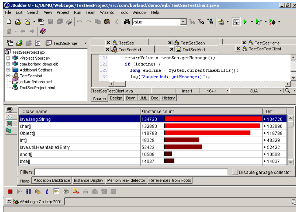
Figure 12: Optimizeit Profiler attached to WebLogic 7.x within JBuilder 8
