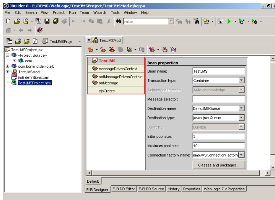
Figure 31: JBuilder created a MDB visually and provided a GUI to configure the MDB
