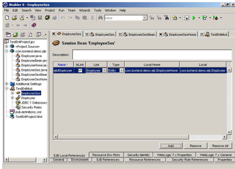
Figure 17: Creating an EJB Reference visually using JBuilder deployment descriptor editor tool
