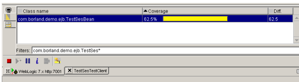
Figure 14: Optimizeit Code Coverage tool started in JBuilder 8 and attached with WebLogic Server 7.x
