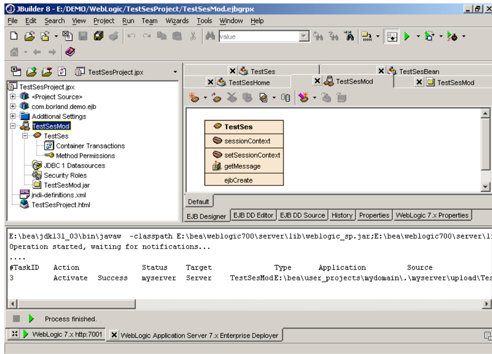
Figure 6: JBuilder displaying the deployment status of JAR file in a separate tab
