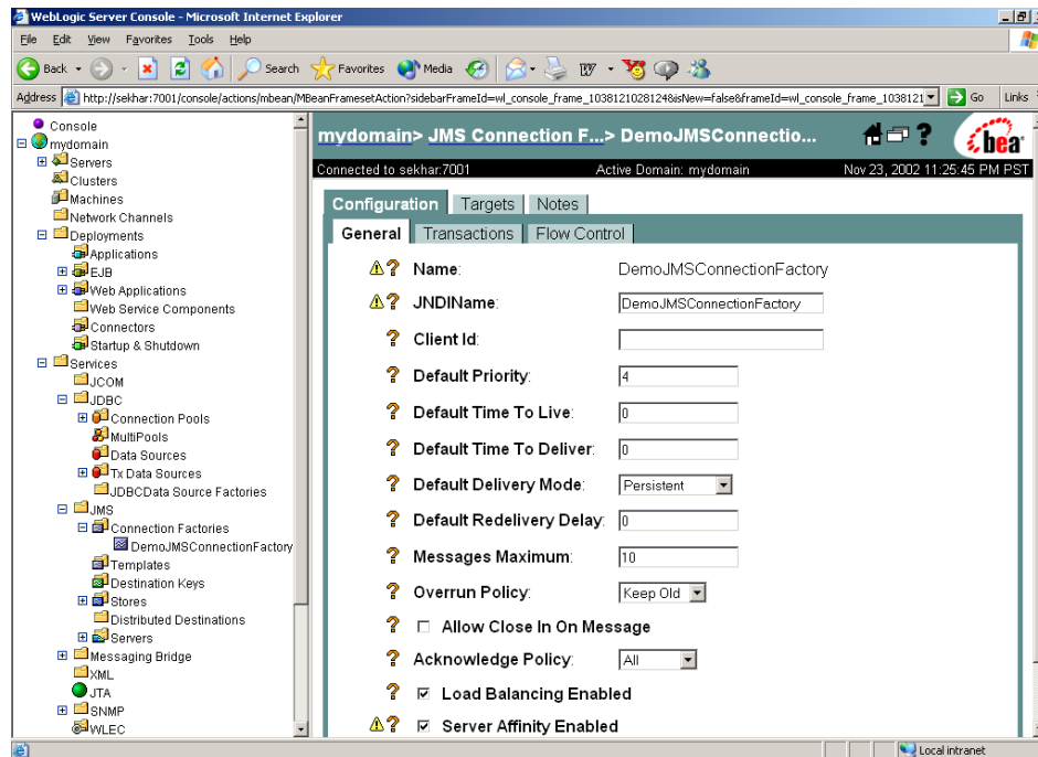
Figure 27: Creating a JMS Connection Factory using WebLogic Server Console
