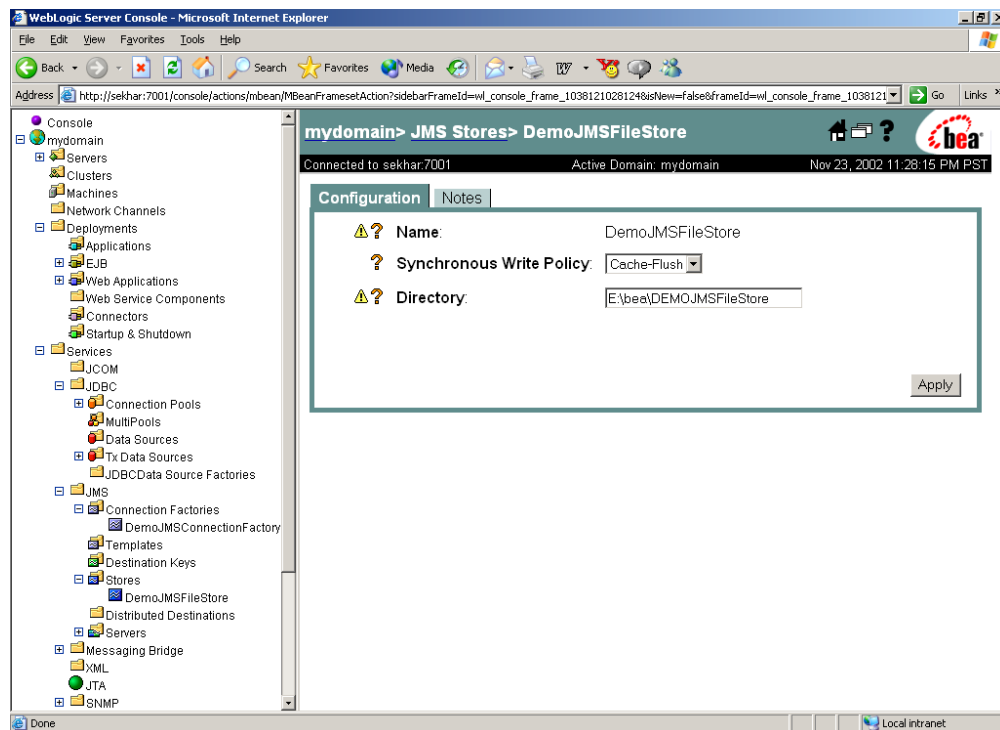
Figure 28: Creating a JMS File Store using WebLogic Server Console
