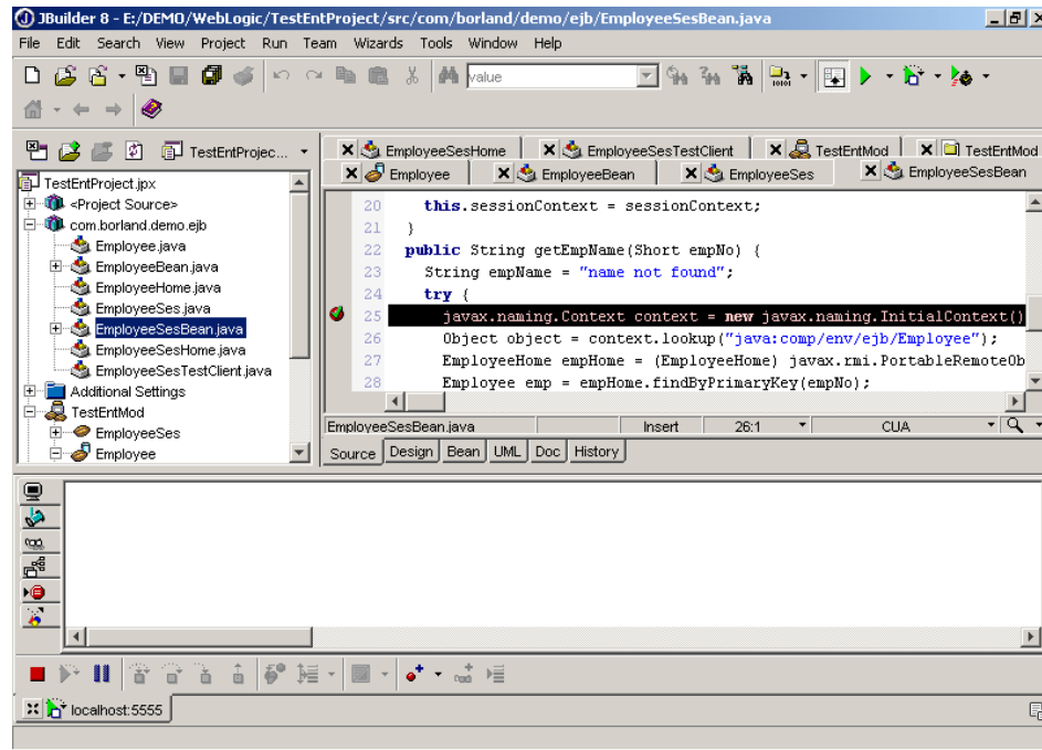
Figure 25: JBuilder opened a connection to remote WebLogic Server
