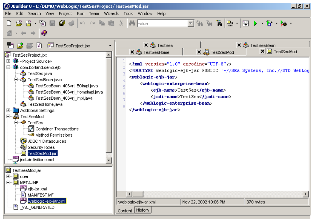
Figure 4: JBuilder has created the container generated files and WebLogic deployment descriptors
