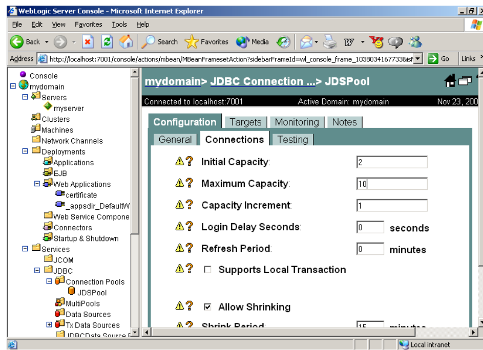
Figure 19: WebLogic Console; specifying the connection parameters for the connection pool
