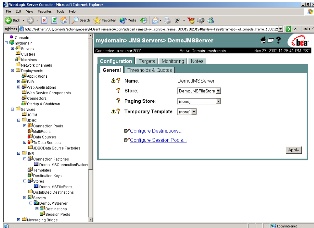
Figure 29: Creating a JMS Server using WebLogic Server Console
