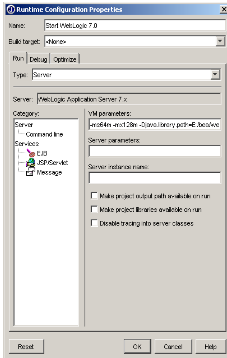
Figure 3: Runtime configuration to run WebLogic within JBuilder
