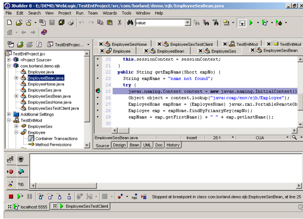
Figure 26: JBuilder remotely debugging running EJBs. Debugger stopped at the breakpoint
