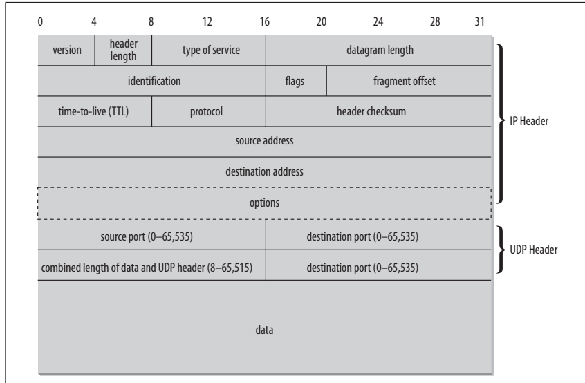
Figure 13-1. The structure of a UDP datagram
