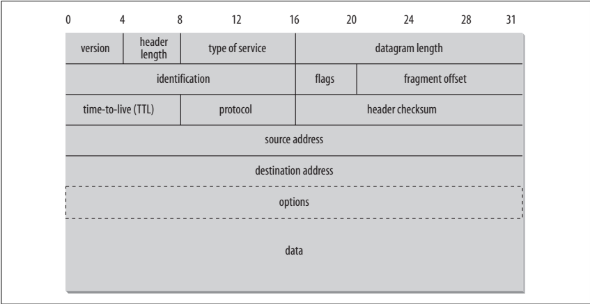
Figure 2-2. The structure of an IPv4 datagram
