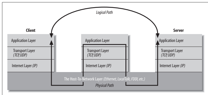
Figure 2-3. Layered connections through a proxy server
