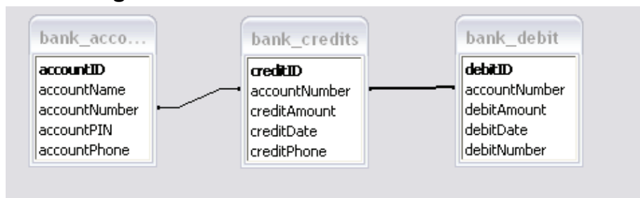
Figure 2: Tables for SMS Banking
