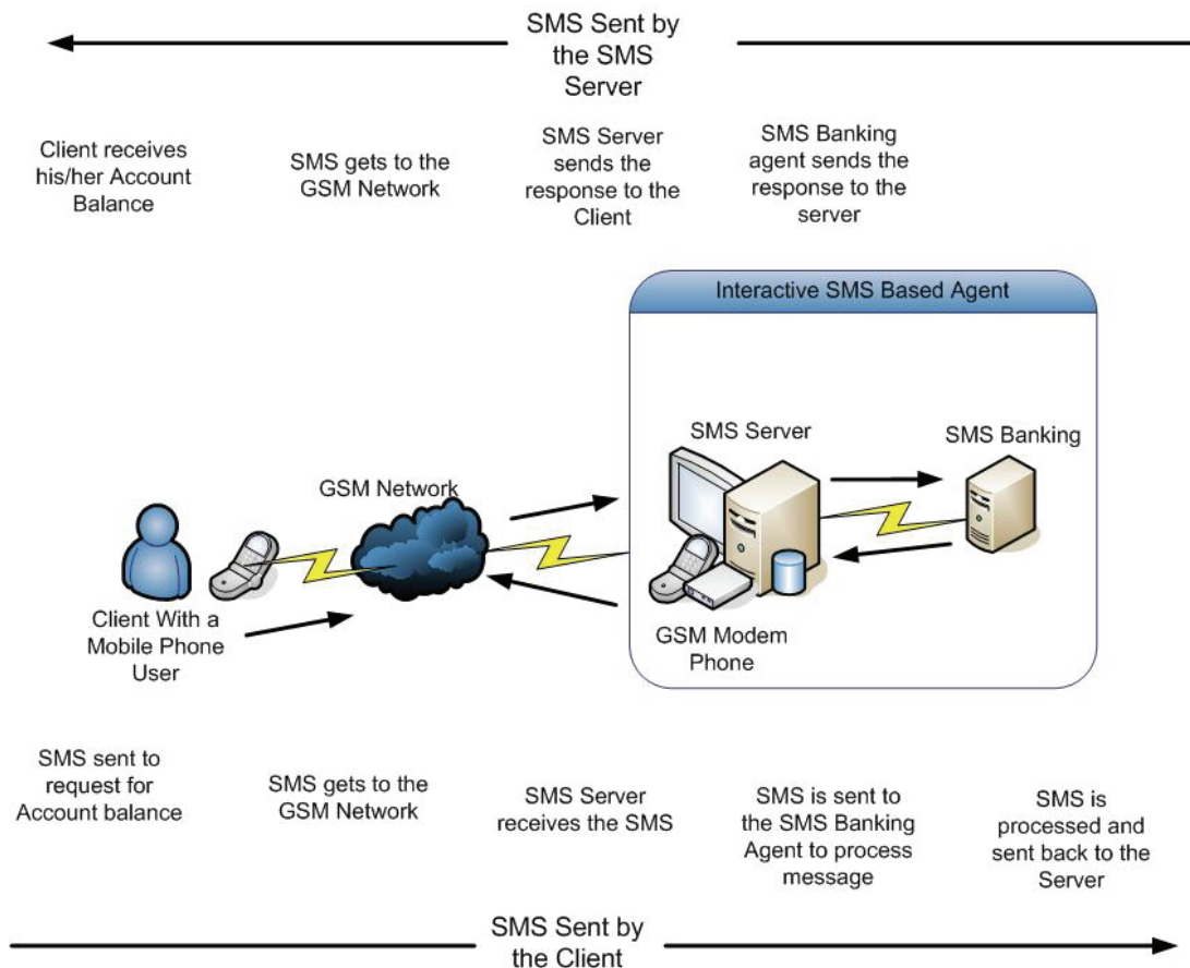
Figure 1: Hardware Architecture Design
