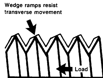
Figure 1.—Spiralock thread.
