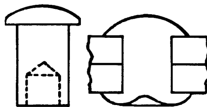
Figure 40.—Semitubular rivet. (From ref. 5.)
