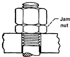
Figure 7.—Jam nut.
