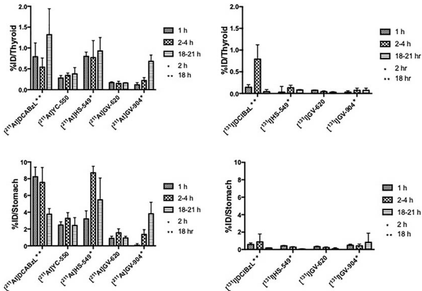
Figure 5. Percentage of the injected dose of ^{211}\text{At} and ^{131}\text{I} activity present in the thyroid and the stomach after injection of ^{211}\text{At} - and ^{131}\text{I} -labeled PSMA inhibitors.
