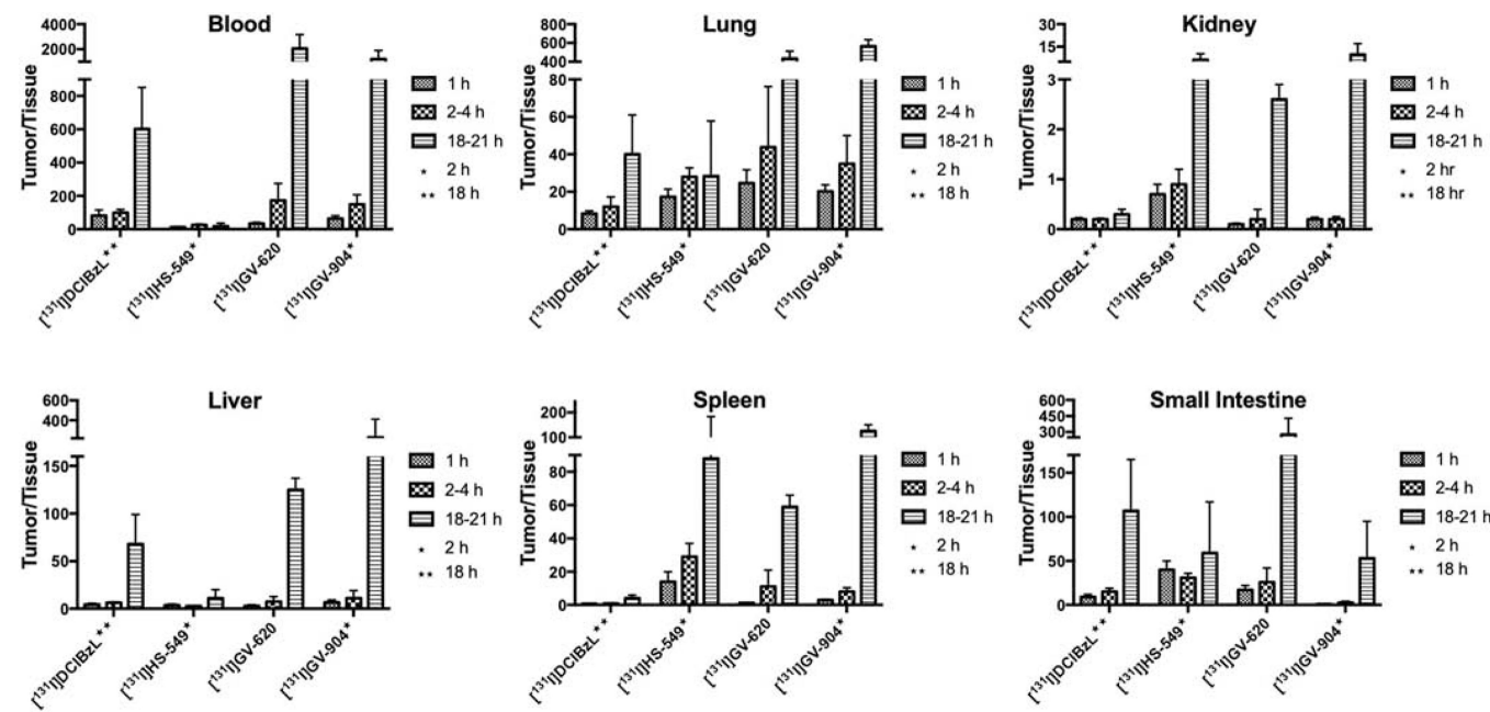
Figure 7. PSMA+ PC3 PIP tumor-to-normal tissue ratios of ^{131}\text{I} activity after injection of ^{131}\text{I} -labeled PSMA inhibitors.
