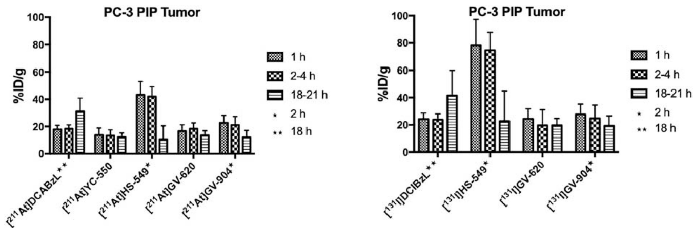
Figure 2. Uptake of 211 At and 131 I activity after injection of 211 At- and 131 I-labeled PSMA inhibitors in subcutaneous PSMA+ PC3 PIP subcutaneous xenografts.
