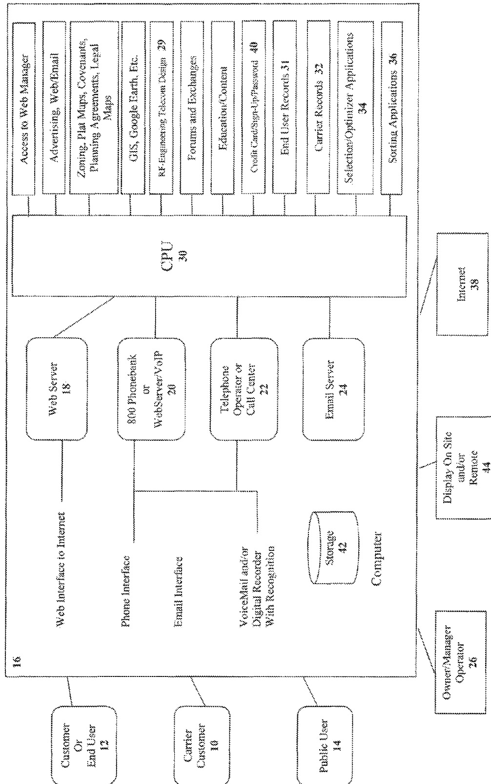
Fig. 1 Clearinghouse System
