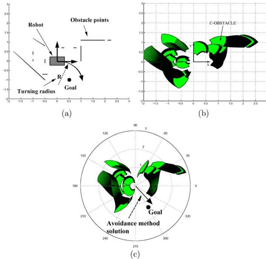
Figure 11. Iteration of the obstacle avoidance process. A sensory description of the obstacles (a) is used to compute the region of the configuration space in collision with the robot (rectangular shape) over the manifold of circular paths, (b), where the robot is represented by a point. The coordinates of the manifold are changed (c) so that the motion is free of kinematic constraints and the robot is a point. Here we use the avoidance method that computes the best motion direction “Avoidance method solution”, which represents an arc of circle in the workspace [“Turning radius” in figure (a)].
