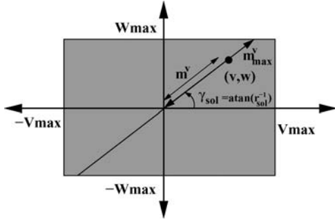
Figure 10. This figure shows how to compute the motion command (v, w) within the physical limits (maximum velocities v_{\max} and w_{\max} ) given a turning radius r_{\text{sol}} . The module of the speed vector m^v is reduced linearly with the distance to the closest obstacle (when there are obstacles closer than a given distance to the robot).
