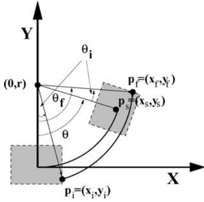
Figure 4. This figure shows how the motion over a circle leads a point of the robot boundary (x_i, y_i) to the obstacle point (x_f, y_f) , in the robot system of reference. The robot location (x_s, y_s) represents the limit between collision and no collision, that is, the boundary of C-Obstacle.
