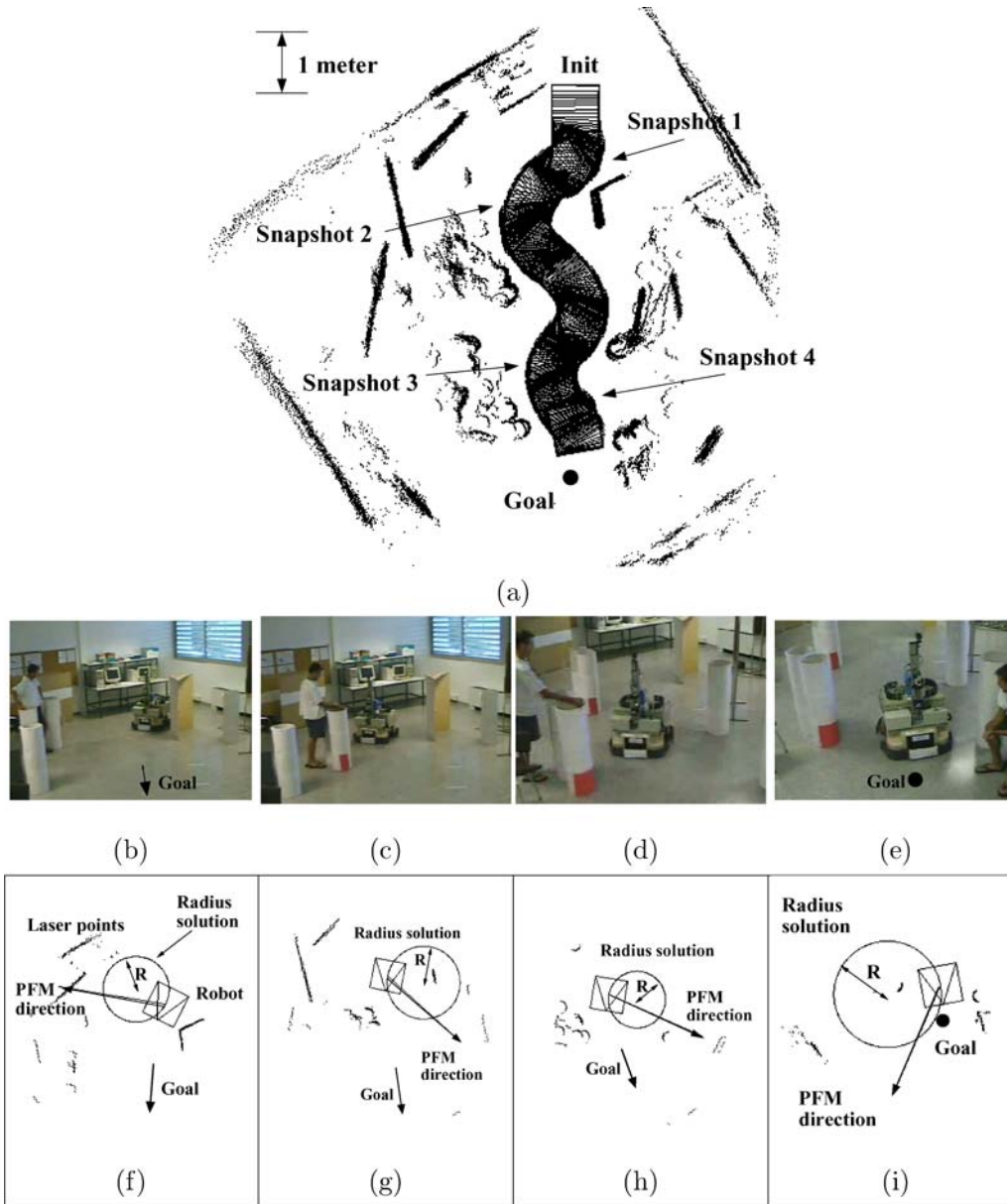
Figure 13. Experiment with the PFM method using the abstraction layer to take into account the shape and kinematics constraints. (a) Path executed by the vehicle and laser points collected in the experiment. (b)–(e) Some snapshots that correspond to Figs. (f)–(i) showing the laser measurement used, the robot location, the radius solution using PFM in the ARM^P and the direction that would be obtained by PFM without using the abstraction.
