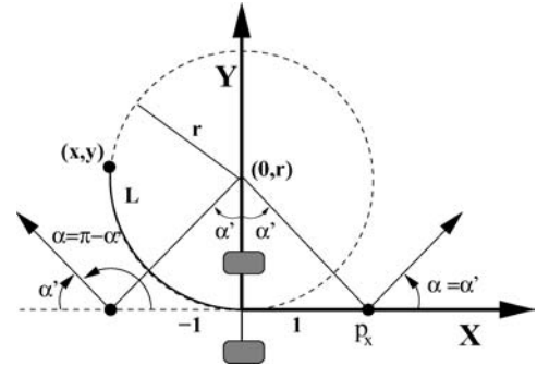
Figure 8. This figure shows how, where the point is located in the positive X-axis, the value of \alpha is \alpha' . If the point is in the negative axis, the problem is symmetrical with respect to the Y-axis.
