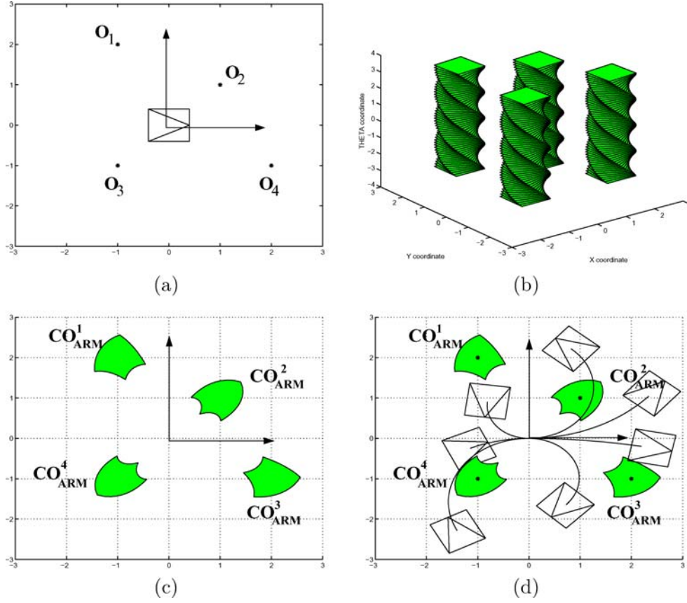
Figure 6. This figure shows the computation of the free space for a rectangular robot that moves over circular paths. (a) Robot and obstacles O_i ; (b) the C-Obstacles in the configuration space that result from the four obstacle points. These volumes contain all the configurations in collision with the obstacles; (c) each obstacle point creates a region of collision locations CO_{ARM}^i that all together are CO_{ARM} . The free space is the space outside these regions. Graphically, these regions are the inter-section between the volumes in (b) and the surface of figure 3(b). (d) Superposition of both the workspace and the ARM, and some robot locations and the paths that lead to them.
