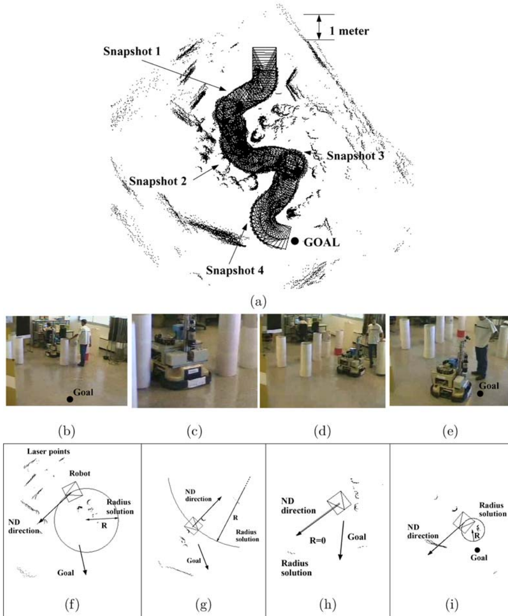
Figure 15. Experiment with the ND method using the abstraction layer to take into account the shape and kinematic constraints. (a) Path executed by the vehicle and laser points collected in the experiment. (b)–(e) Some snapshots that correspond to Figs. (f)–(i) showing the laser measurement used at that moment, the robot location, the radius solution using the ND in the ARM^P and the direction obtained by the ND without using the abstraction.
