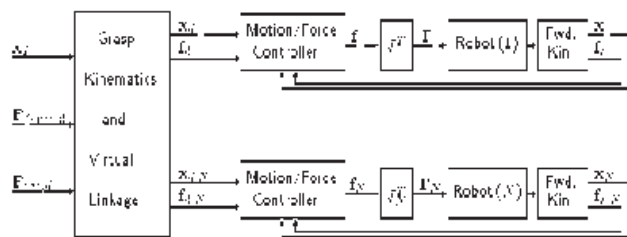
Fig. 5. Decentralized Control Structure
