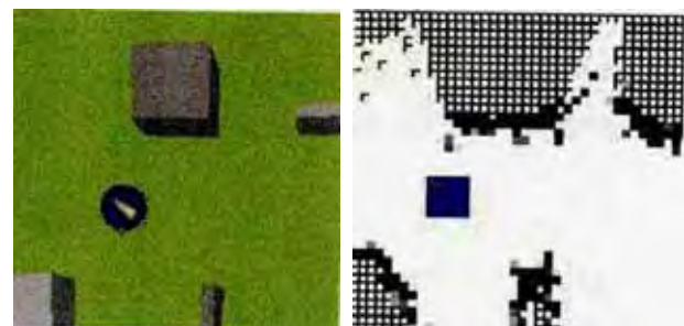
(a) A robot environment with a robot inside it (b) Incrementally constructed histogram grid-based map
