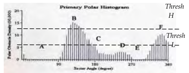
d) Polar histogram and the two threshold parameters
