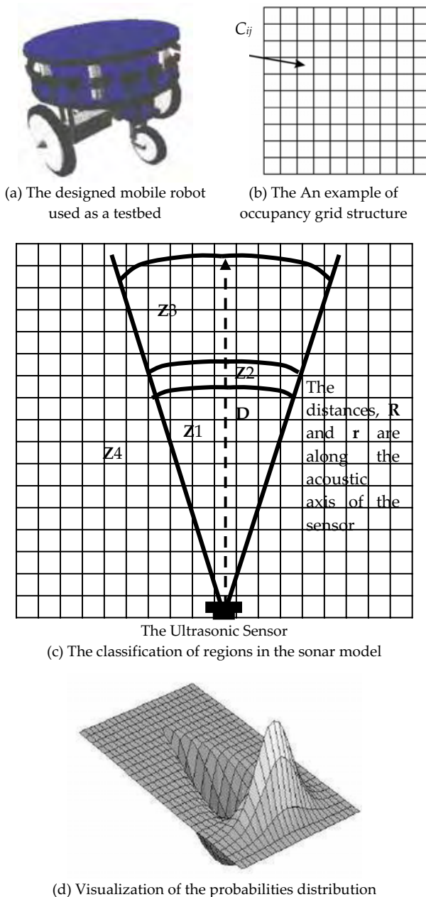
Fig. 1. shows the model of the designed mobile robot and the regions in the sonar model
