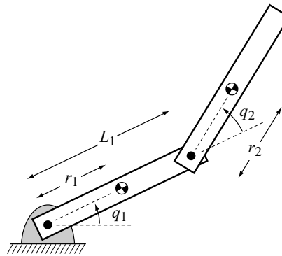
Figure 12.35 A 2R robot arm.
