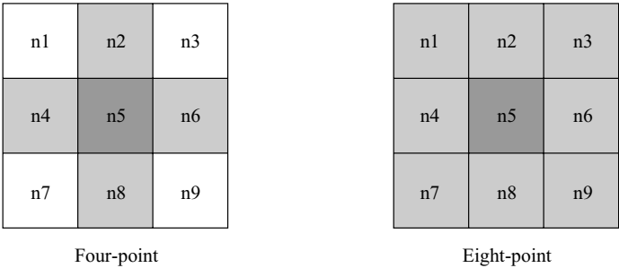
Figure 4.8 Four-point vs. eight-point connectivity.
