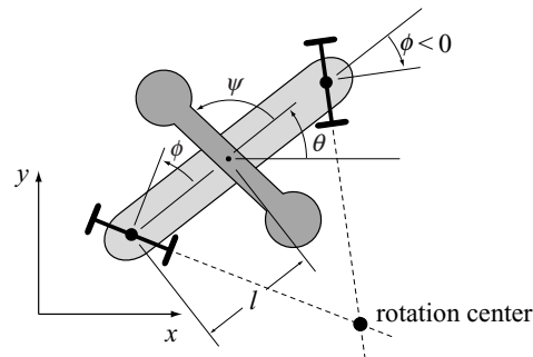
Figure 12.36 The snakeboard model.
