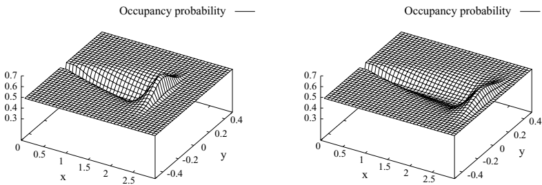
Figure 9.16 Local occupancy probability grids for a single ultrasound measurement of y(k) = 2.0m (left) and y(k) = 2.5m (right).
