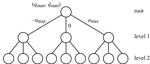
Figure 11.8 The search tree for three controls.
