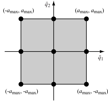
Figure 11.10 The control discretization for n_Q = 2 .
