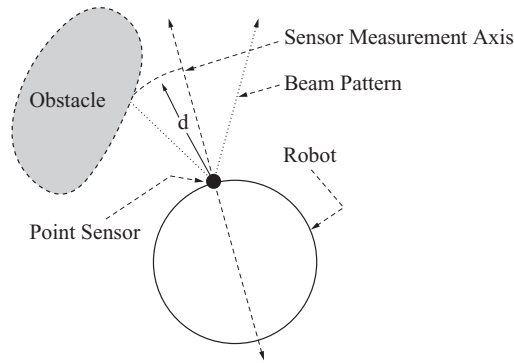
Figure 2.19 Centerline model.
