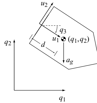
Figure 12.3 The planar body with thrusters (PBWT).
