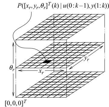
Figure 9.2 Grid-based representation of the state space.
