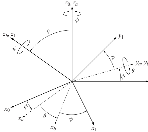
Figure 3.20 Euler angle representation.
