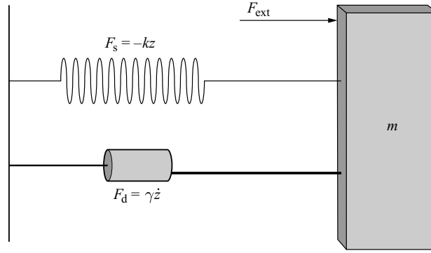
Figure J.1 Mass-spring-damper system.
