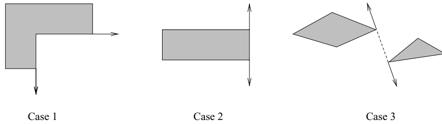
Figure 6.35 The three conservative edge construction cases.
