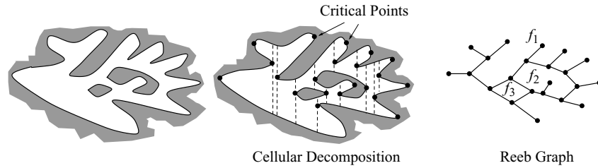
Figure 6.25 In this decomposition example, there are twenty-one critical points (nodes in the graph), N_{cp} = 21 , and two obstacles (faces f_2, f_3 in the graph; f_1 is the outer boundary), N_{ob} = 2 . Using the modified Euler's formula N_{ce} = N_{cp} + N_{ob} - 1 , there must be twenty-two cells (edges in the graph), N_{ce} = 22 .
