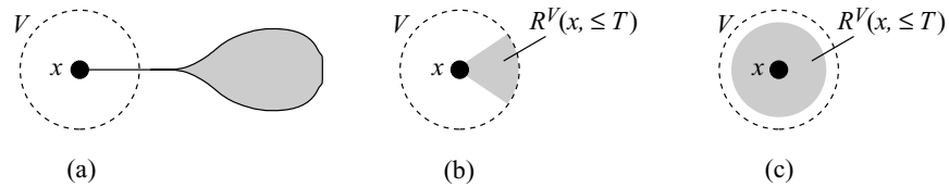
Figure 12.11 Reachable spaces for three systems on \mathbb{R}^2 . (a) This system is accessible from x , but neither small-time locally accessible (STLA) nor small-time locally controllable (STLC). The reachable set is two-dimensional, but not while confined to the neighborhood V . (b) This system is STLA from x , but not STLC. The reachable set without leaving V does not contain a neighborhood of x . (c) This system is STLC from x .
