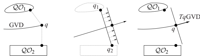
Figure 5.13 The tangent space to the GVD is orthogonal to the line that connects the two closest points on the two closest obstacles.
