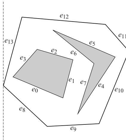
Figure 6.5 L : \emptyset \rightarrow \{e_8, e_{13}\} .
