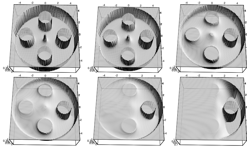
Figure 4.16 Navigation function for a sphere-space with five obstacles for \kappa = 3 , \kappa = 4 , \kappa = 6 , \kappa = 7 , \kappa = 8 , and \kappa = 10 .
