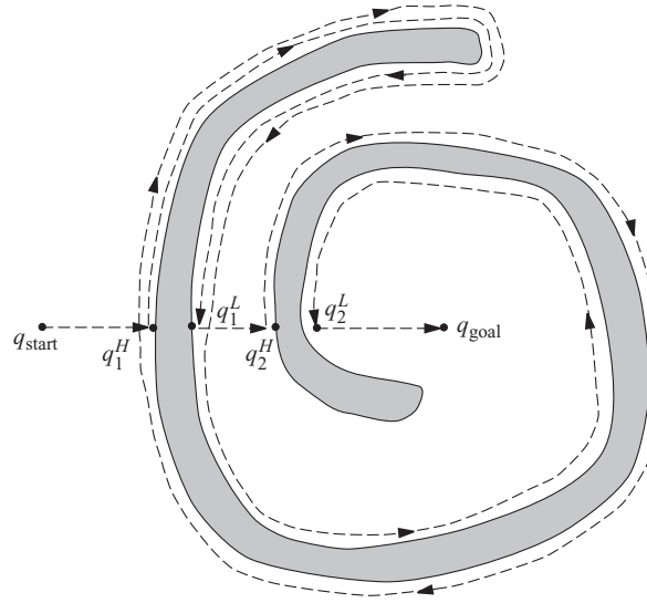
Figure 2.4 Bug2 Algorithm.
