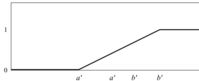
Figure I.1 Cumulative uniform distribution.
