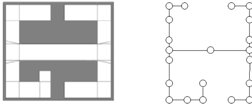
Figure 6.34 Conservative regions and their corresponding adjacency graph.
