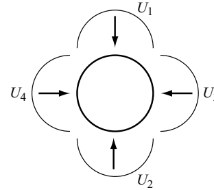
Figure 3.14 Four charts covering the circle S^1 .
