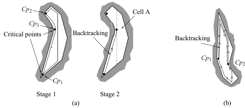
Figure 6.28 (a) The robot starts to cover the space from Cp_1 . Along the first cycle path, it discovers the critical points Cp_1 , Cp_2 , and Cp_3 . The robot moves back to Cp_3 by following the boundary of the obstacle to start to cover cell A. (b) The robot travels back to Cp_2 from Cp_1 by boundary-following and lapping. Therefore, the length of the backtracking path is bounded above by P_{\text{cell}} + D for each cell.
