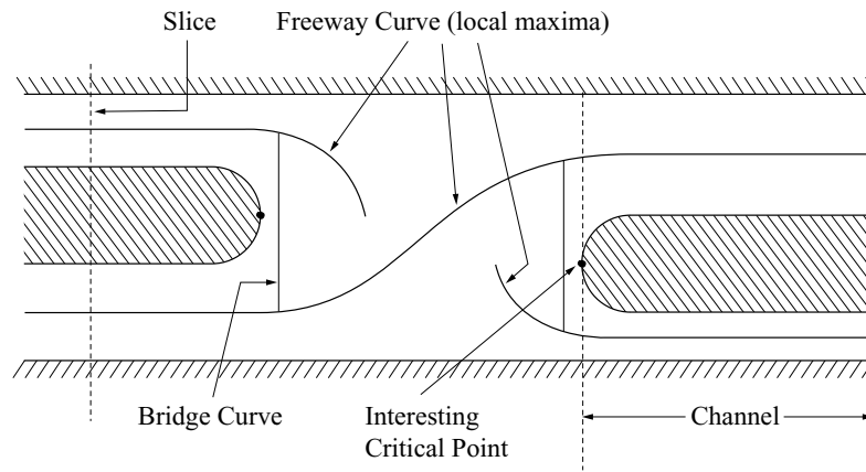
Figure 5.34 Schematic of the OPP planning scheme.
