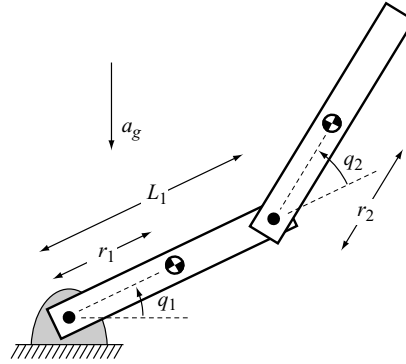
Figure 10.8 The 2R robot arm.
