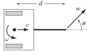
Figure 12.30 A single trailer.
