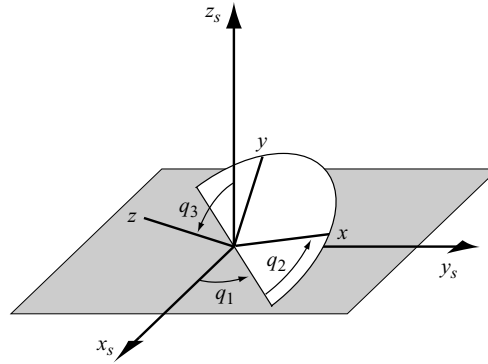
Figure 10.7 Euler angles for a rotating body.
