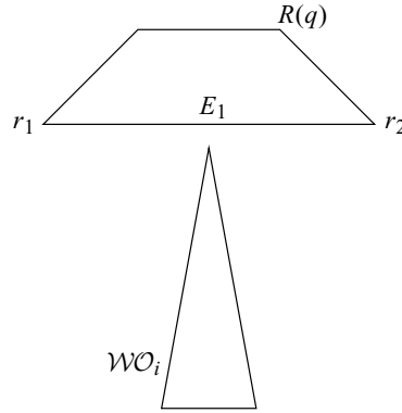
Figure 4.20 The repulsive forces exerted on the robot vertices r_1 and r_2 may not be sufficient to prevent a collision between edge E_1 and the obstacle.
