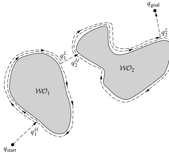
Figure 2.1 The Bug1 algorithm successfully finds the goal.
