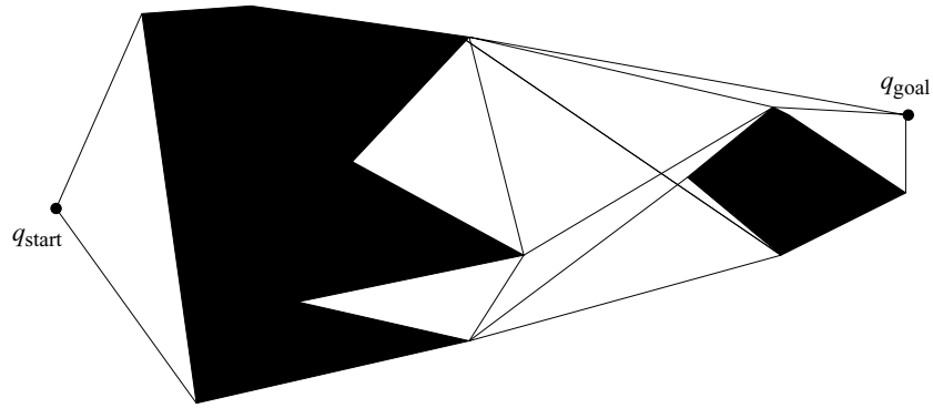
Figure 5.7 Reduced visibility graph with nonconvex obstacles.
