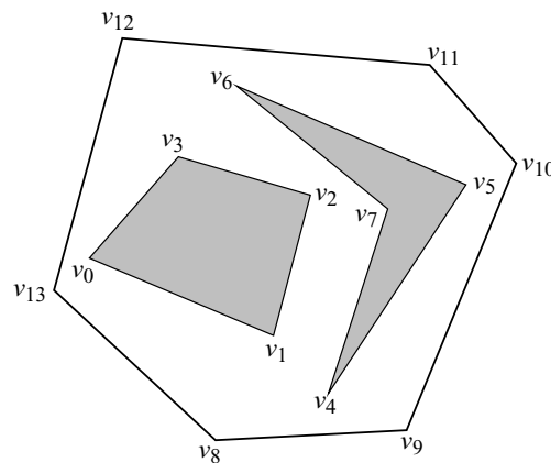
Figure 6.1 Sample polygonal configuration space.
