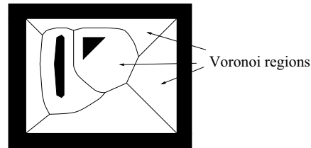
Figure 6.15 GVD of an environment.
