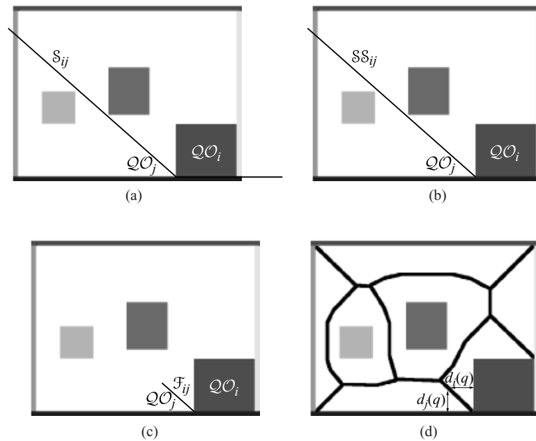
Figure 5.9 (a) The set S_{ij} contains points equidistant to two obstacles QO_i and QO_j . (b) The set SS_{ij} contains equidistant points with distinct gradients; note that there is no SS_{ij} structure to the right of the obstacles. We delay discussion of this structure for a moment. (c) The set F_{ij} has the closest pair of obstacles. (d) The GVD is the union of all such sets.
