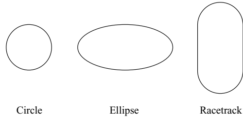
Figure 3.12 A circle, an ellipse, and a racetrack.
