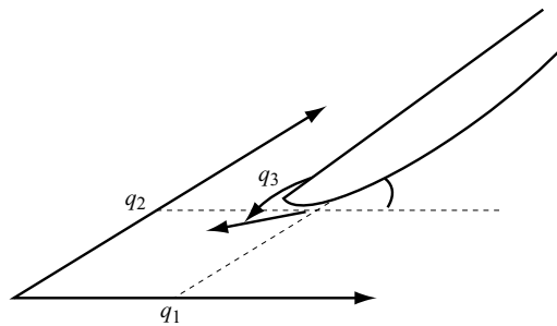
Figure 10.3 A knife-edge on a plane.
