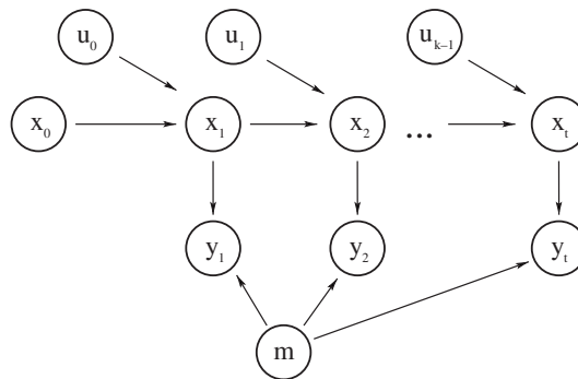
Figure 9.21 Graphical model of incremental probabilistic SLAM.
