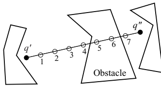
(a) Incremental: The algorithm returns failure after five collision checks.
