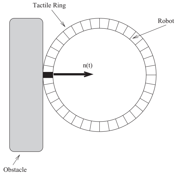
Figure 2.15 A fine-resolution tactile sensor.
