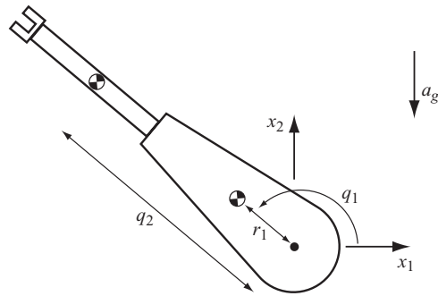
Figure 10.2 The RP manipulator.
