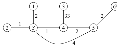
Figure H.14 Dijkstra graph search example.
