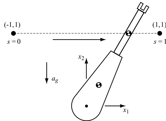
Figure 11.6 The path followed by the RP manipulator.
