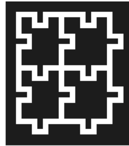
4 holes, 111 edges, 4 pursuers
