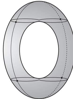
Figure 5.32 Silhouette curves on the torus.
