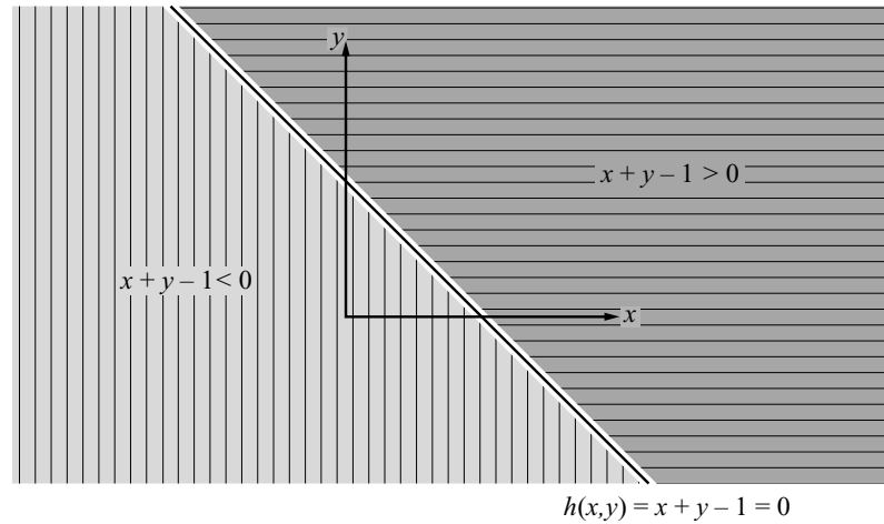
Figure F.1 Half-planes defined by h(x, y) = x + y - 1 .
