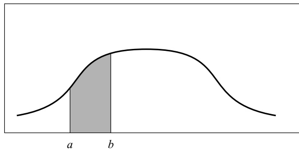
Figure I.2 Probability density function.
