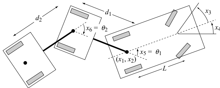
Figure 12.29 A car pulling two trailers.
