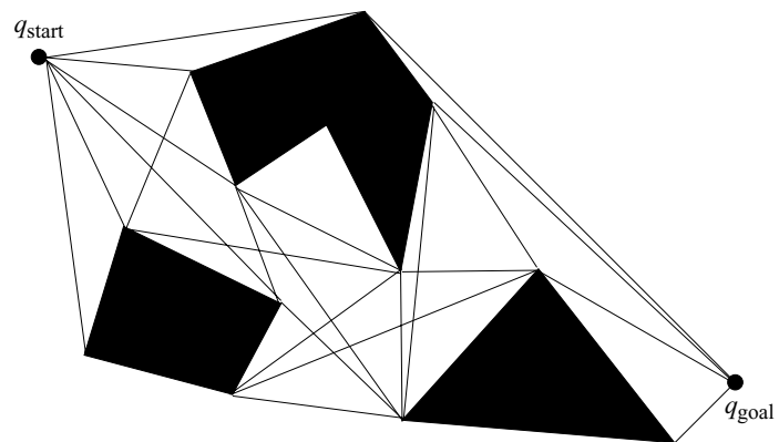
Figure 5.6 Reduced visibility graph.
