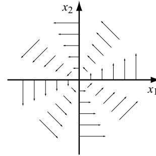
Figure 12.5 The vector field \frac{1}{2}[-x_2, x_1]^T .
