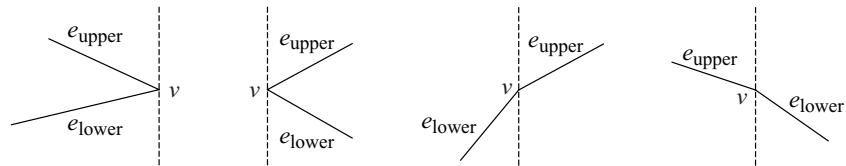
Figure 6.4 The kinds of events.
