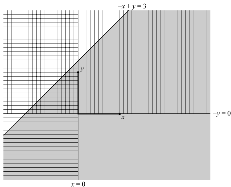
Figure E2 A convex polygonal region constructed from the half planes h_1^- , h_2^- , and h_3^- .
