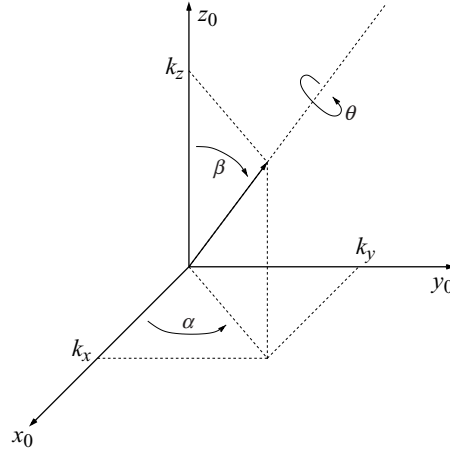
Figure E.2 Rotation about an arbitrary axis.
