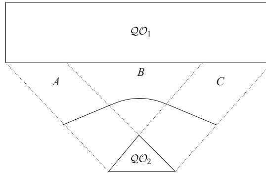
Figure 5.14 GVD edge fragment for two polygonal obstacles.
