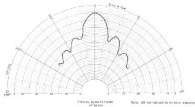
Figure 2.18 Beam pattern for the Polaroid transducer.
