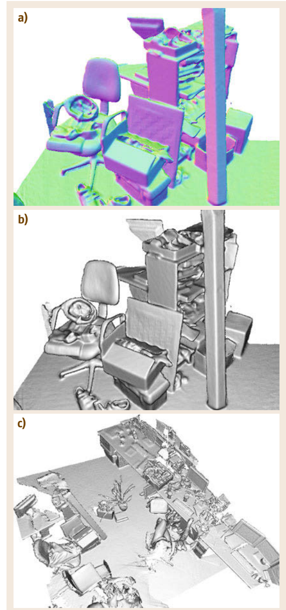
Fig.46.10a–c Results obtained with KinectFusion (after [46.134]). (a) A local scene as a normal map and (b) as a Phong-shaded rendering. The (c) image depicts a larger scene (image courtesy of Richard Newcombe, Imperial College London)
