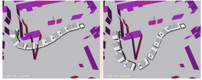
Fig. 47.17 A differentially-driven mobile robot towing a trailer applying the trajectory deformation algorithm to avoid obstacles detected online
