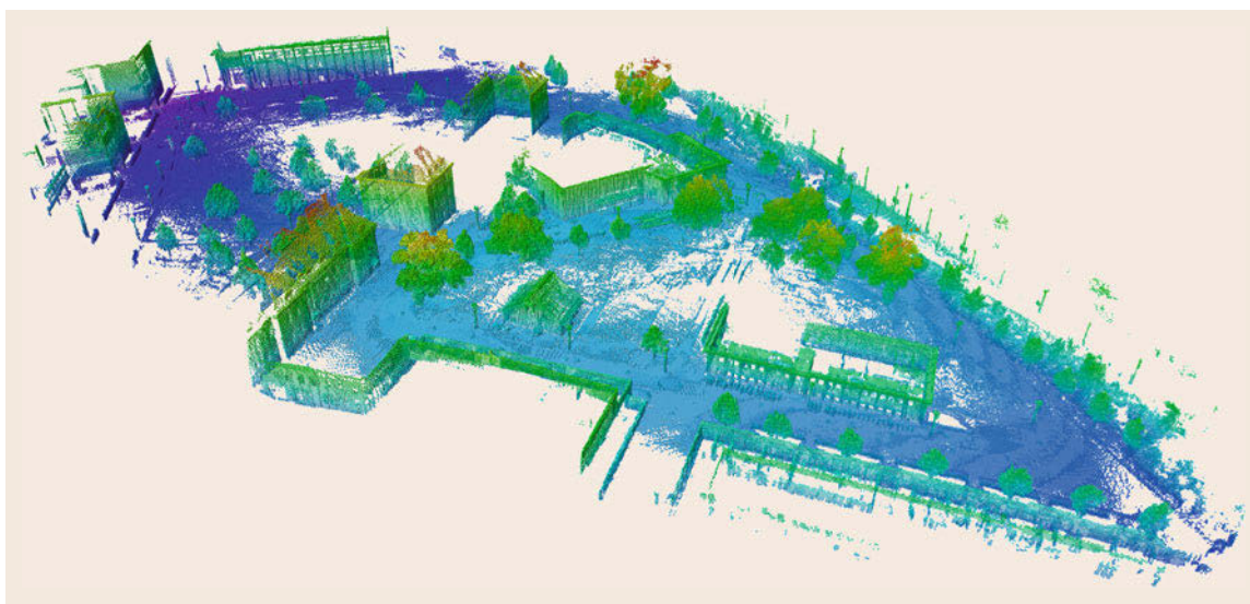
Fig. 45.14 Resulting octree-based representation of an outdoor environment at 0.2m resolution (size of the scene: 292 m × 167 m × 28 m) (after [45.25]). For clarity, only occupied volumes are shown with height visualized by a color (gray scale) coding
