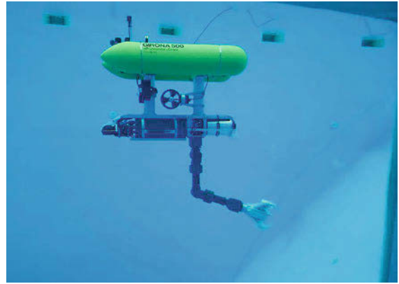
Fig. 51.8 An underwater vehicle–manipulator system (courtesy of FP7-TRIDENT Project Consortium)
