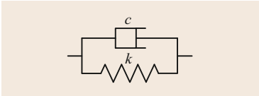
Fig. 37.14 Kelvin–Voigt model
