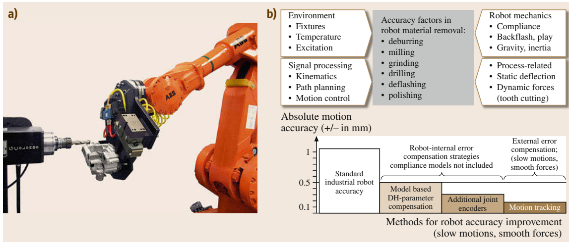
Fig.54.19a-d For small-to-medium-sized parts, a preferred configuration is to have the part grasped and guided by the robot relative to the fixed spindle. (a) The robot's gripper is mounted on a force-torque sensor to measure and limit process forces. For machining the edges of the workpiece (deflashing) the machining software package provides a machine-learning technique for optimising the motions [54.51]. (b) Influences on accuracy in robotic machining and methods for robot accuracy improvement. Still typical machine tool motion accuracies are in the order of \pm 0.01 mm or better (courtesy of ABB, Fraunhofer IPA)
