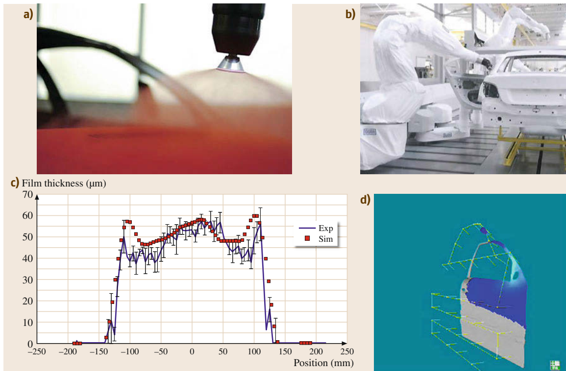
Fig.54.18a–d High-speed rotating atomizer and a multirobot workcell for car body painting. (a) A Dürr EcoBell2 paint gun which atomizes the paint material at the edge of the rotating bell disk by centrifugal forces. All current paint materials such as solvent-based or water-borne paints can be used in car production. (b) Multiple robots work in parallel for optimal throughput and accessibility of the car body. Most of the programming which includes the synchronization of the robots is performed offline, also with respect to optimal coverage of the painted surface. (c) Simulation of the painting process is critical for achieving highest yields (e.g., minimal overspray, uniform paint deposition, etc.) (d) Results from simulations for optimized program generation are shown (courtesy of Dürr, Fraunhofer IPA, Stuttgart)
