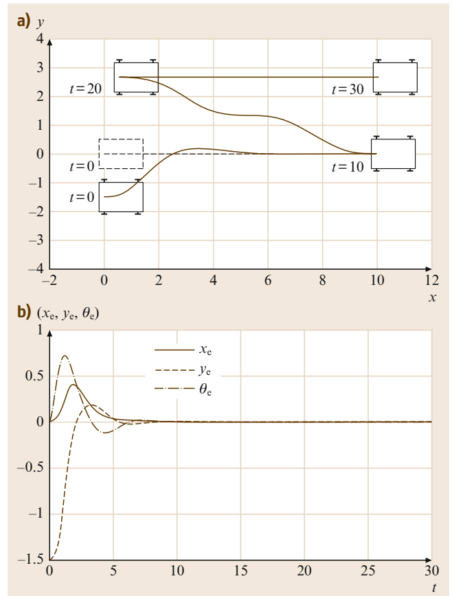
Fig.49.8a,b Tracking of a reference vehicle. (a) Cartesian motion; (b) error coordinates versus time
