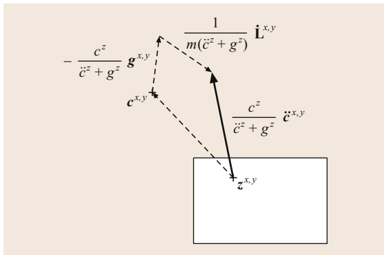
Fig. 48.3 The horizontal acceleration \ddot{c}^{x,y} of the COM of the robot is the sum of a force pushing the COM c^{x,y} away from the CoP z^{x,y} the effect of gravity -g^{x,y} and variations \dot{\mathbf{L}}^{x,y} of the angular momentum
