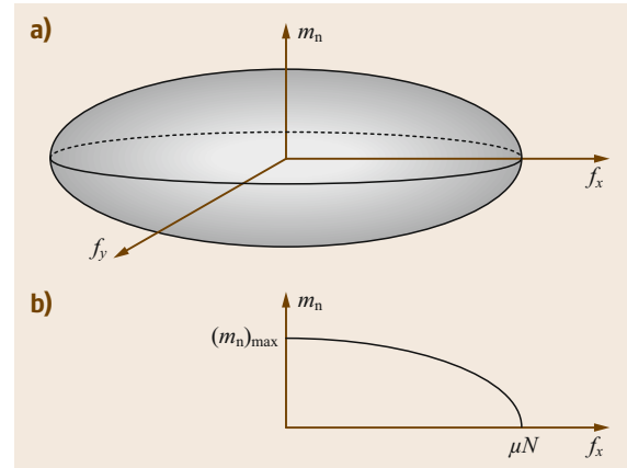
Fig.37.19a,b Friction limit surface for soft fingers: (a) a 3-D ellipsoid representing the limit surface, and (b) a section of the ellipsoidal limit surface showing the coupled relationship between the force and moment, as those obtained in Fig. 37.18
