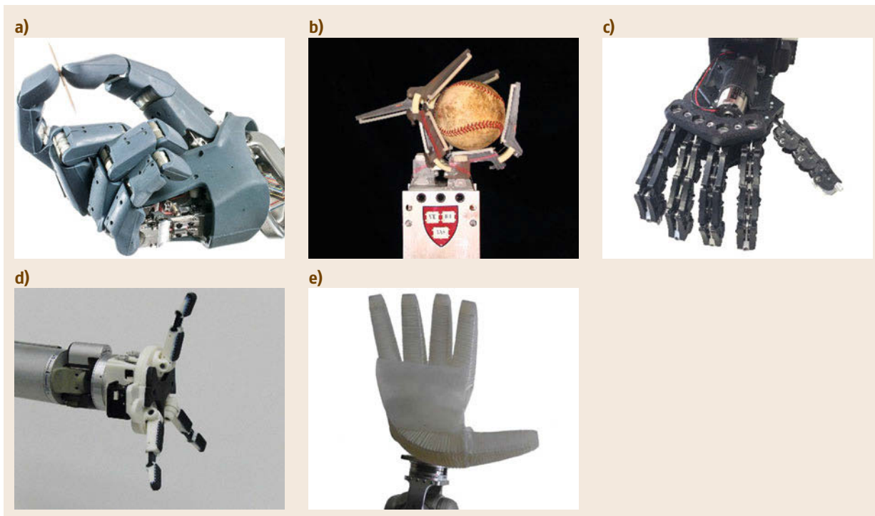
Fig.40.2a–e Various hand designs leveraging compliance to improve performance. (a) Awiwi hand (DLR), (b) SDM hand (Harvard), (c) Pisa-IIT hand, (d) i-HY hand (iRobot, Harvard, Yale), (e) RBO hand z (TU Berlin)
