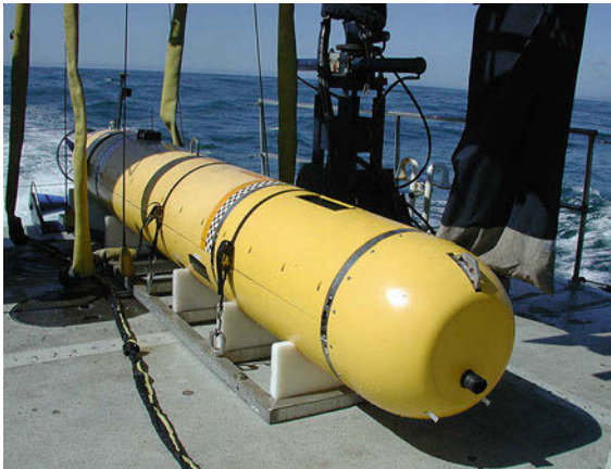
Fig. 51.3 The AUV Dorado (courtesy of Monterey Bay Aquarium Research Institute [51.22])
