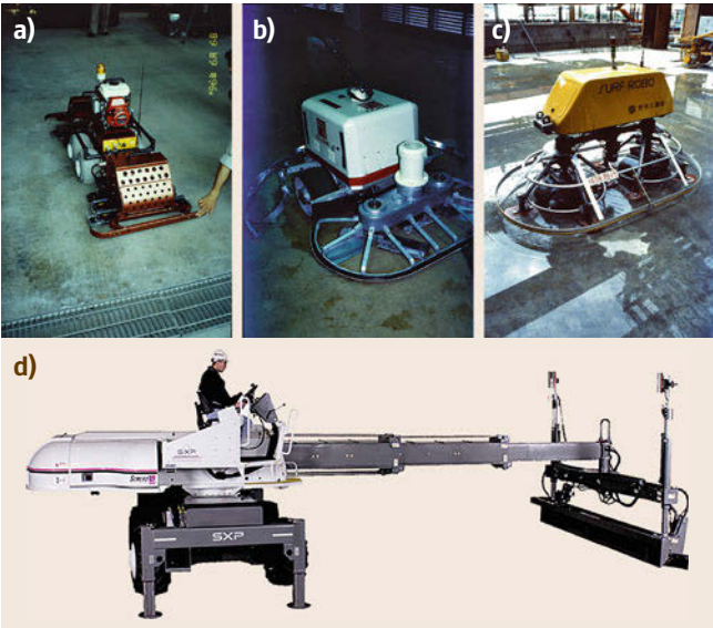
Fig. 57.19 (a) Hazama robot; (b) Kajima Kote King robot; (c) Tak-enaka Surf Robo; (d) auto-leveling concrete screed machine (courtesy Somero Enterprises, Inc.)
