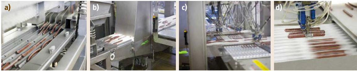
Fig. 54.9a–d Units of sausage are cut from strings, then placed into the thermo-formed cavities before applying lidding. The coordination of the robots and the optimization of the picking frequency require a selection of the best path for each robot. Missed sausages are fed back on the conveyor for another try. The shown 4-DOF parallel robot reaches cycle times of 1–3 Hz and can move payloads of up to 8 kg (courtesy of robomotion, Germany)
