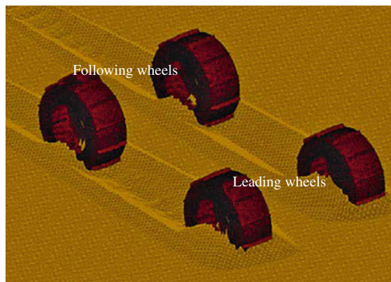
Fig. 50.1 Dynamics of a plastically deformable surface in consideration with the multipass effect of wheels (after [50.4])
