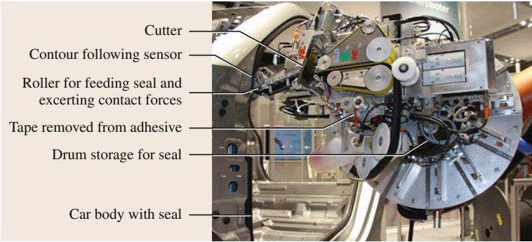
Fig. 54.15 A robot-guided tool for handling and processing limb material, in this case a self-adhesive seal for car bodies
