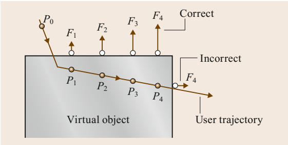
Fig. 42.8 Illustration of subtle aspects of haptic rendering of contact force. The operator fingertip trajectory enters object surface moving down and to the right. Haptic interaction points (HIP) are shown at times 1–4 (solid circles, P_0 – P_4 ). Intermediate haptic interaction points (IHIP) are shown when the HIP is inside the object (open circles). At position P_4 , the algorithm must not render force based on the closest surface point or the operator will be ejected from the side of the object (feeling unnatural force tangential to the top surface)
