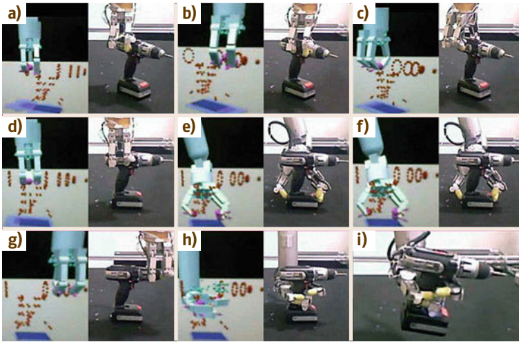
Fig.41.8a-i An example sequence of grasping a powerdrill based on a depth-2 search through belief space. The right-hand side of each pair of images shows the grasp just executed, while the left-hand side shows the resulting belief. The dark blue flat rectangle and the red point-outline of the powerdrill show the most likely state, while the light blue rectangles show states that are 1 standard deviation away from the mean in each dimension ( x, y, \theta ). Panels (a–c) and (e–g) show information-gathering grasps being used to localize the drill, panel (d) shows the robot reorienting the drill to bring the desired grasp within reach, and panels (h) and (i) show the robot using the desired final grasp on the drill, lifting, and pulling the trigger successfully (after [41.42])
