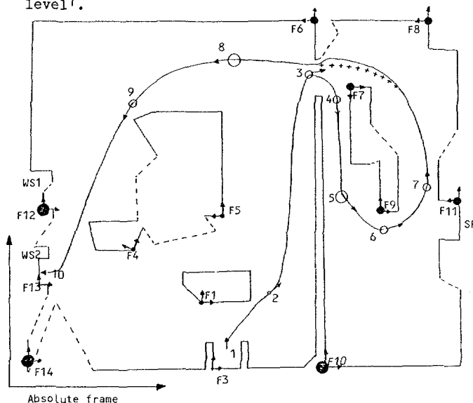
FIGURE 6: The final model with the associated errors on robot and frame position (the orientations errors are not represented)
