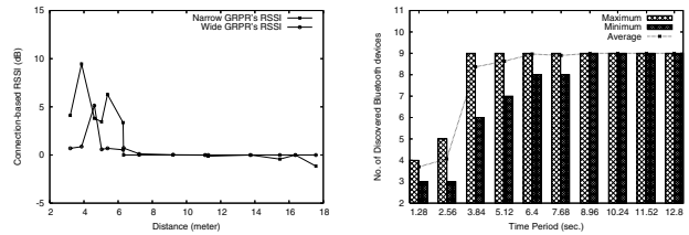
(a) Connection-based RSSI for 2 different Bluetooth adapters (b) Max, min and avg no. of discovered Bluetooth adapters with different inquiry periods (Total no. of devices = 9).
