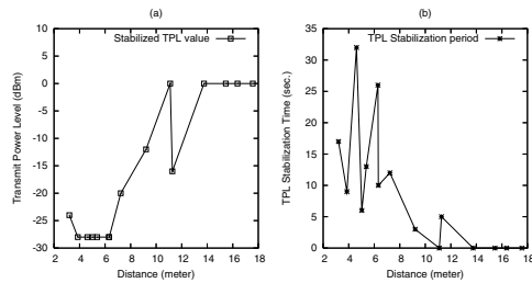
Figure 4: Stabilized TPLs &amp; time periods to attain them.
