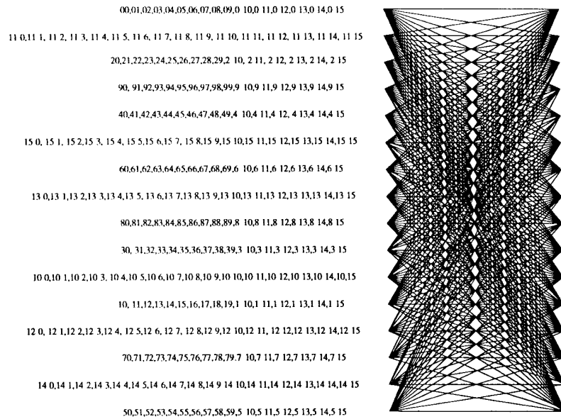
Fig. 19. 2-space-time 16-QAM code, 16 states, 4 b/s/Hz.
