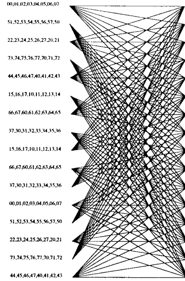
Fig. 8. 2-space-time code, 8-PSK, 16 states, 3 b/s/Hz.
