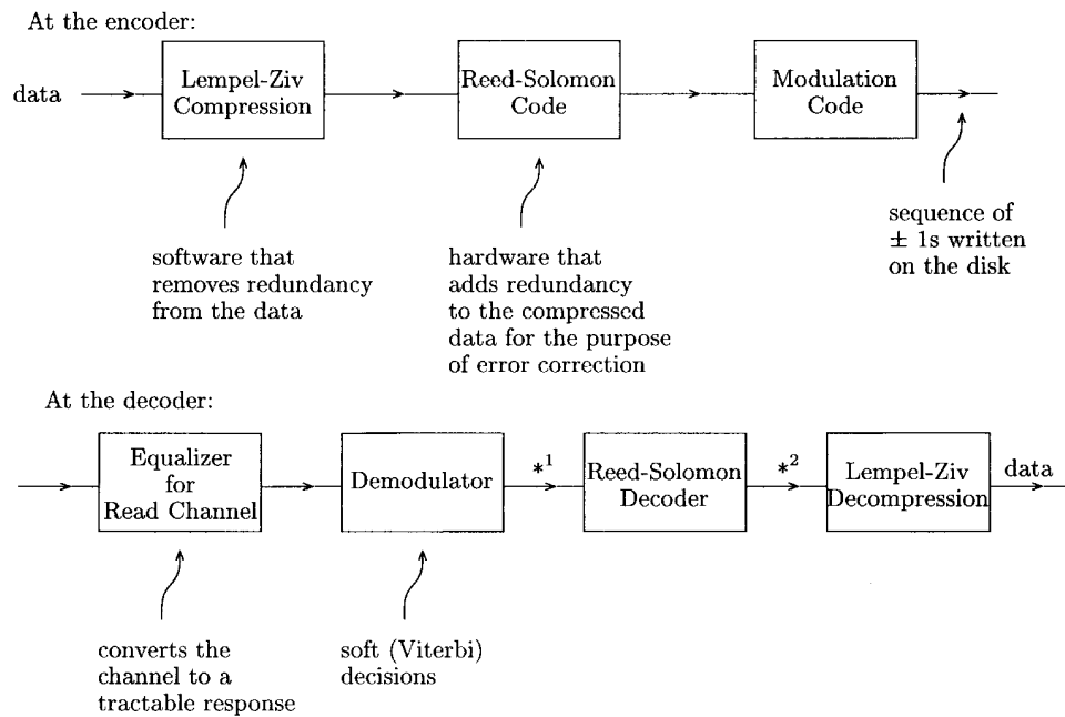
Fig. 9. Concatenation of an inner modulation code with an outer Reed–Solomon code. At *^1 the demodulator provides a maximum-likelihood estimate of the \pm valued sequence written on the disk, and the bit-error probability might be between 10^{-6} and 10^{-10} depending on the aggressiveness of the modulation strategy. At *^2 the bit-error probability needs to be 10^{-18} , that is, essentially error-free.
